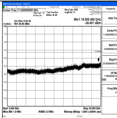
Band2_20MHz_QPSK_19100_1RB#0_3000~20000_3000~20000
