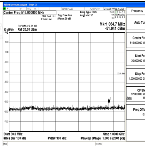
Band2_20MHz_QPSK_19100_1RB#0_30~1000_30~1000
