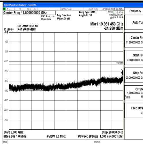
Band2_20MHz_16QAM_19100_1RB#0_3000~20000_3000~20000
