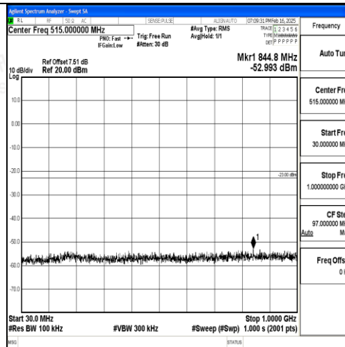
Band2_20MHz_16QAM_18700_1RB#0_30~1000_30~1000
