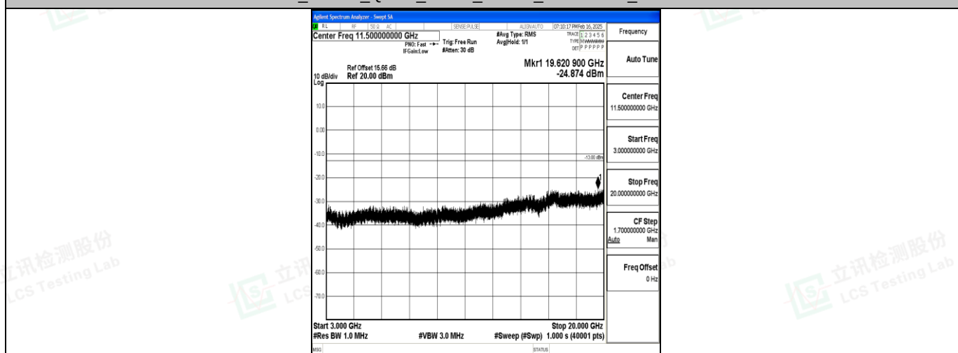
Band2_20MHz_QPSK_18900_1RB#0_3000~20000_3000~20000
