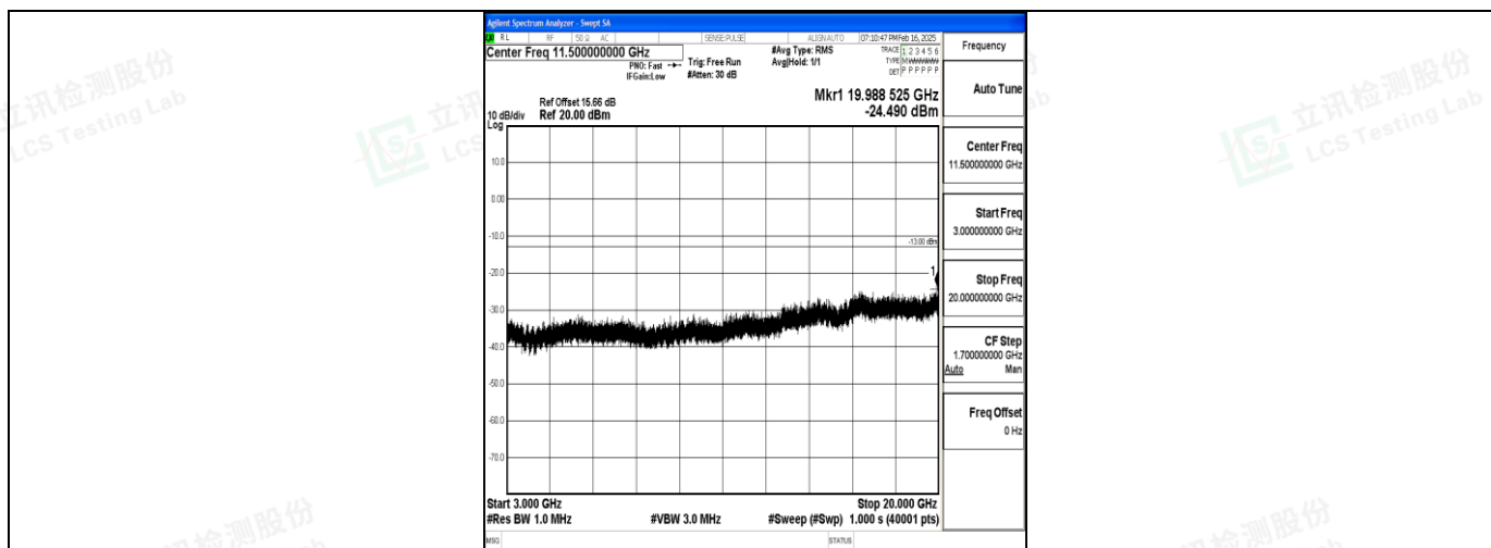
Band2_20MHz_16QAM_18900_1RB#0_3000~20000_3000~20000
