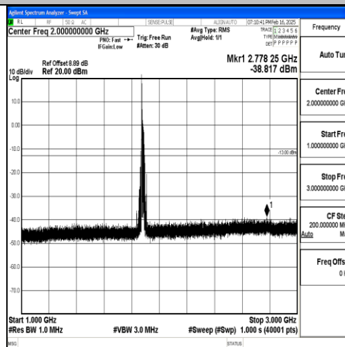
Band2_20MHz_16QAM_18900_1RB#0_1000~3000_1000~3000
