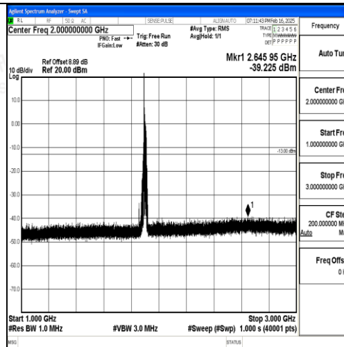
Band2_20MHz_16QAM_19100_1RB#0_1000~3000_1000~3000
