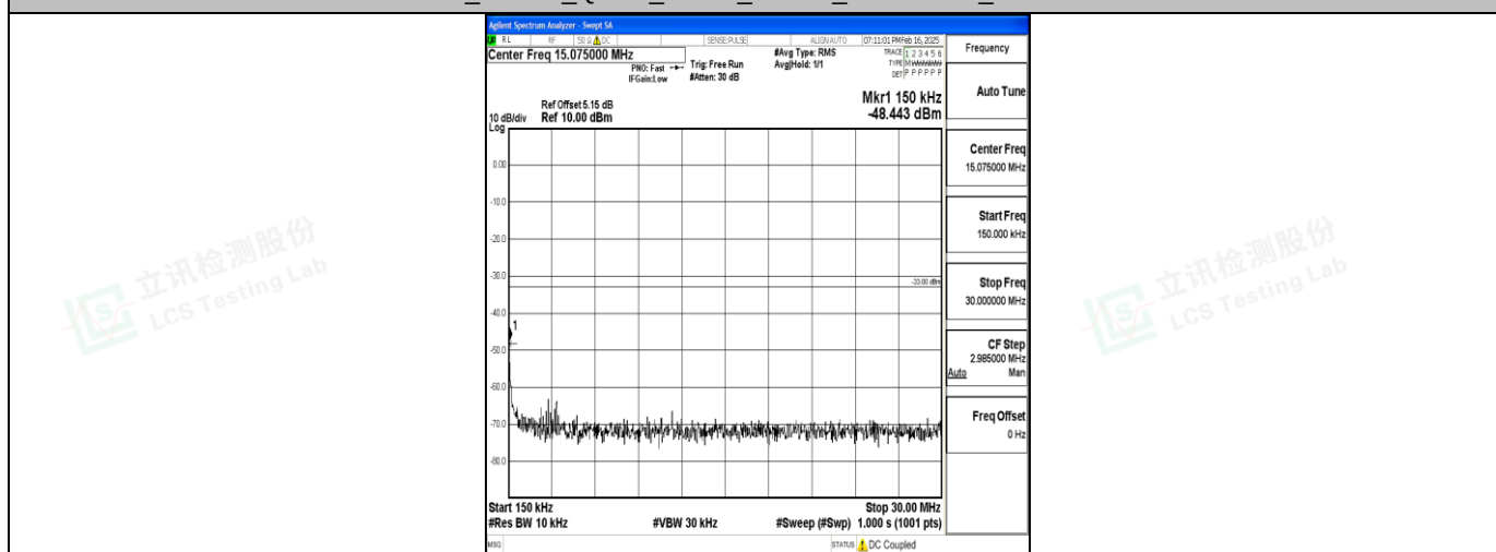
Band2_20MHz_QPSK_19100_1RB#0_0.15~30_0.15~30
