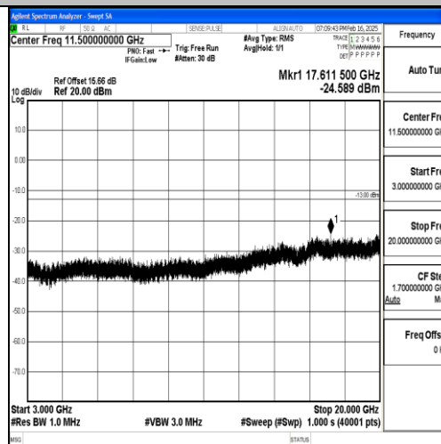
Band2_20MHz_16QAM_18700_1RB#0_3000~20000_3000~20000
