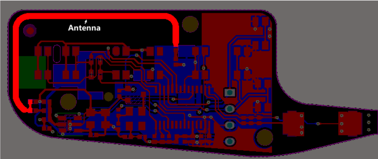
Antenna Size:15mm*26mm*1mm
