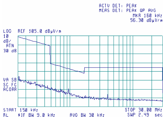
Plot 7.15.12 Radiated emission measurements from 0.15 to 30 MHz at the 5.805GHz carrier frequency
