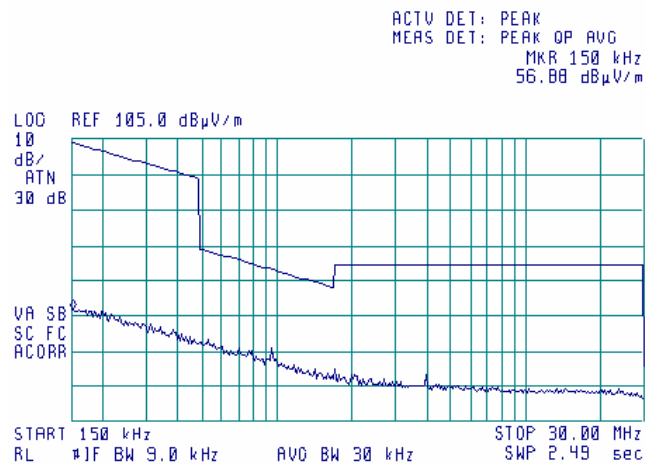
Plot 7.14.10 Radiated emission measurements from 0.15 to 30 MHz at the 5.745GHz carrier frequency
