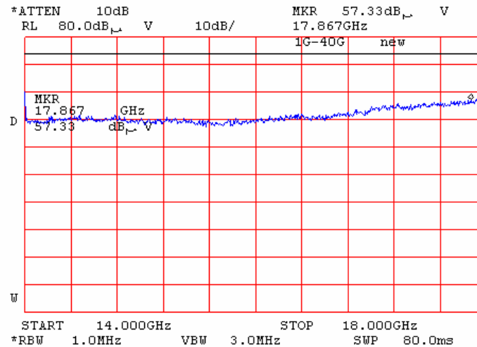
Plot 7.15.34 Radiated emission measurements from 14 to 18 GHz at the 5.18GHz carrier frequency
