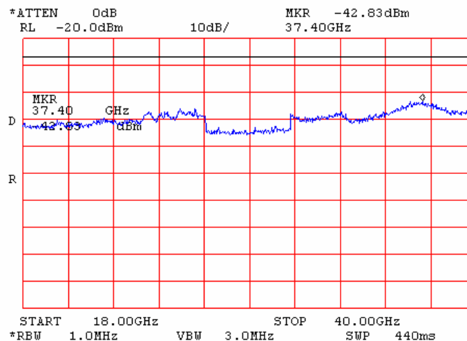
Plot 7.17.34 Conducted emission measurements from 18 to 40 GHz at the 5.745GHz carrier frequency
