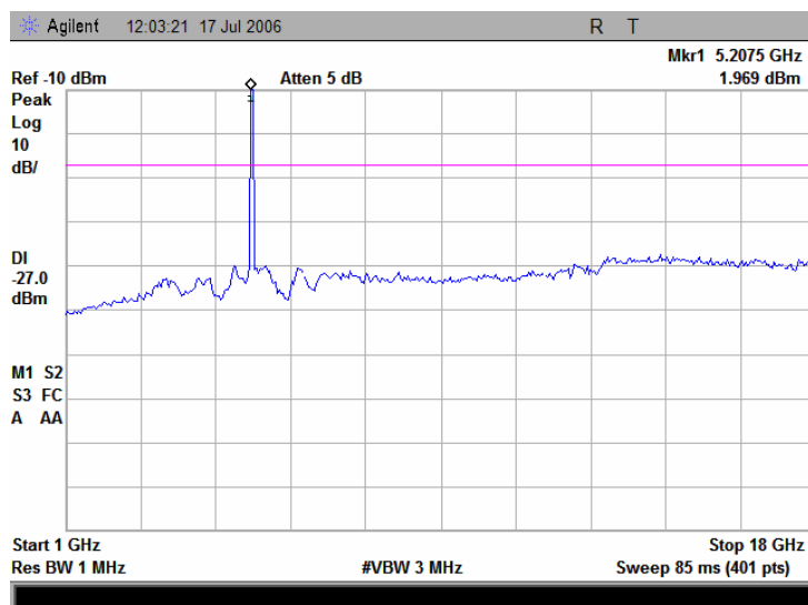
Plot 7.16.19 Conducted emission measurements from 1.0 to 18 GHz at the 5.18 GHz carrier frequency
