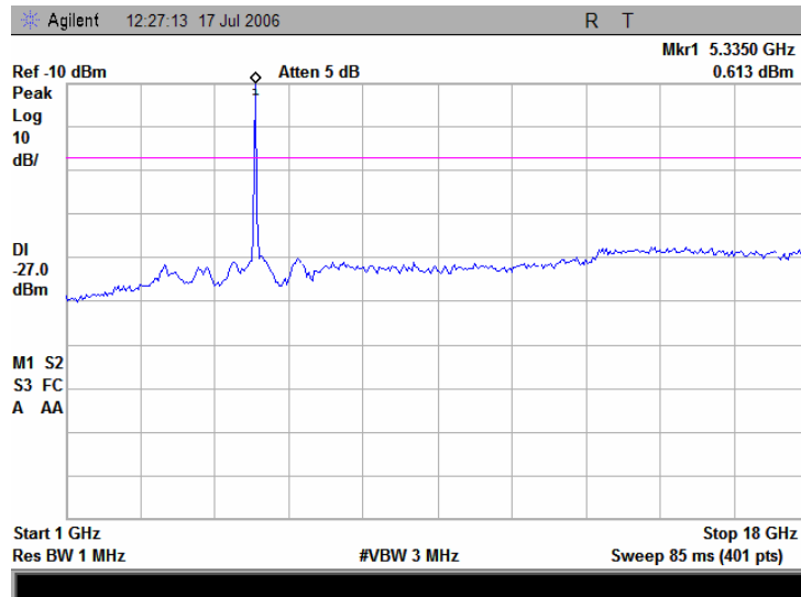
Plot 7.16.25 Conducted emission measurements from 1.0 to 18 GHz at the 5.32 GHz carrier frequency
