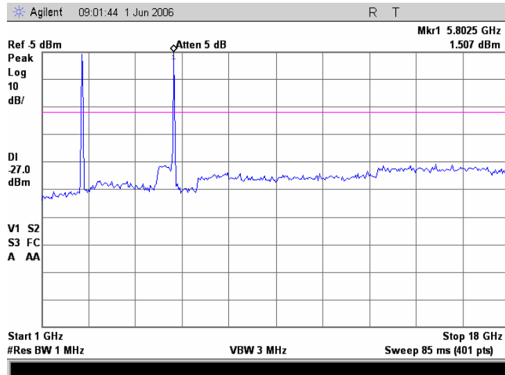
Plot 7.17.35 Conducted emission measurements from 1.0 to 18 GHz at the 5.785 GHz carrier frequency
