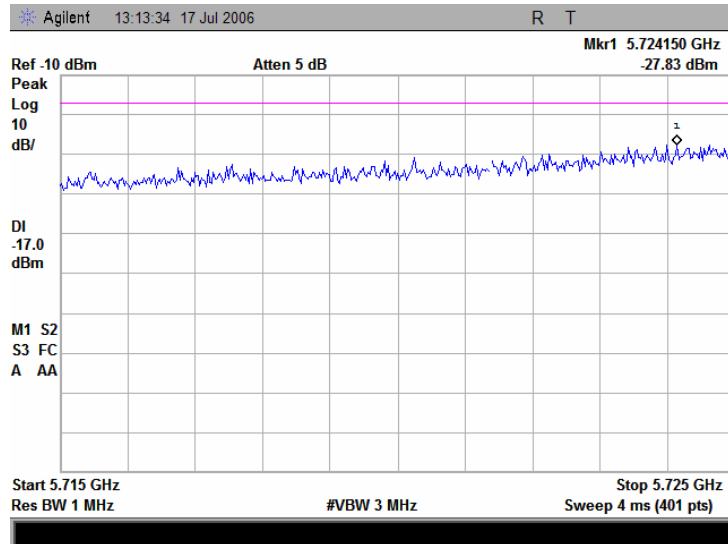
Plot 7.16.31 Conducted emission measurements from 5.715 to 5.725 GHz at the 5.745 GHz carrier frequency
