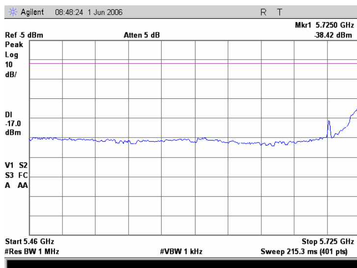
Plot 7.17.32 Conducted emission measurements from 5.46 to 5.725 GHz at the 5.745 GHz carrier frequency
