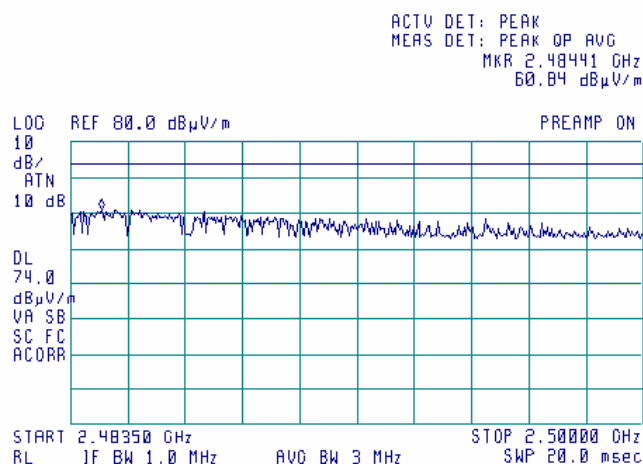
Plot 7.15.58 Radiated emission measurements from 2.4835 to 2.5GHz at the 5.32 GHz carrier frequency
