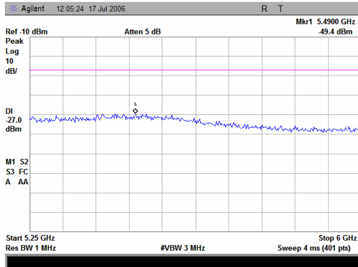
Plot 7.16.21 Conducted emission measurements from 5.25 to 6.0 GHz at the 5.18 GHz carrier frequency
