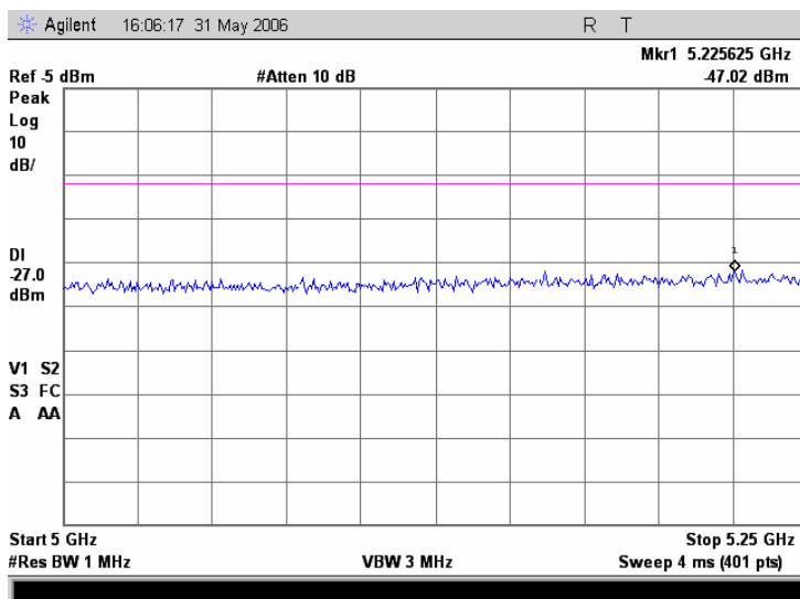
Plot 7.17.26 Conducted emission measurements from 5.0 to 5.25 GHz at the 5.32 GHz carrier frequency
