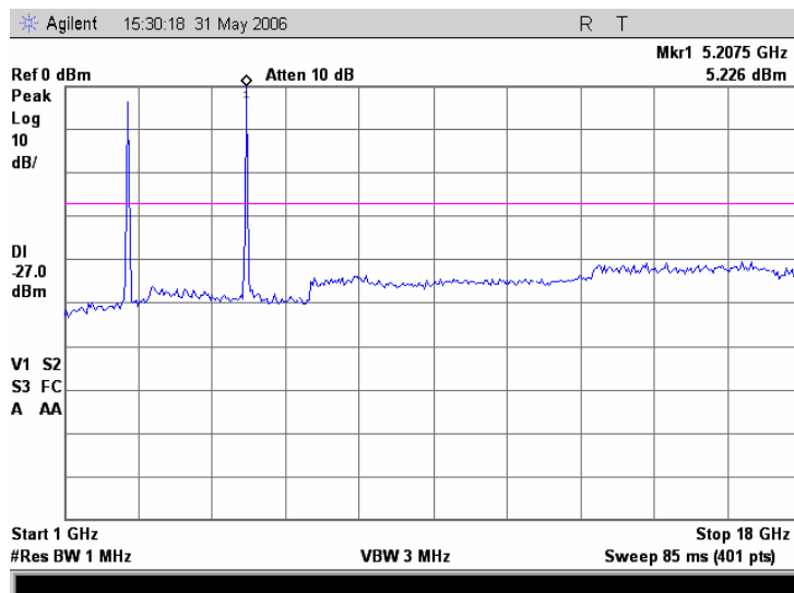
Plot 7.17.19 Conducted emission measurements from 1.0 to 18 GHz at the 5.18 GHz carrier frequency
