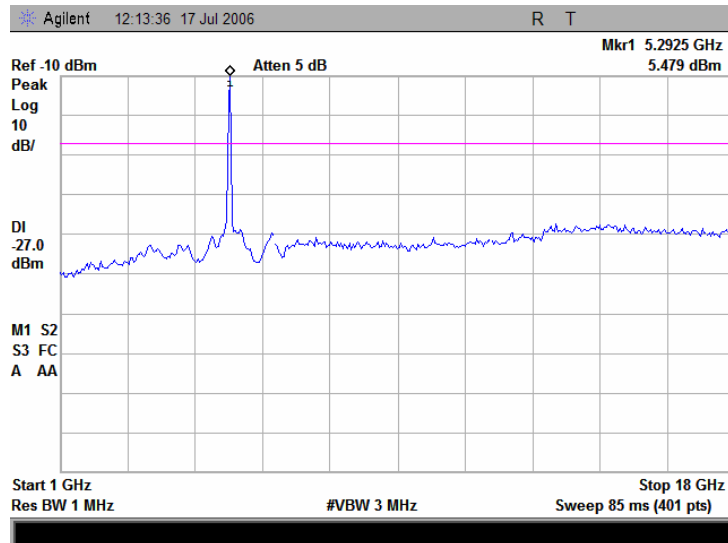
Plot 7.16.23 Conducted emission measurements from 1.0 to 18 GHz at the 5.26 GHz carrier frequency
