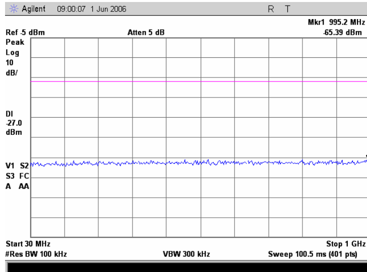
Plot 7.17.18 Conducted emission measurements from 30 to 1000 MHz at the 5.805GHz carrier frequency
