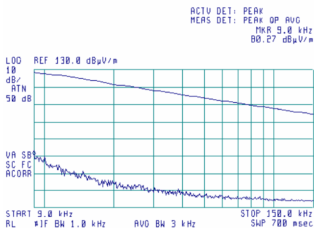
Plot 7.14.6 Radiated emission measurements from 9 to 150 kHz at the 5.805GHz carrier frequency
