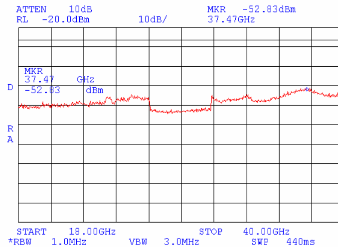
Plot 7.16.37 Conducted emission measurements from 18 to 40 GHz at the 5.785GHz carrier frequency
