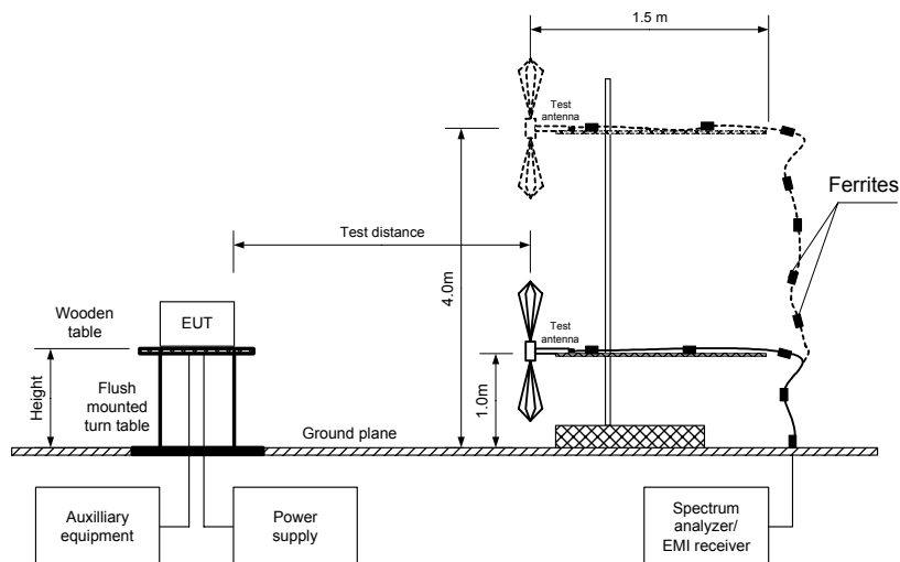
Figure 7.14.2 Setup for spurious emission field strength measurements above 30 MHz
