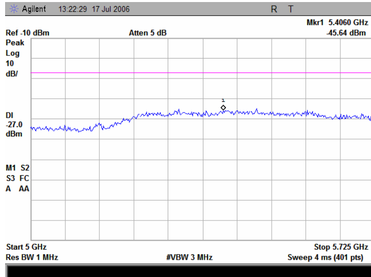
Plot 7.16.39 Conducted emission measurements from 5.0 to 5.725 GHz at the 5.805 GHz carrier frequency
