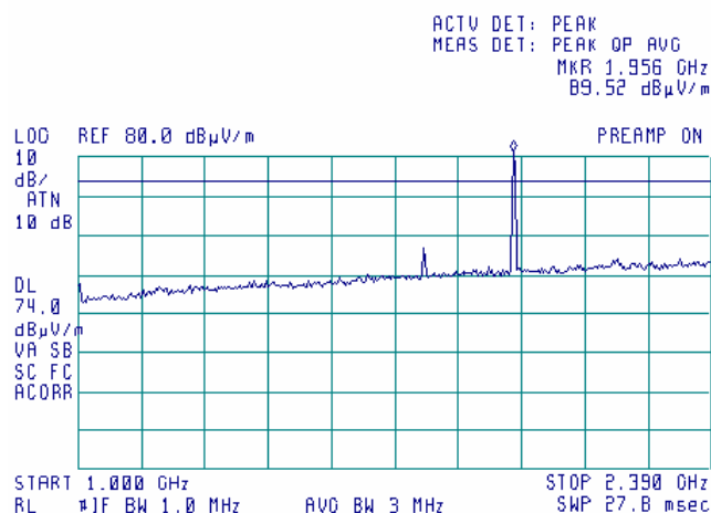
Plot 7.15.112 Radiated emission measurements from 1.0 to 2.39 GHz at the 5.805 GHz carrier frequency
