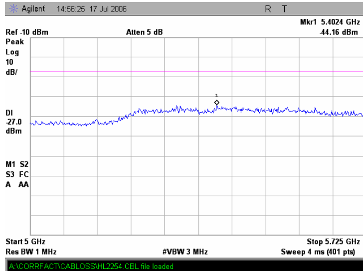
Plot 7.16.35 Conducted emission measurements from 5.0 to 5.725 GHz at the 5.785 GHz carrier frequency
