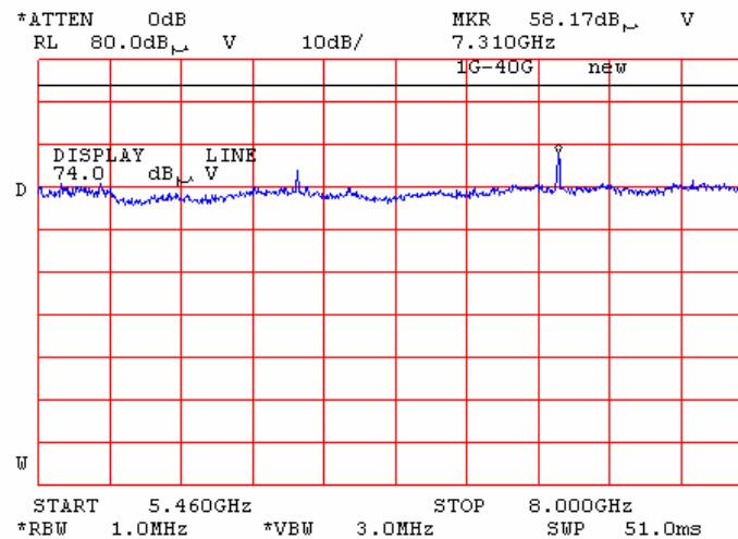
Plot 7.14.66 Radiated emission measurements from 5.46 to 8.0 GHz at the 5.32GHz carrier frequency
