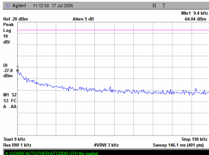
Plot 7.16.4 Conducted emission measurements from 9 to 150 kHz at the 5.745GHz carrier frequency
