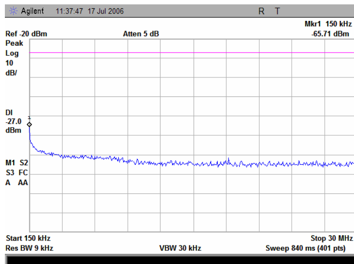
Plot 7.16.8 Conducted emission measurements from 0.15 to 30 MHz at the 5.26GHz carrier frequency
