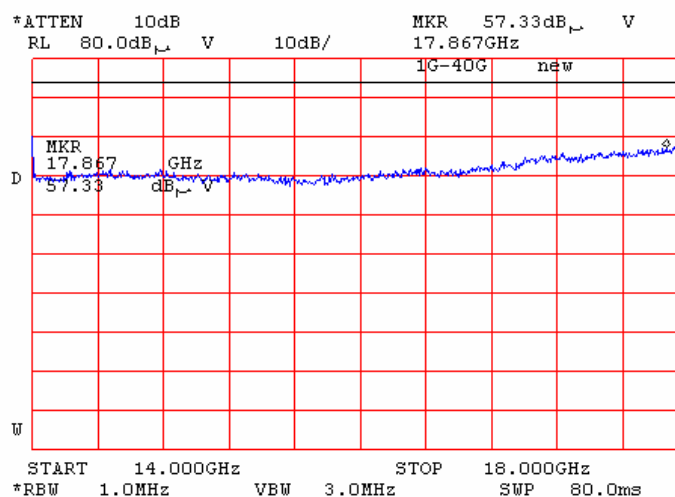
Plot 7.14.34 Radiated emission measurements from 14 to 18 GHz at the 5.18GHz carrier frequency
