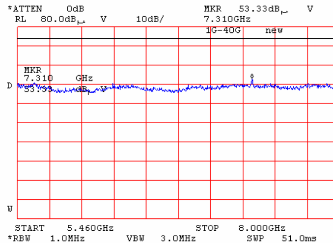
Plot 7.15.30 Radiated emission measurements from 5.46 to 8.0 GHz at the 5.18 GHz carrier frequency
