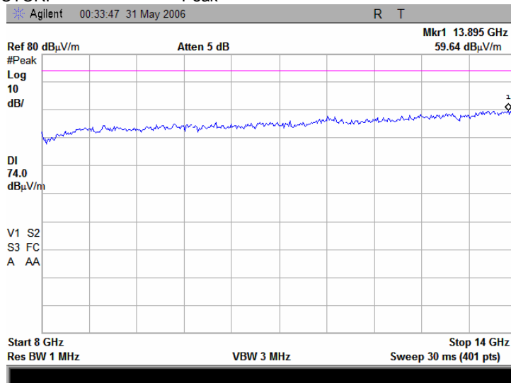
Plot 7.14.68 Radiated emission measurements from 8 to 14 GHz at the 5.32 GHz carrier frequency
