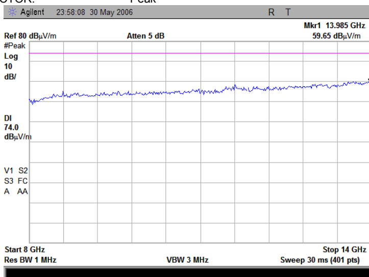
Plot 7.14.124 Radiated emission measurements from 8 to 14 GHz at the 5.805GHz carrier frequency
