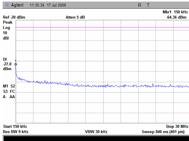
Plot 7.16.10 Conducted emission measurements from 0.15 to 30 MHz at the 5.745GHz carrier frequency
