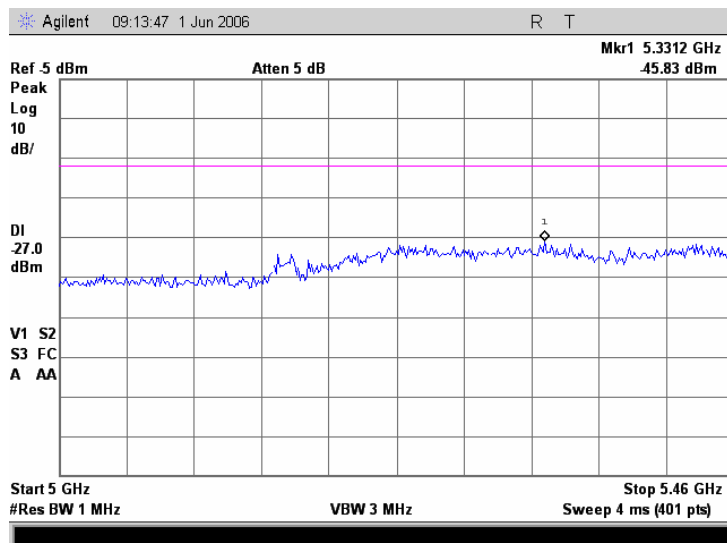
Plot 7.17.41 Conducted emission measurements from 5.0 to 5.46 GHz at the 5.805 GHz carrier frequency
