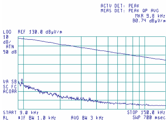
Plot 7.15.6 Radiated emission measurements from 9 to 150 kHz at the 5.805GHz carrier frequency
