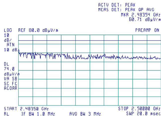
Plot 7.14.114 Radiated emission measurements from 2.4835 to 2.5GHz at the 5.805 GHz carrier frequency
