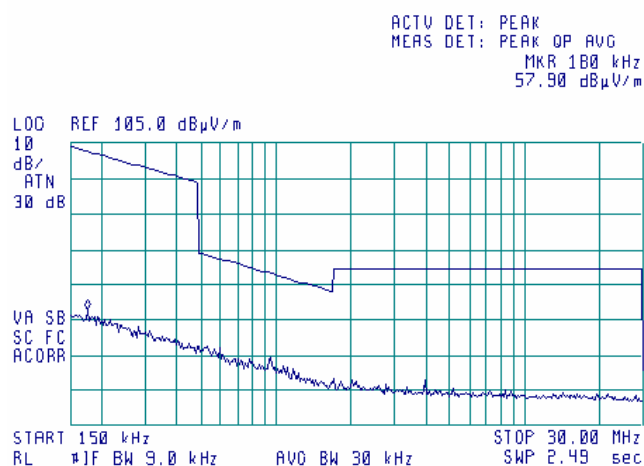
Plot 7.14.12 Radiated emission measurements from 0.15 to 30 MHz at the 5.805GHz carrier frequency
