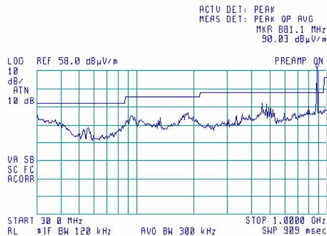
Plot 7.15.14 Radiated emission measurements from 30 to 1000 MHz at the 5.26GHz carrier frequency
