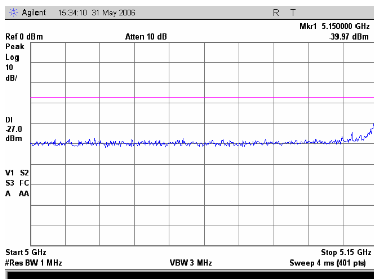
Plot 7.17.20 Conducted emission measurements from 5.0 to 5.15 GHz at the 5.18 GHz carrier frequency
