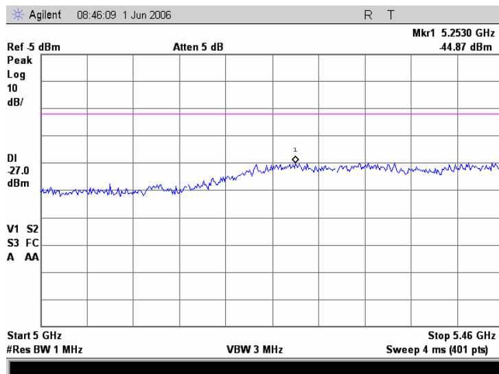
Plot 7.17.31 Conducted emission measurements from 5.0 to 5.46 GHz at the 5.745 GHz carrier frequency
