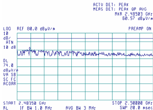
Plot 7.15.114 Radiated emission measurements from 2.4835 to 2.5GHz at the 5.805 GHz carrier frequency
