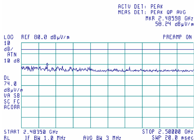
Plot 7.14.22 Radiated emission measurements from 2.4835 to 2.5 GHz at the 5.18GHz carrier frequency
