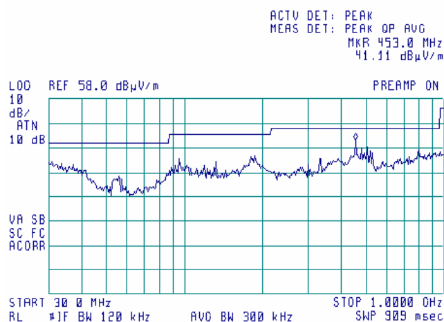
Plot 7.14.14 Radiated emission measurements from 30 to 1000 MHz at the 5.26GHz carrier frequency
