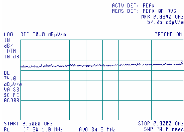
Plot 7.15.116 Radiated emission measurements from 2.5 to 2.9 GHz at the 5.805 GHz carrier frequency
