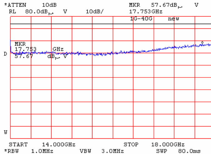
Plot 7.14.88 Radiated emission measurements from 14 to 18 GHz at the 5.745GHz carrier frequency
