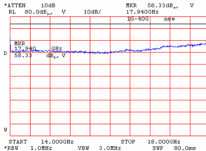
Plot 7.14.126 Radiated emission measurements from 14 to 18 GHz at the 5.805GHz carrier frequency
