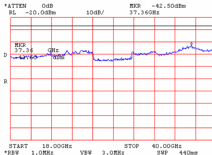
Plot 7.17.24 Conducted emission measurements from 18 to 40 GHz at the 5.26 GHz carrier frequency
