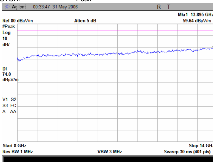
Plot 7.15.68 Radiated emission measurements from 8 to 14 GHz at the 5.32 GHz carrier frequency
