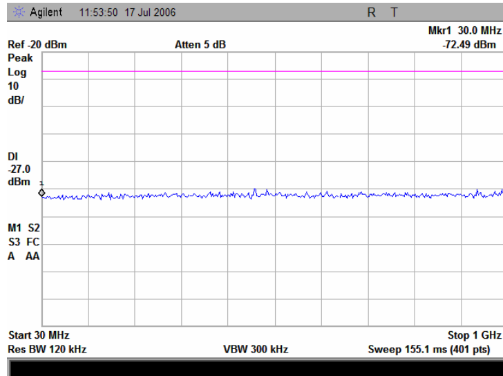
Plot 7.16.18 Conducted emission measurements from 30 to 1000 MHz at the 5.805GHz carrier frequency
