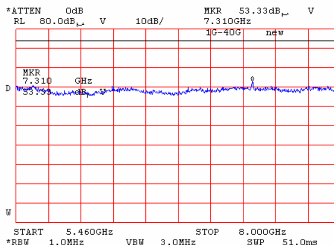
Plot 7.14.30 Radiated emission measurements from 5.46 to 8.0 GHz at the 5.18GHz carrier frequency
