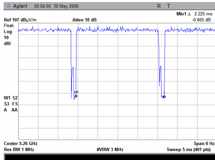
Plot 7.14.147 Transmission burst period
