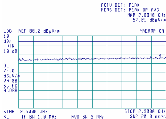
Plot 7.15.24 Radiated emission measurements from 2.5 to 2.9 GHz at the 5.18GHz carrier frequency
