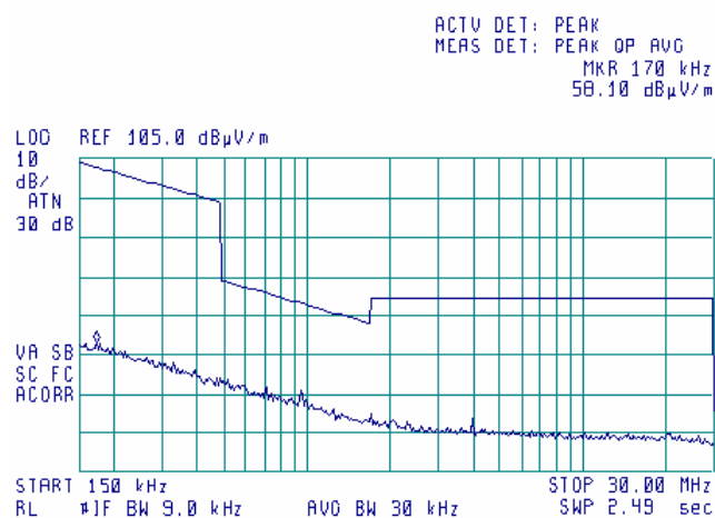
Plot 7.15.8 Radiated emission measurements from 0.15 to 30 MHz at the 5.26GHz carrier frequency
