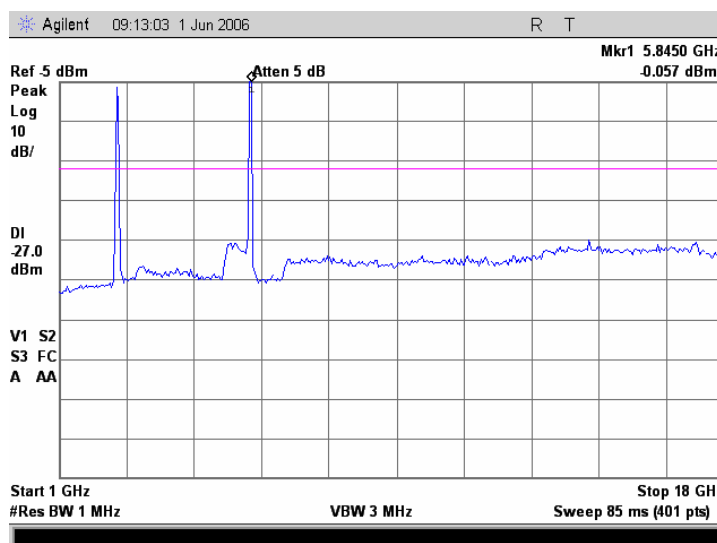
Plot 7.17.40 Conducted emission measurements from 1.0 to 18 GHz at the 5.805 GHz carrier frequency
