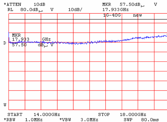
Plot 7.15.70 Radiated emission measurements from 14 to 18 GHz at the 5.32GHz carrier frequency
