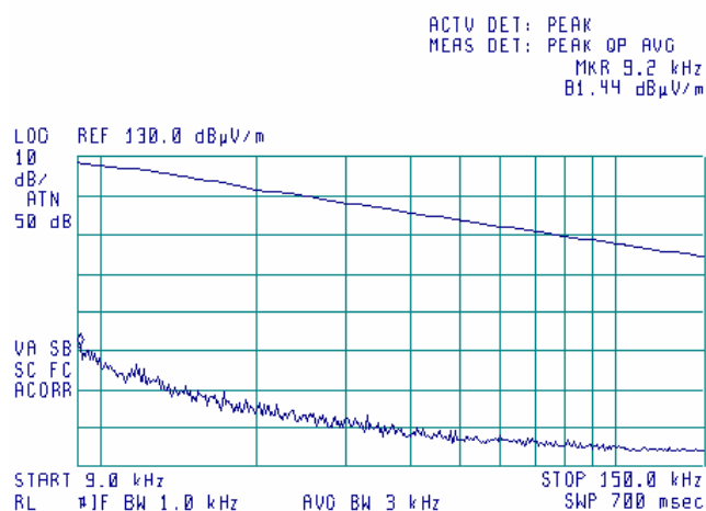
Plot 7.15.2 Radiated emission measurements from 9 to 150 kHz at the 5.26GHz carrier frequency
