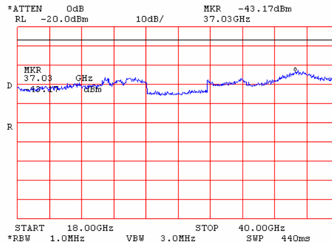
Plot 7.17.29 Conducted emission measurements from 18 to 40 GHz at the 5.32GHz carrier frequency
