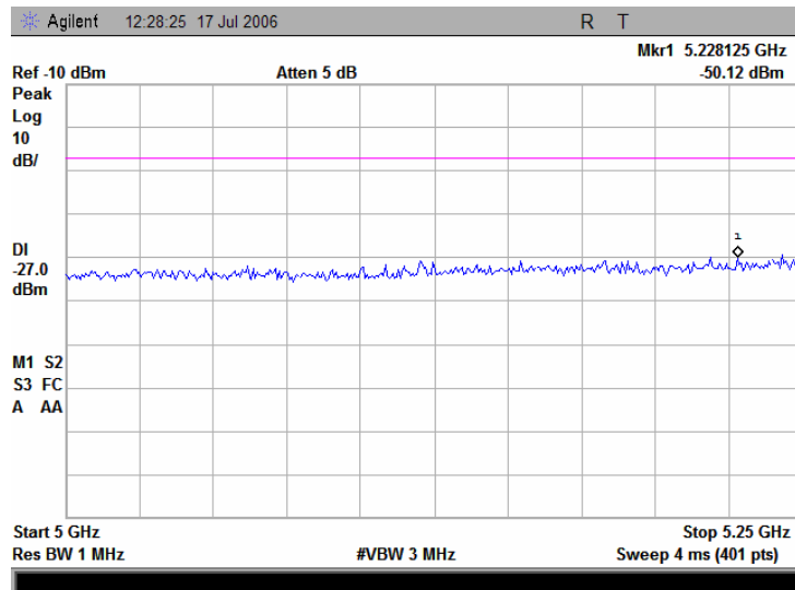
Plot 7.16.26 Conducted emission measurements from 5.0 to 5.25 GHz at the 5.32 GHz carrier frequency
