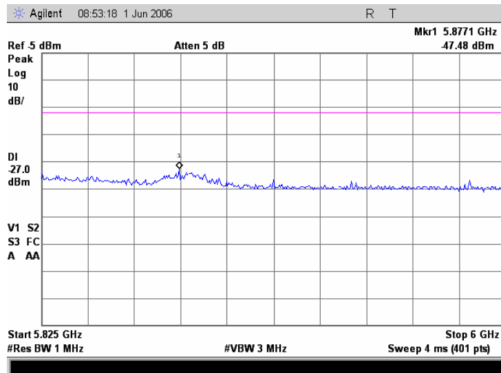
Plot 7.17.33 Conducted emission measurements from 5.825 to 6.0 GHz at the 5.745 GHz carrier frequency
