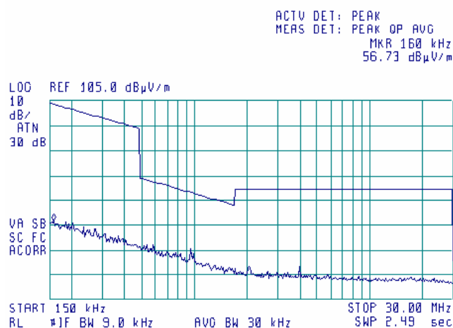
Plot 7.15.10 Radiated emission measurements from 0.15 to 30 MHz at the 5.745GHz carrier frequency
