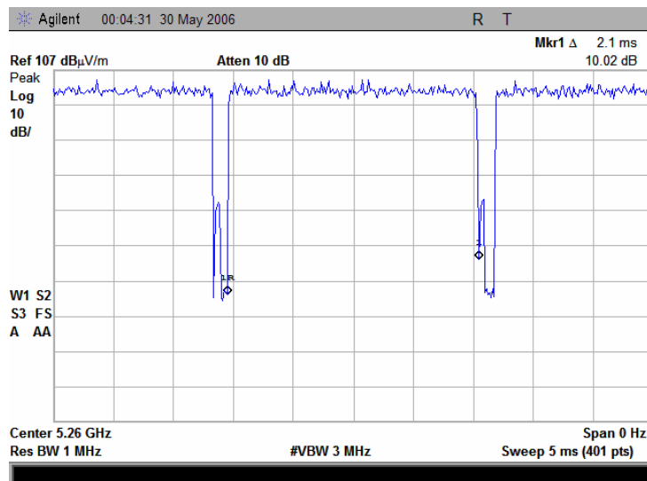
Plot 7.15.146 Transmission burst duration
