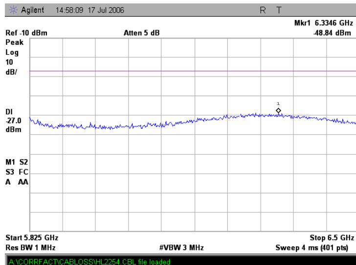
Plot 7.16.36 Conducted emission measurements from 5.825 to 6.5 GHz at the 5.785 GHz carrier frequency
