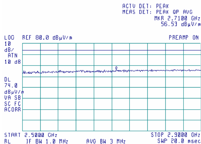
Plot 7.14.60 Radiated emission measurements from 2.5 to 2.9 GHz at the 5.32 GHz carrier frequency
