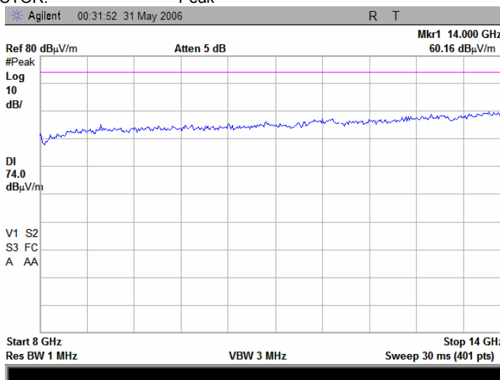
Plot 7.14.86 Radiated emission measurements from 8 to 14 GHz at the 5.745 GHz carrier frequency
