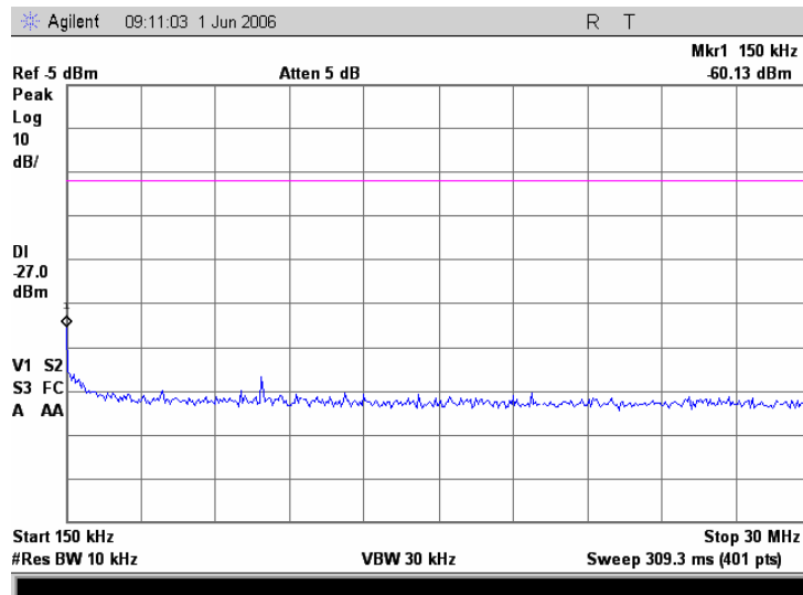
Plot 7.17.12 Conducted emission measurements from 0.15 to 30 MHz at the 5.805GHz carrier frequency
