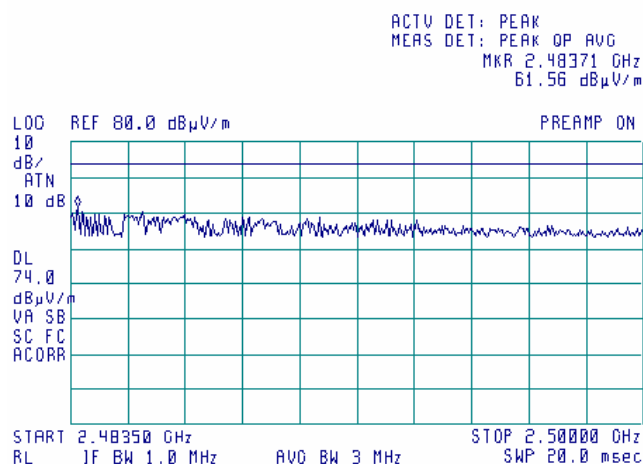
Plot 7.14.58 Radiated emission measurements from 2.4835 to 2.5GHz at the 5.32 GHz carrier frequency
