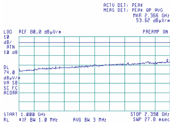
Plot 7.14.20 Radiated emission measurements from 1.0 to 2.39 GHz at the 5.18 GHz carrier frequency
