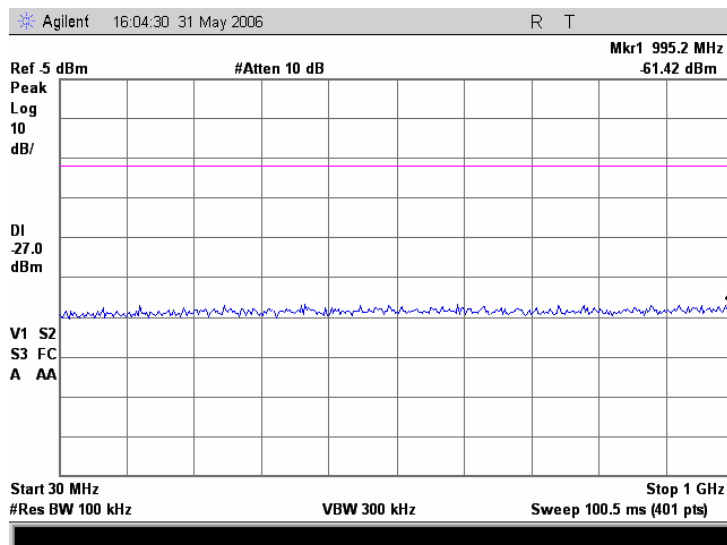
Plot 7.17.16 Conducted emission measurements from 30 to 1000 MHz at the 5.745GHz carrier frequency
