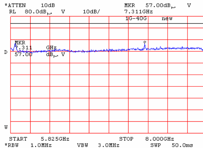
Plot 7.15.84 Radiated emission measurements from 5.825 to 8.0 GHz at the 5.745 GHz carrier frequency
