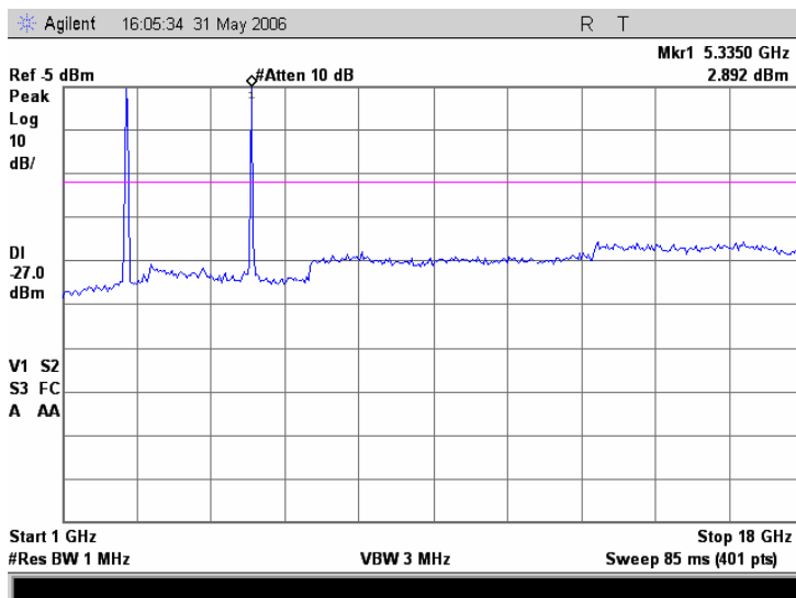
Plot 7.17.25 Conducted emission measurements from 1.0 to 18 GHz at the 5.32 GHz carrier frequency
