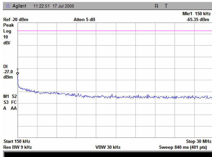
Plot 7.16.12 Conducted emission measurements from 0.15 to 30 MHz at the 5.805GHz carrier frequency
