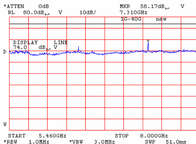
Plot 7.15.66 Radiated emission measurements from 5.46 to 8.0 GHz at the 5.32GHz carrier frequency
