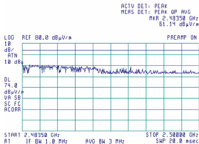
Plot 7.15.22 Radiated emission measurements from 2.4835 to 2.5GHz at the 5.18GHz carrier frequency
