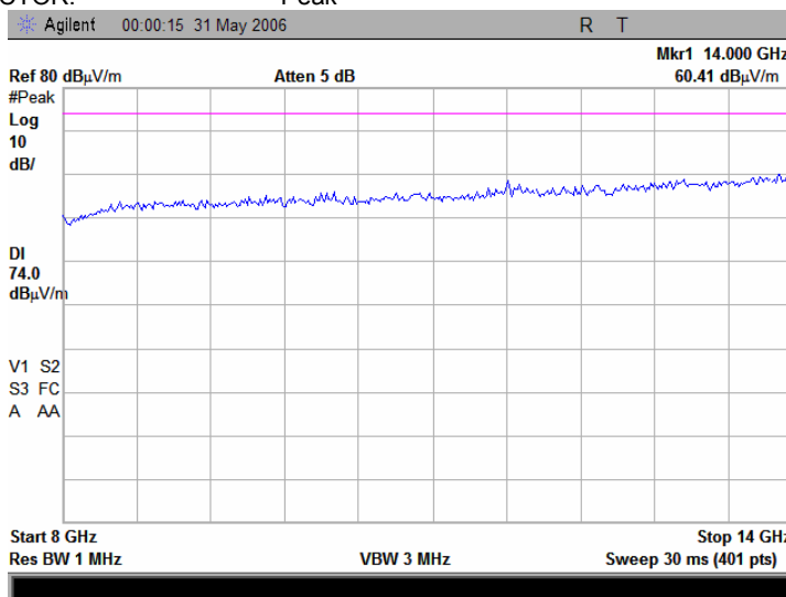
Plot 7.15.124 Radiated emission measurements from 8 to 14 GHz at the 5.805 GHz carrier frequency
