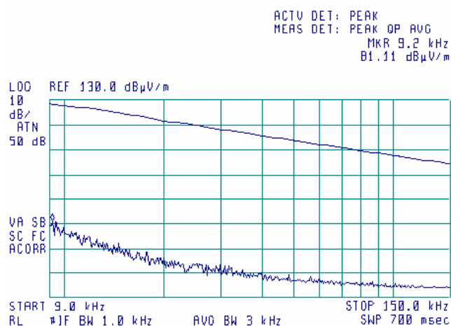
Plot 7.14.2 Radiated emission measurements from 9 to 150 kHz at the 5.26GHz carrier frequency
