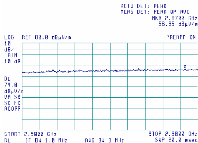
Plot 7.14.24 Radiated emission measurements from 2.5 to 2.9 GHz at the 5.18GHz carrier frequency
