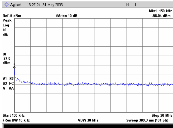
Plot 7.17.10 Conducted emission measurements from 0.15 to 30 MHz at the 5.745GHz carrier frequency
