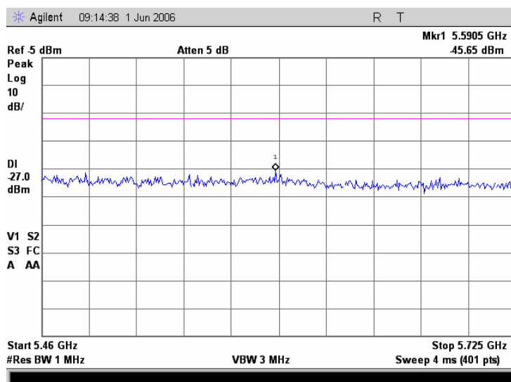
Plot 7.17.42 Conducted emission measurements from 5.46 to 5.725 GHz at the 5.805 GHz carrier frequency
