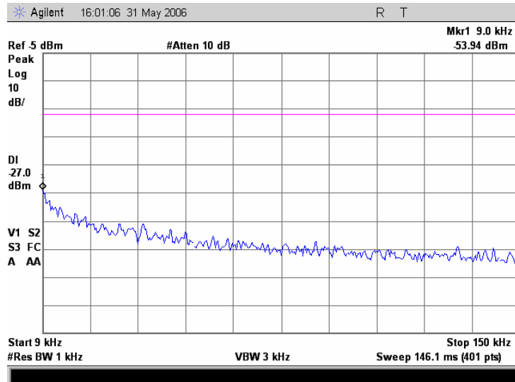
Plot 7.17.4 Conducted emission measurements from 9 to 150 kHz at the 5.745GHz carrier frequency
