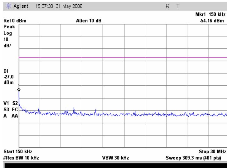
Plot 7.17.8 Conducted emission measurements from 0.15 to 30 MHz at the 5.26GHz carrier frequency
