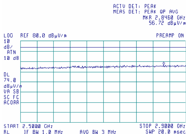
Plot 7.14.116 Radiated emission measurements from 2.5 to 2.9 GHz at the 5.805 GHz carrier frequency
