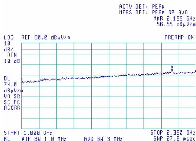
Plot 7.14.56 Radiated emission measurements from 1.0 to 2.39 GHz at the 5.32 GHz carrier frequency
