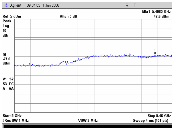
Plot 7.17.36 Conducted emission measurements from 5.0 to 5.46 GHz at the 5.785 GHz carrier frequency
