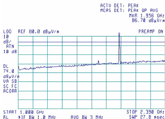
Plot 7.15.56 Radiated emission measurements from 1.0 to 2.39 GHz at the 5.32 GHz carrier frequency
