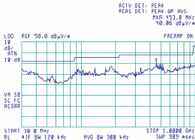
Plot 7.14.18 Radiated emission measurements from 30 to 1000 MHz at the 5.805GHz carrier frequency
