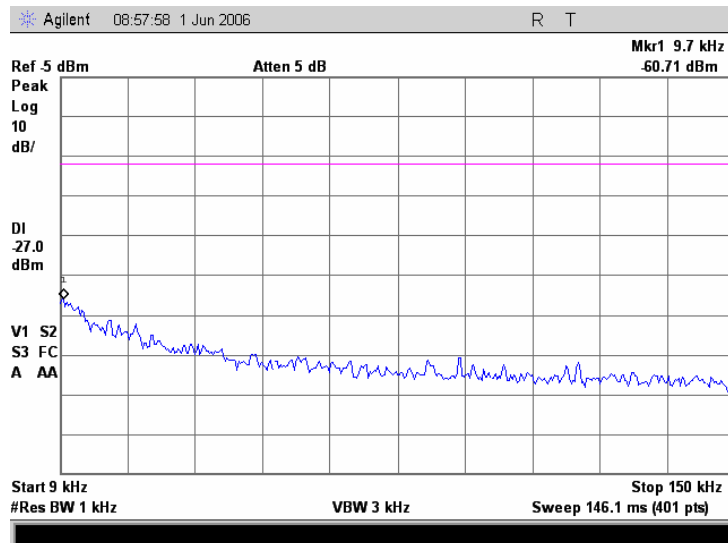
Plot 7.17.6 Conducted emission measurements from 9 to 150 kHz at the 5.805GHz carrier frequency
