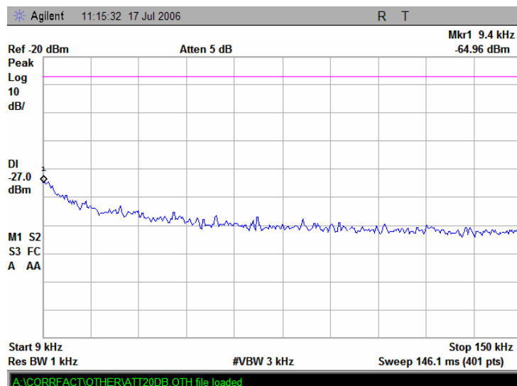
Plot 7.16.6 Conducted emission measurements from 9 to 150 kHz at the 5.805GHz carrier frequency
