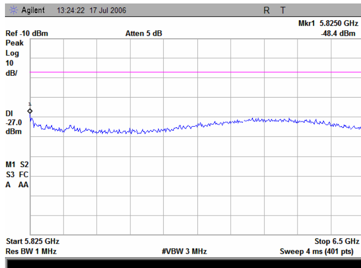
Plot 7.16.40 Conducted emission measurements from 5.825 to 6.5 GHz at the 5.805 GHz carrier frequency
