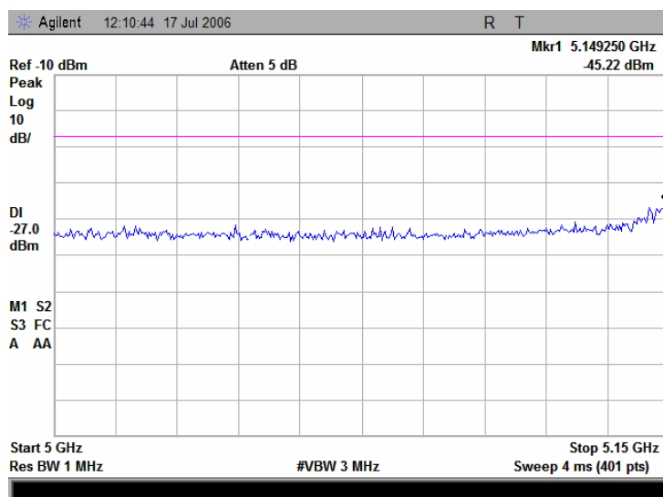
Plot 7.16.20 Conducted emission measurements from 5.0 to 5.15 GHz at the 5.18 GHz carrier frequency
