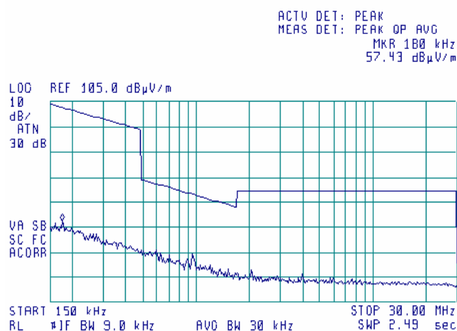
Plot 7.14.8 Radiated emission measurements from 0.15 to 30 MHz at the 5.26GHz carrier frequency
