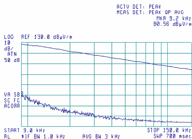
Plot 7.14.4 Radiated emission measurements from 9 to 150 kHz at the 5.745GHz carrier frequency
