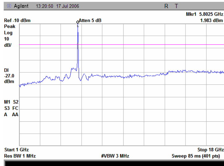
Plot 7.16.38 Conducted emission measurements from 1.0 to 18 GHz at the 5.805 GHz carrier frequency
