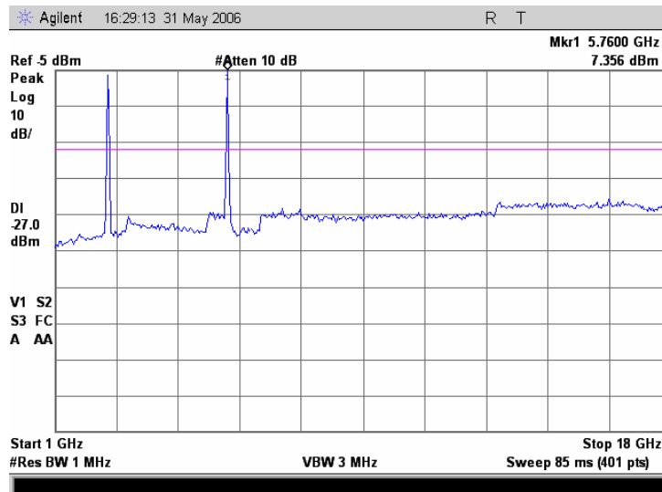
Plot 7.17.30 Conducted emission measurements from 1.0 to 18.0 GHz at the 5.745 GHz carrier frequency
