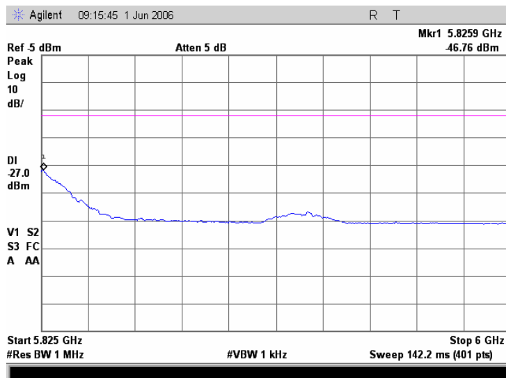
Plot 7.17.43 Conducted emission measurements from 5.825 to 6.0 GHz at the 5.805 GHz carrier frequency
