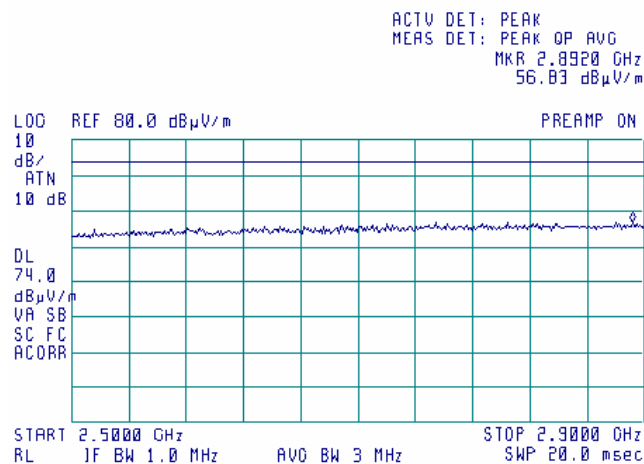
Plot 7.15.60 Radiated emission measurements from 2.5 to 2.9 GHz at the 5.32 GHz carrier frequency
