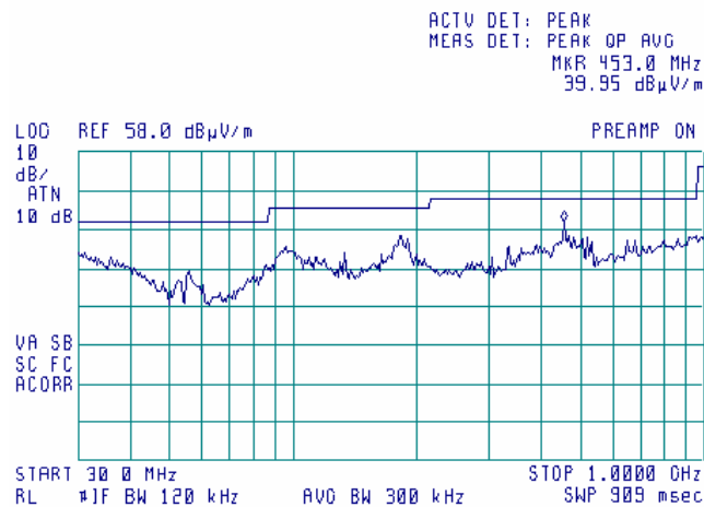
Plot 7.14.16 Radiated emission measurements from 30 to 1000 MHz at the 5.745GHz carrier frequency
