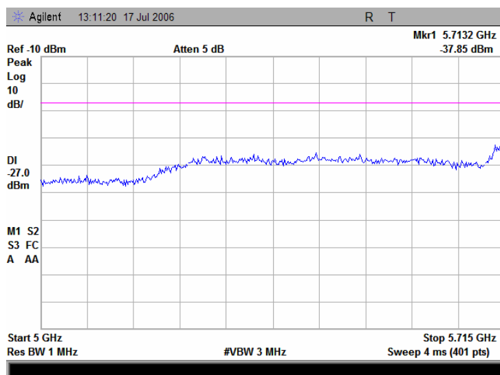
Plot 7.16.30 Conducted emission measurements from 5.0 to 5.715 GHz at the 5.745 GHz carrier frequency
