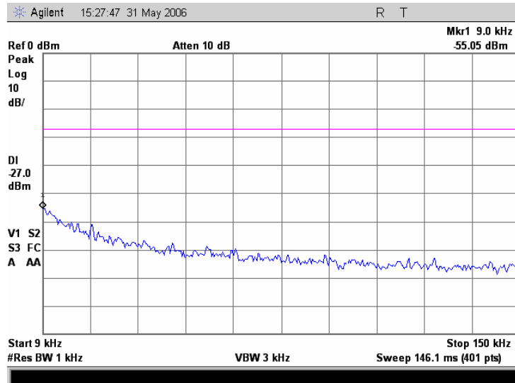
Plot 7.17.2 Conducted emission measurements from 9 to 150 kHz at the 5.26GHz carrier frequency
