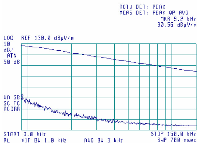
Plot 7.15.4 Radiated emission measurements from 9 to 150 kHz at the 5.745GHz carrier frequency
