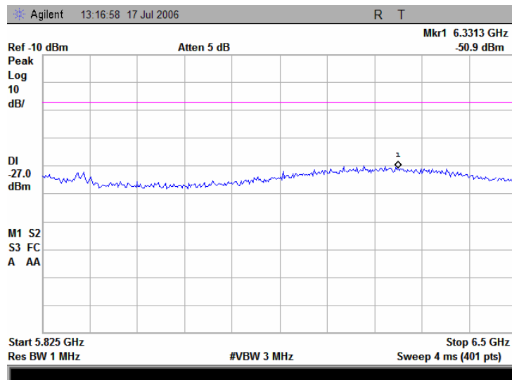
Plot 7.16.32 Conducted emission measurements from 5.825 to 6.5 GHz at the 5.745 GHz carrier frequency
