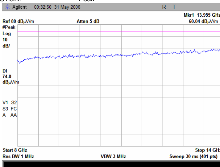
Plot 7.15.32 Radiated emission measurements from 8.0 to 14.0 GHz at the 5.18 GHz carrier frequency
