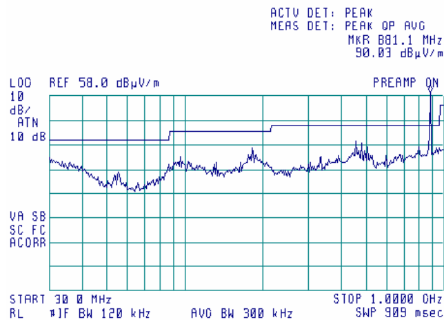
Plot 7.15.16 Radiated emission measurements from 30 to 1000 MHz at the 5.745GHz carrier frequency
