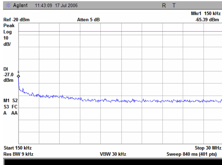
Plot 7.16.11 Conducted emission measurements from 0.15 to 30 MHz at the 5.785GHz carrier frequency
