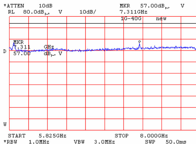
Plot 7.14.84 Radiated emission measurements from 5.825 to 8.0 GHz at the 5.745 GHz carrier frequency
