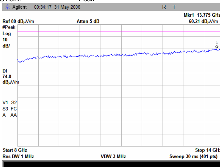
Plot 7.15.86 Radiated emission measurements from 8 to 14 GHz at the 5.745 GHz carrier frequency
