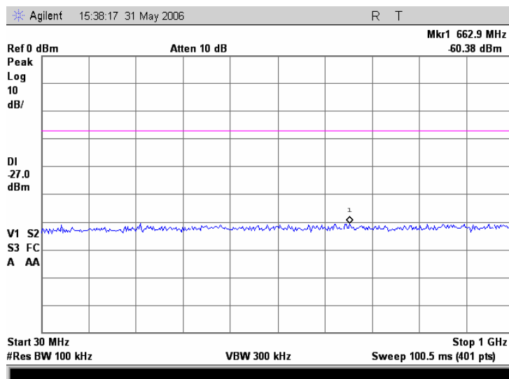
Plot 7.17.14 Conducted emission measurements from 30 to 1000 MHz at the 5.26GHz carrier frequency
