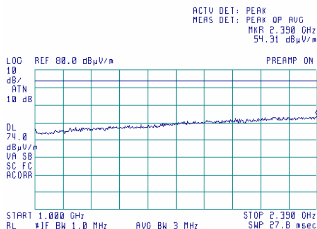
Plot 7.14.112 Radiated emission measurements from 1.0 to 2.39 GHz at the 5.805 GHz carrier frequency
