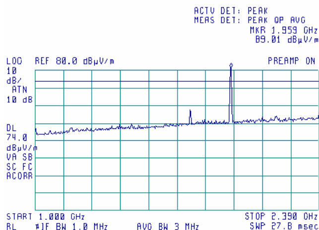
Plot 7.15.20 Radiated emission measurements from 1.0 to 2.39 GHz at the 5.18 GHz carrier frequency
