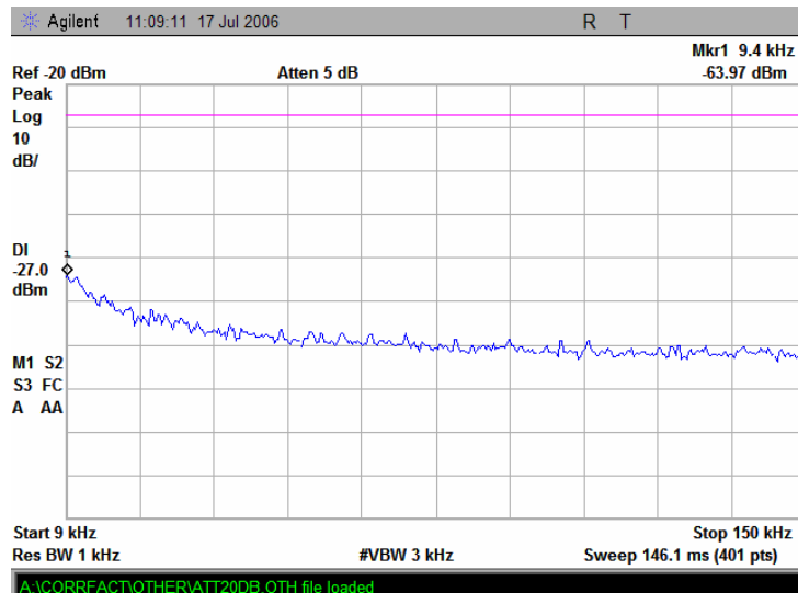
Plot 7.16.2 Conducted emission measurements from 9 to 150 kHz at the 5.26GHz carrier frequency
