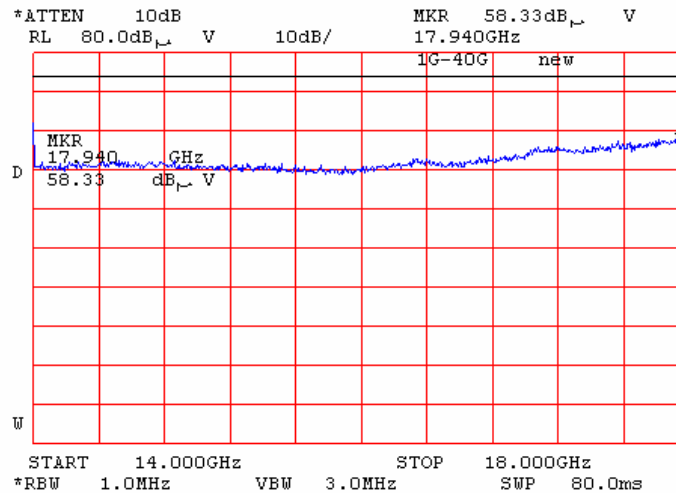
Plot 7.15.126 Radiated emission measurements from 14 to 18 GHz at the 5.805GHz carrier frequency
