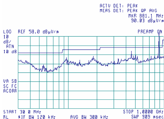
Plot 7.15.18 Radiated emission measurements from 30 to 1000 MHz at the 5.805GHz carrier frequency
