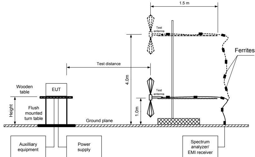
Figure 7.15.2 Setup for spurious emission field strength measurements above 30 MHz
