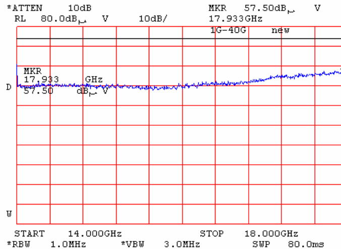
Plot 7.14.70 Radiated emission measurements from 14 to 18 GHz at the 5.32 GHz carrier frequency
