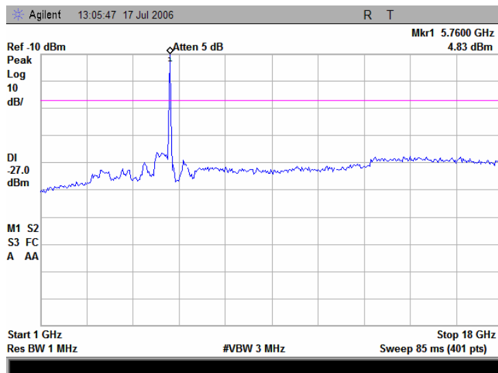
Plot 7.16.29 Conducted emission measurements from 1.0 to 18.0 GHz at the 5.745 GHz carrier frequency
