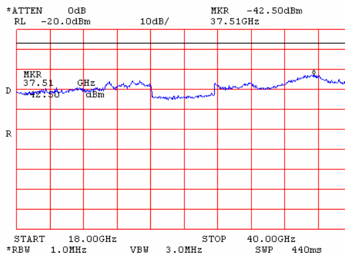
Plot 7.17.44 Conducted emission measurements from 18 to 40 GHz at the 5.805GHz carrier frequency
