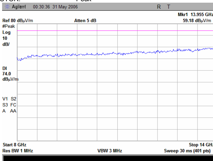
Plot 7.14.32 Radiated emission measurements from 8.0 to 14.0 GHz at the 5.18GHz carrier frequency
