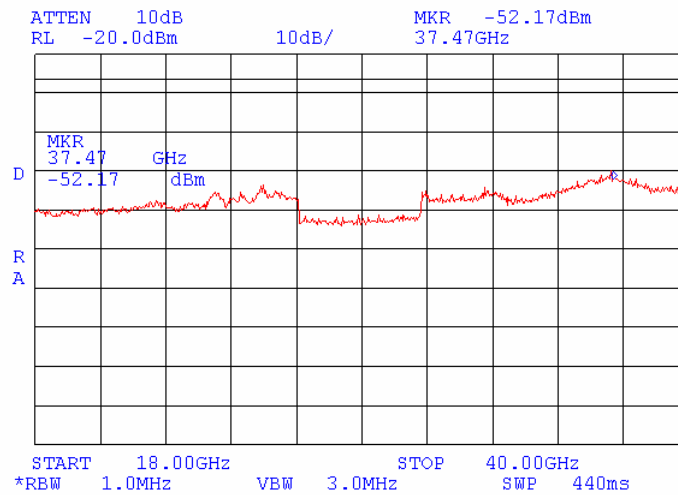
Plot 7.16.41 Conducted emission measurements from 18 to 40 GHz at the 5.805GHz carrier frequency
