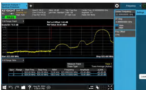
Band26(824-849)-1.4MHz-QPSK-26797-1RB#5-PASS
