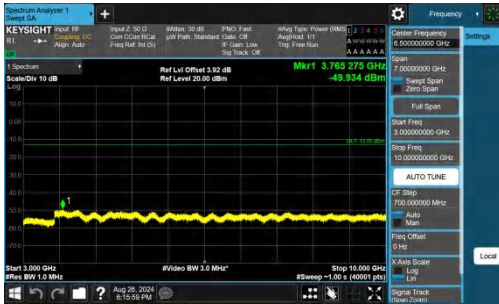
Band26(824-849)-15MHz-QPSK-26965-1RB#0-3000~10000-PAS
