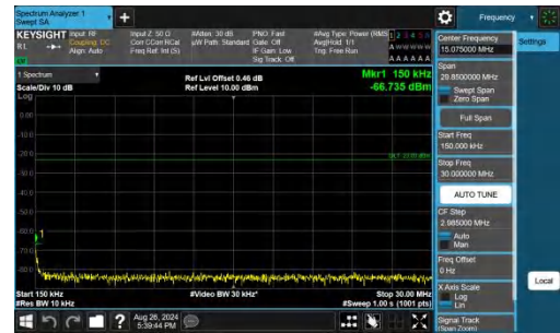
Band26(824-849)-1.4MHz-QPSK-26797-1RB#0-0.15~30-PASS
