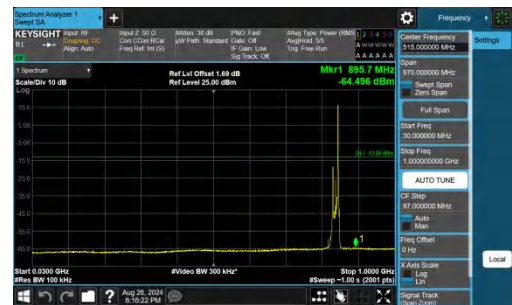
Band26(824-849)-15MHz-QPSK-26965-1RB#74-30~1000-PASS
