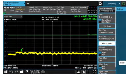
Band26(824-849)-1.4MHz-QPSK-26915-1RB#5-3000~10000-PASS S
