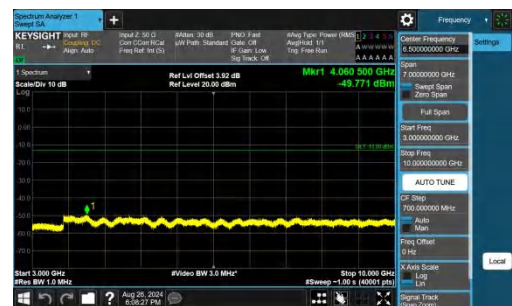
Band26(824-849)-10MHz-QPSK-26990-1RB#49-3000~10000-PAS
