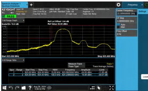
Band26(824-849)-1.4MHz-QPSK-26797-1RB#0-PASS
