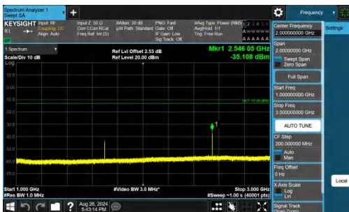
Band26(824-849)-1.4MHz-QPSK-27033-1RB#5-1000~3000-PASS
