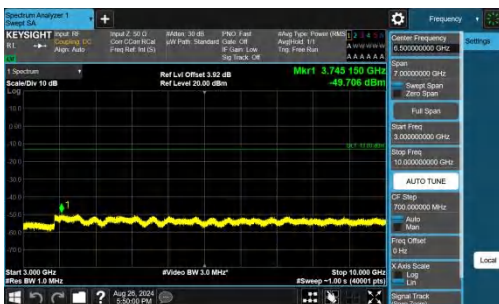
Band26(824-849)-3MHz-QPSK-26915-1RB#0-3000~10000-PASS
