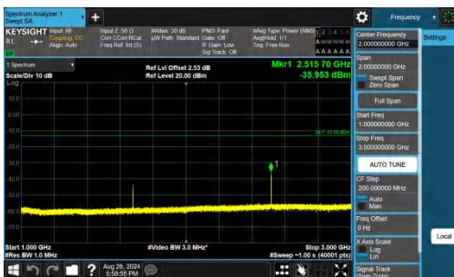
Band26(824-849)-5MHz-QPSK-26915-1RB#24-1000~3000-PASS
