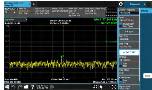
Band26(824-849)-15MHz-QPSK-26965-1RB#74-0.009~0.15-PASS
