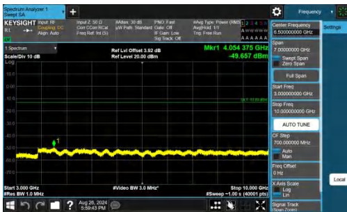
Band26(824-849)-5MHz-QPSK-27015-1RB#0-3000~10000-PASS
