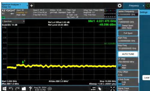
Band26(824-849)-10MHz-QPSK-26840-1RB#0-3000~10000-PAS
