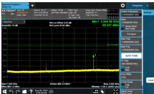
Band26(824-849)-15MHz-QPSK-26965-1RB#74-1000~3000-PAS
