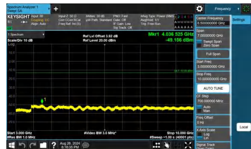
Band26(824-849)-15MHz-QPSK-26965-1RB#74-3000~10000-PAS
