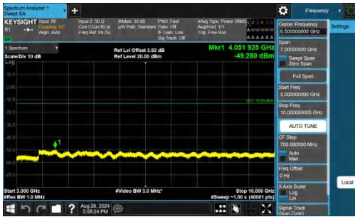
Band26(824-849)-5MHz-QPSK-26915-1RB#0-3000~10000-PASS
