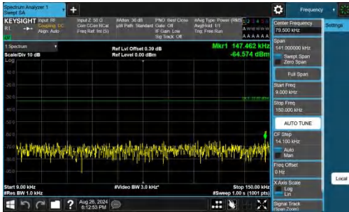
Band26(824-849)-15MHz-QPSK-26865-1RB#0-0.009~0.15-PASS
