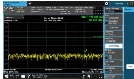
Band26(824-849)-5MHz-QPSK-26815-1RB#24-0.009~0.15-PASS
