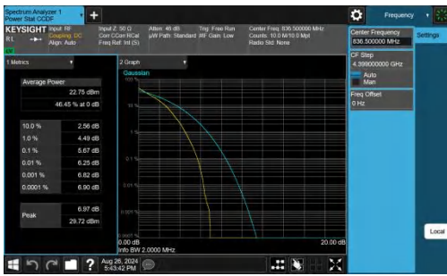
Band26(824-849)-1.4MHz-QPSK-26915-6RB#0-PASS
