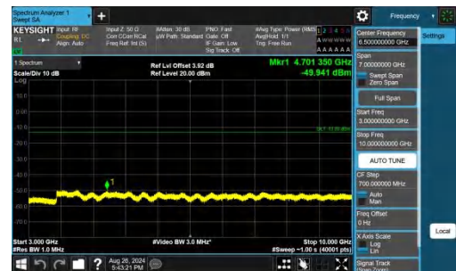
Band26(824-849)-1.4MHz-QPSK-27033-1RB#5-3000~10000-PAS S
