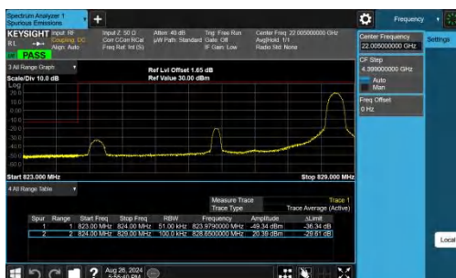
Band26(824-849)-5MHz-QPSK-26815-1RB#24-PASS
