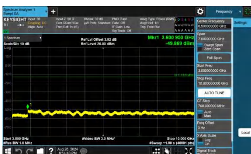
Band26(824-849)-15MHz-QPSK-26915-1RB#0-3000~10000-PAS
