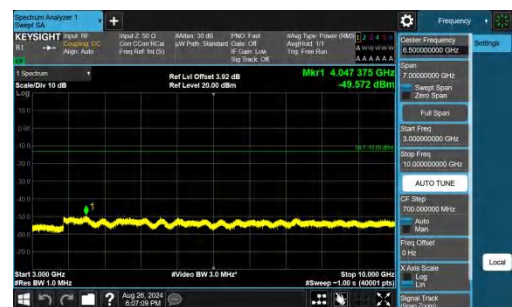
Band26(824-849)-10MHz-QPSK-26915-1RB#49-3000~10000-PAS S
