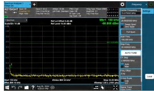
Band26(824-849)-10MHz-QPSK-26840-1RB#0-0.15~30-PASS
