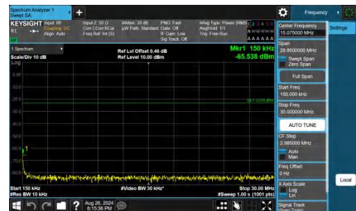
Band26(824-849)-15MHz-QPSK-26965-1RB#0-0.15~30-PASS
