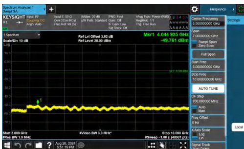
Band26(824-849)-3MHz-QPSK-27025-1RB#0-3000~10000-PASS
