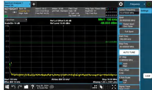
Band26(824-849)-15MHz-QPSK-26865-1RB#0-0.15~30-PASS
