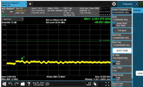
Band26(824-849)-5MHz-QPSK-26815-1RB#0-3000~10000-PASS
