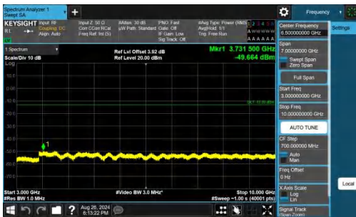
Band26(824-849)-15MHz-QPSK-26865-1RB#0-3000~10000-PASS
