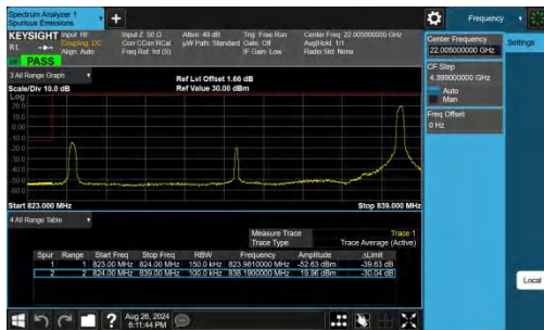
Band26(824-849)-15MHz-QPSK-26865-1RB#74-PASS
