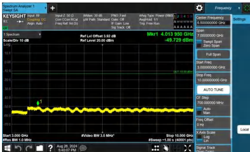
Band26(824-849)-1.4MHz-QPSK-26797-1RB#0-3000~10000-PAS
