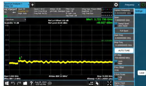
Band26(824-849)-5MHz-QPSK-26815-1RB#24-3000~10000-PASS
