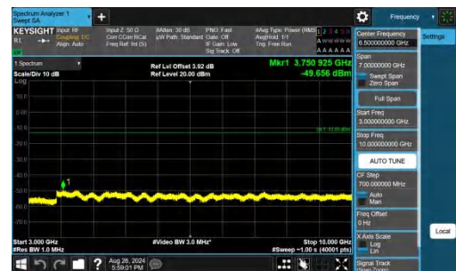
Band26(824-849)-5MHz-QPSK-26915-1RB#24-3000~10000-PASS
