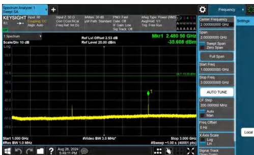
Band26(824-849)-3MHz-QPSK-26805-1RB#14-1000~3000-PASS
