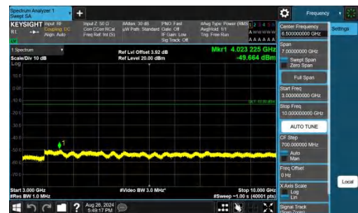
Band26(824-849)-3MHz-QPSK-26805-1RB#14-3000~10000-PASS
