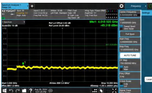
Band26(824-849)-1.4MHz-QPSK-26915-1RB#0-3000~10000-PASS
