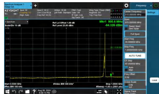
Band26(824-849)-10MHz-QPSK-26990-1RB#49-30~1000-PASS
