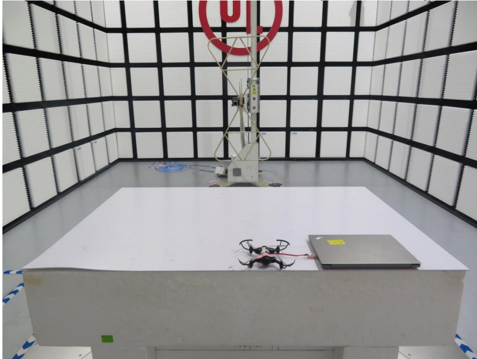
WIFI Module RADIATED RF MEASUREMENT SETUP (30MHz ~ 1 GHz)
