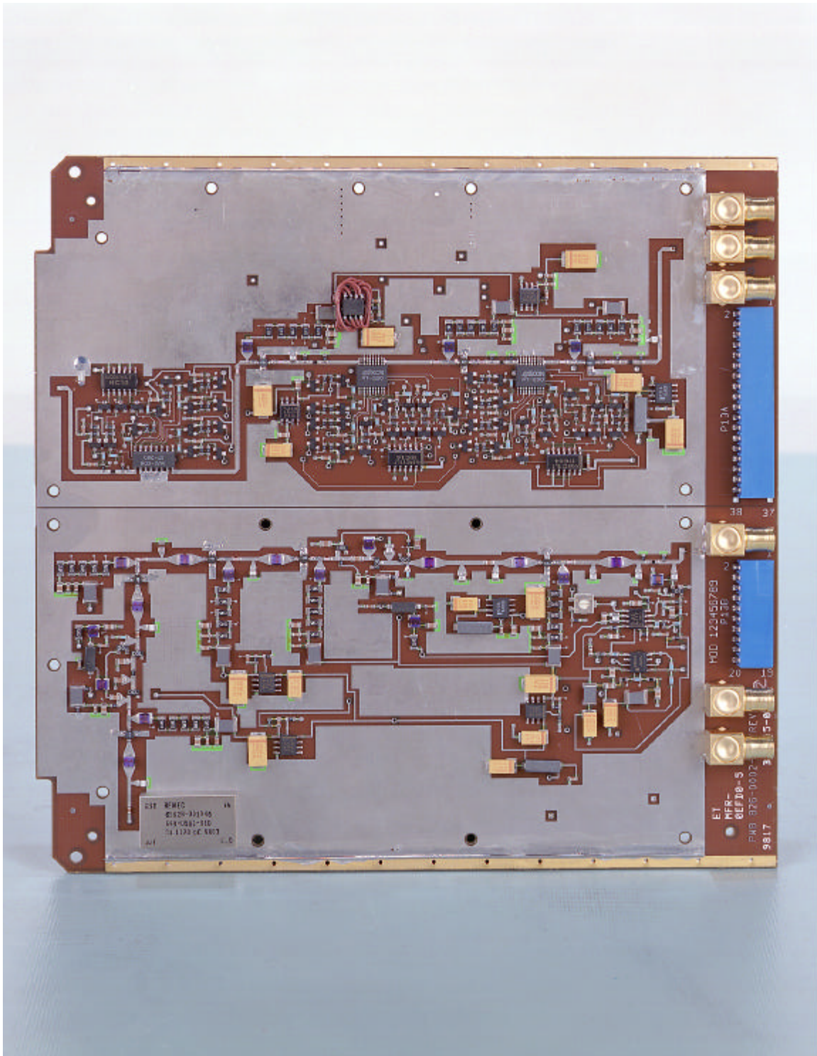
Figure 8-7 Up/Down Converter Card Assembly (Bottom View)
