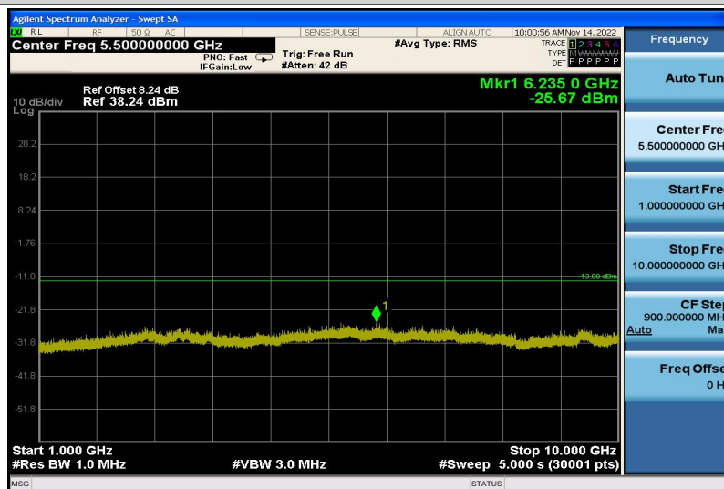
GSM850-251-1000~10000
