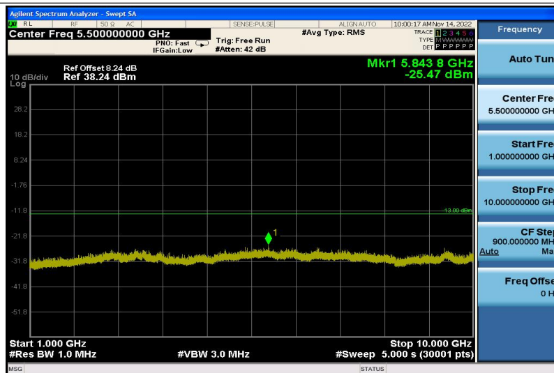
GSM850-190-1000~10000
