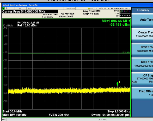
11B-Ant1-2437-30~1000-3.37
