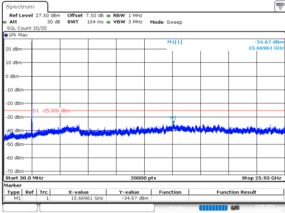
5MHz_Middle_QPSK_1@0 -34.67dBm
