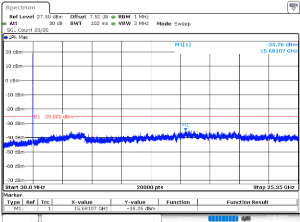
15MHz_Middle_QPSK_75@0 -35.26dBm
