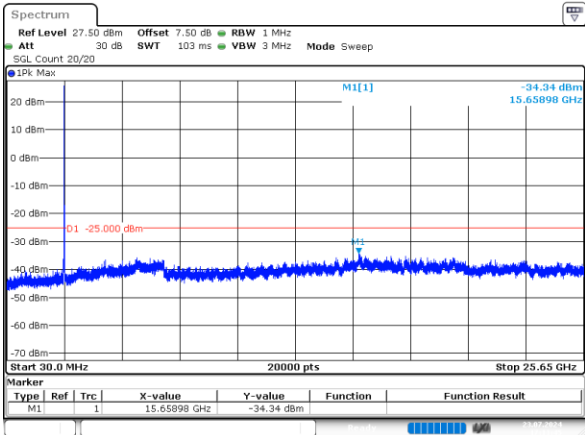
3_20MHz_Low_QPSK_1@0 -34.34dBm
