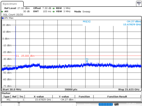
15MHz_High_QPSK_75@0 -34.27dBm
