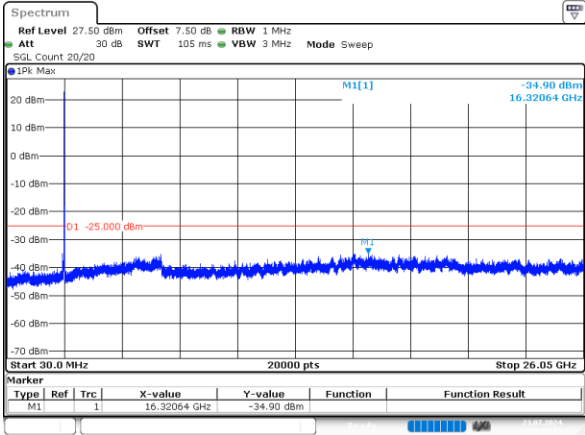
3_20MHz_Middle_QPSK_1@0 -34.90dBm
