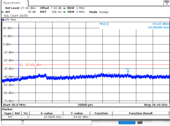
3_20MHz_High_QPSK_1@0 -34.62dBm
