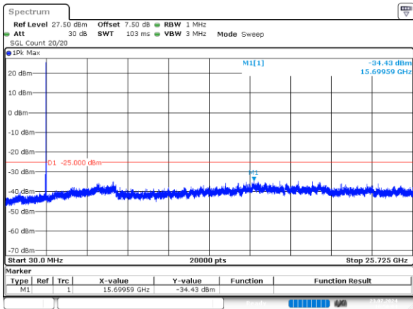
5MHz_Low_QPSK_1@0 -34.43dBm
