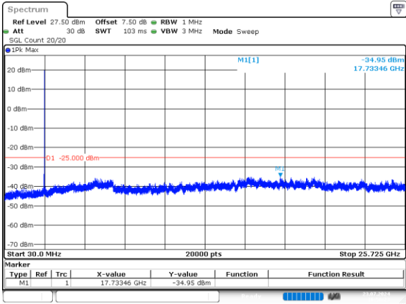
5MHz_Low_QPSK_25@0 -34.95dBm
