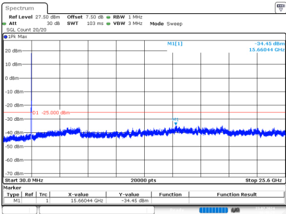
20MHz_High_QPSK_100@0 -34.45dBm
