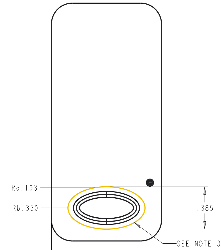
BACK SIDE
