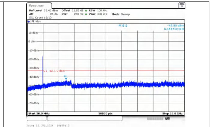
30.0 MHz - 25000.0 MHz IEEE 802.11n_Channel 9_40MHz_Antenna 0
