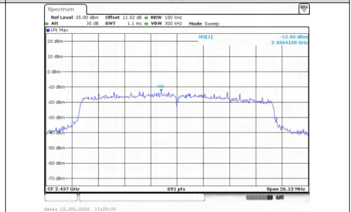
In-Band Reference Level IEEE 802.11ax_Channel 6_20MHz_Antenna 0_RU&Index SU
