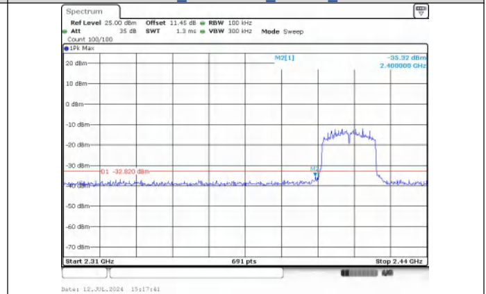
Out Of Band Emission IEEE 802.11ax_Channel 1_20MHz_Antenna 0_RU&Index SU
