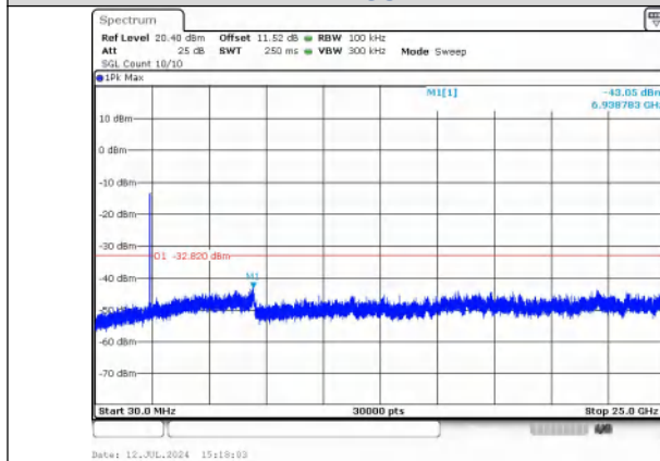
30.0 MHz - 25000.0 MHz IEEE 802.11ax_Channel 1_20MHz_Antenna 0_RU&Index SU
