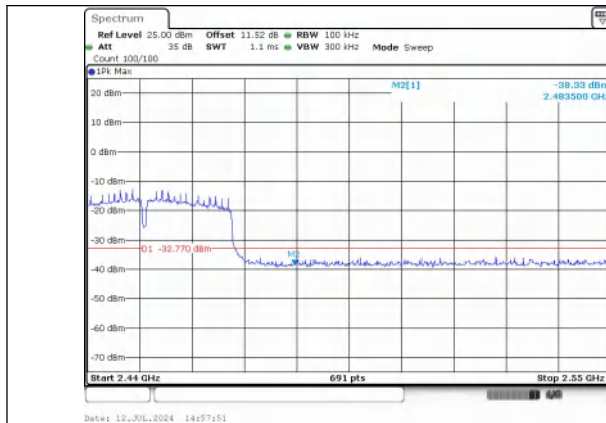
Out Of Band Emission IEEE 802.11n_Channel 9_40MHz_Antenna 0
