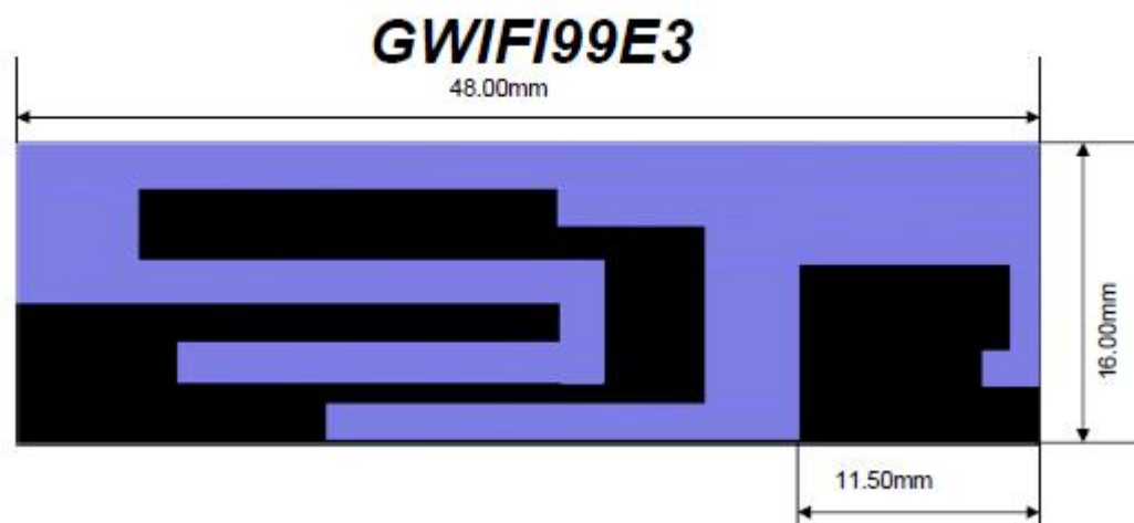
5. Antenna layout
