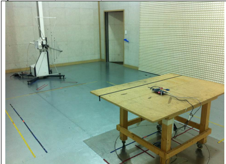
Photo of radiated spurious emission (30 MHz ~ 1 GHz)
