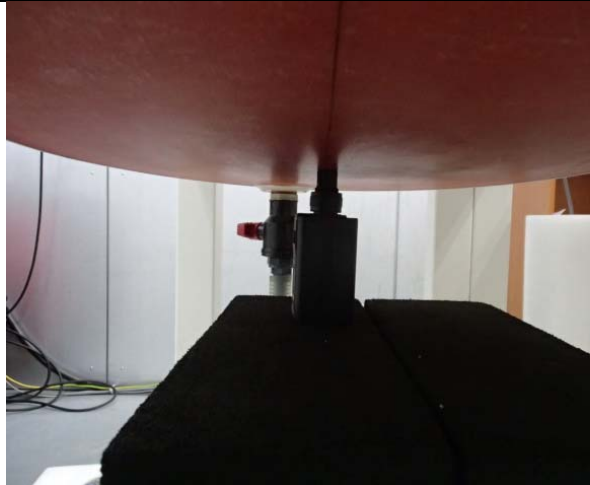
Photograph B10: Body, Top, 0mm (Side view)
