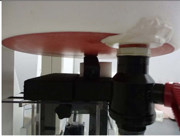
Photograph B14: Body, Right tilt, 0mm (Side view)
