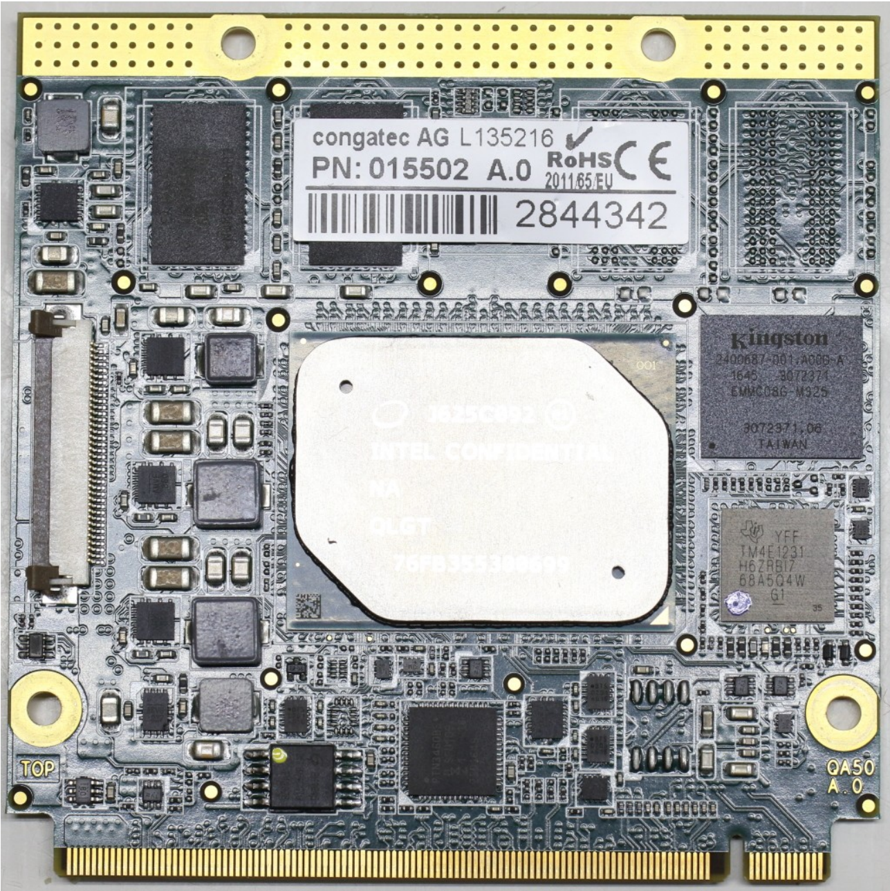
congatec QA5 x86 PCB [2]
