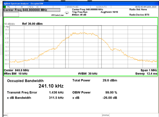
EGPRS_850_Higher_26BW and 99%
