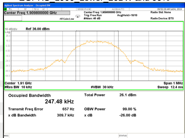
EGPRS_1900_Higher_26BW and 99%
