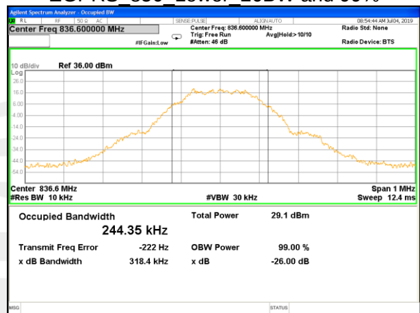
EGPRS_850_Middle_26BW and 99%
