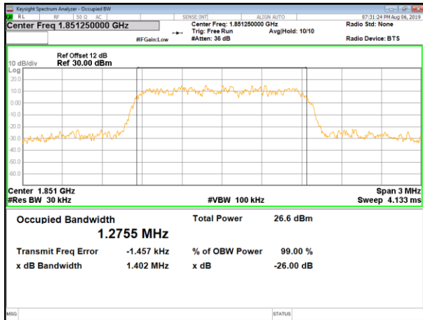
BC1_CDMA_Lower_26BW and 99%
