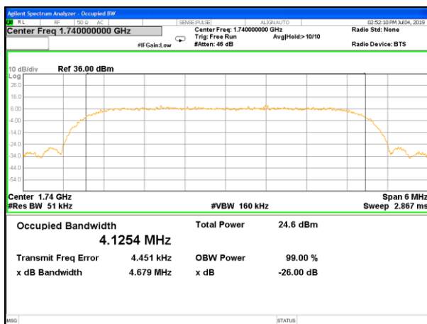
B4_HSUPA_Middle_26BW and 99%
