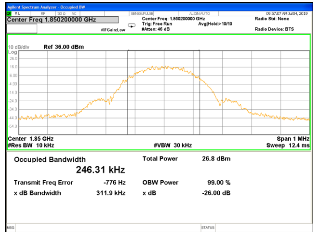
EGPRS_1900_Lower_26BW and 99%
