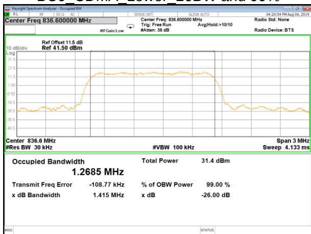
BC0_CDMA_Middle_26BW and 99%
