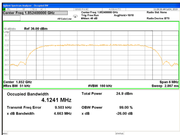
B2_HSDPA_Lower_26BW and 99%
