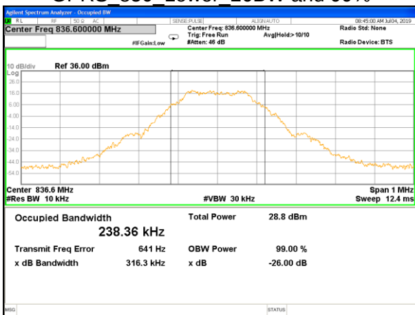
GPRS_850_Middle_26BW and 99%
