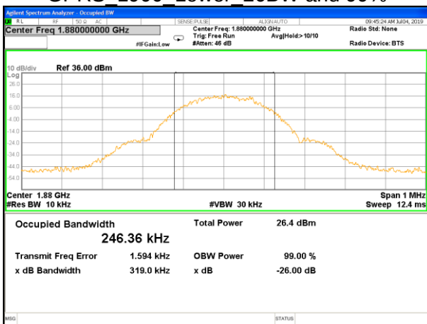
GPRS_1900_Middle_26BW and 99%
