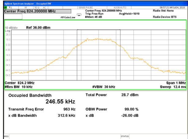
EGPRS_850_Lower_26BW and 99%
