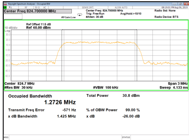
BC0_EVDO_Lower_26BW and 99%
