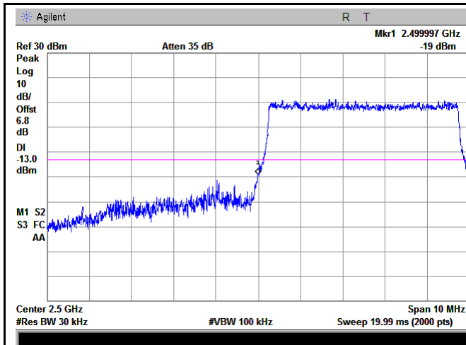
LTE Band 7 - Low Channel QPSK-5
