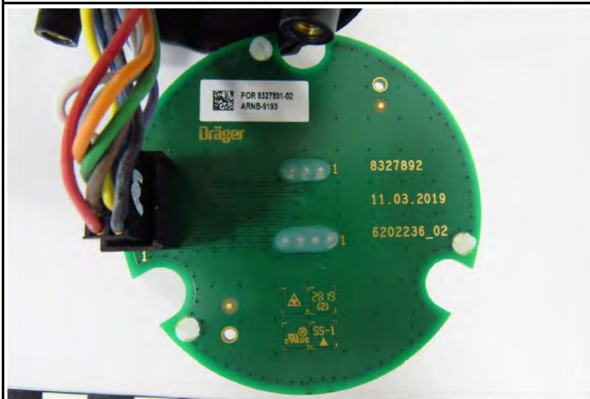
Sensor interface PCB bottom side view
