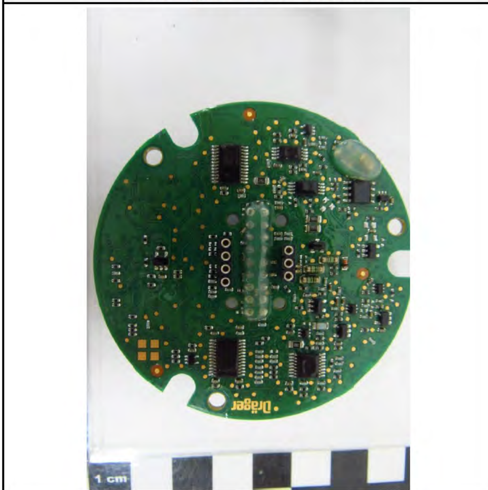
Sensor logic PCB bottom side view
