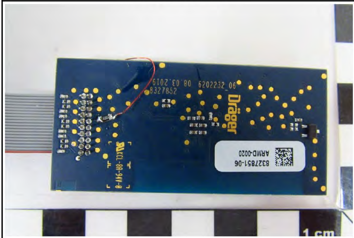
LE PCB bottom view
