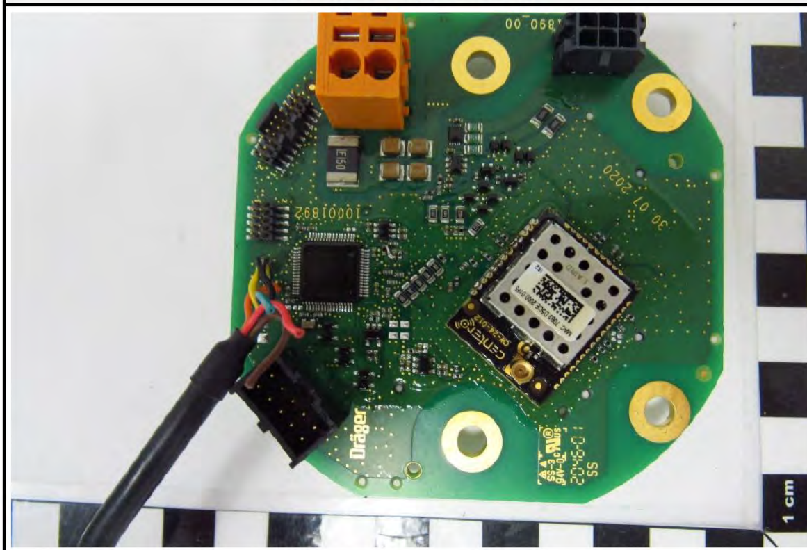
Main PCB top side view
