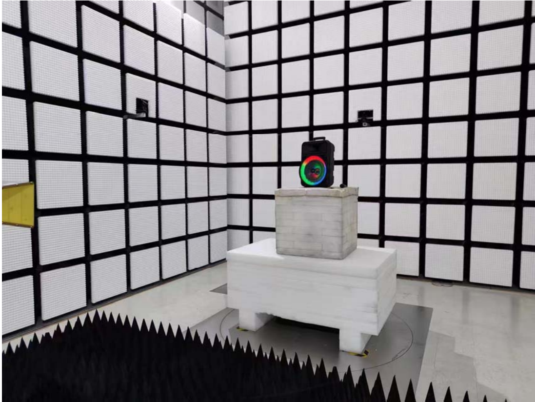
Radiated Emission Above 1G View- Power by DC power port
