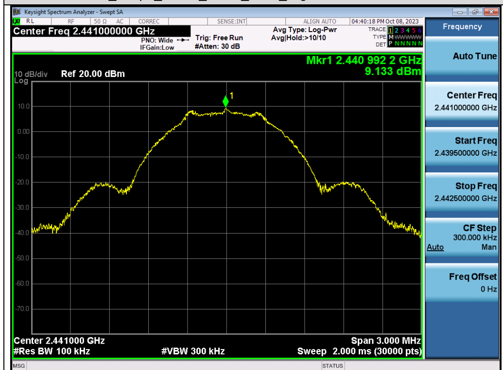
Test_Graph_GFSK_ANT1_2441_Reference Level
