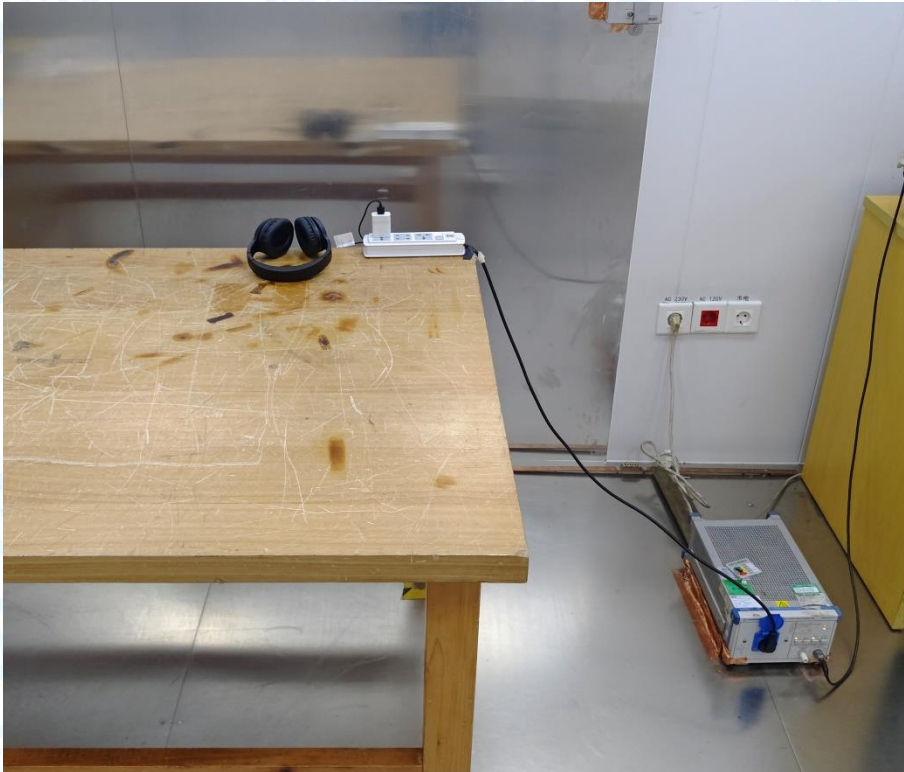
Photo of Setup for Conducted Emission
