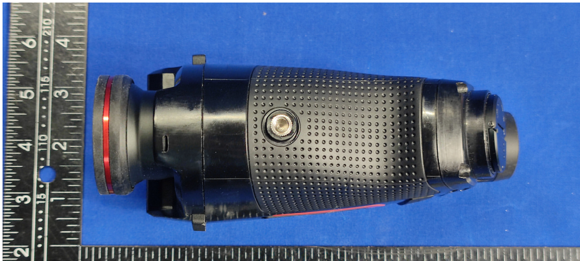
EUT View 9
