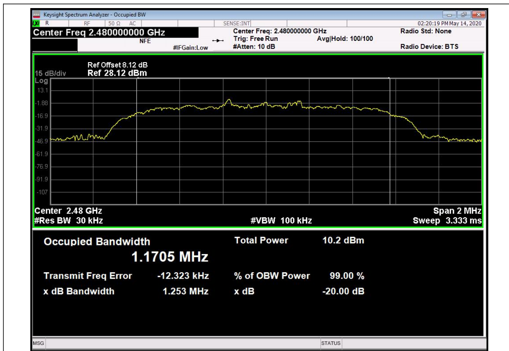
(π/4-DQPSK, Channel 78, 2480MHz)
