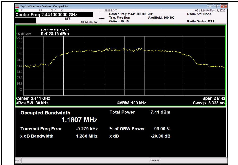
(π/4-DQPSK, Channel 39, 2441MHz)
