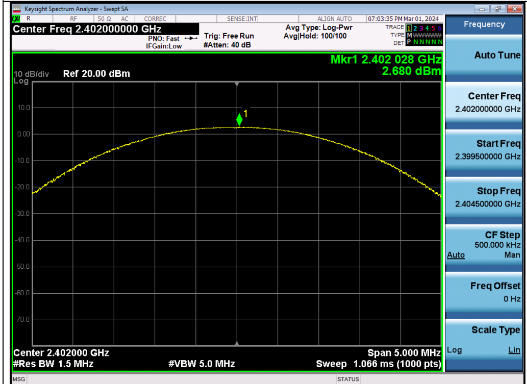
Test_Graph_EDR_ANT1_2402_2Mbps_Peak Power
