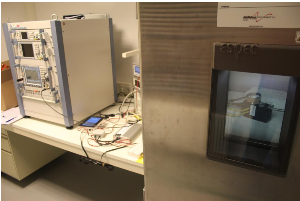
Photo 7 Photograph test setup Carrier stability
