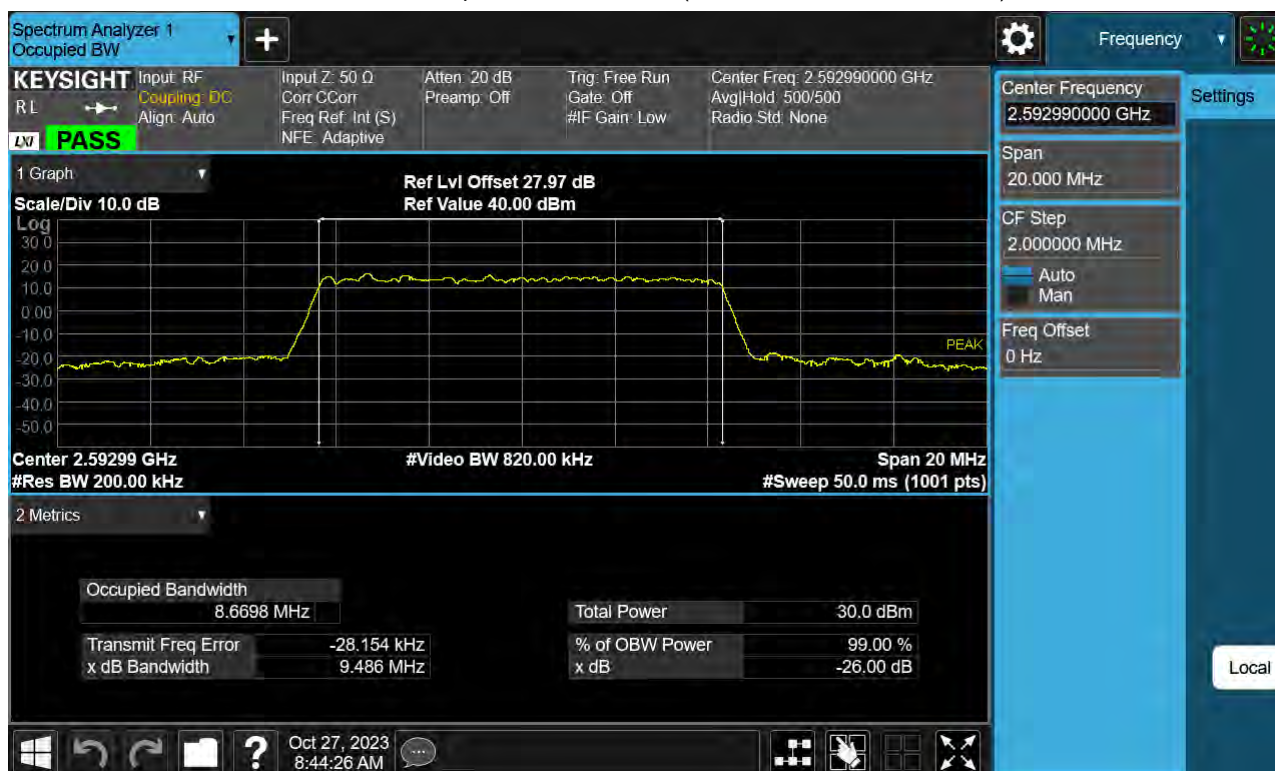
Sub6 n41. Occupied Bandwidth Plot (10 MHz Ch.518598 16-QAM )
