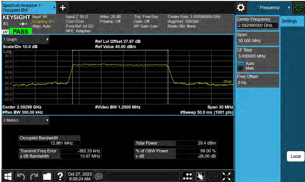
Sub6 n41. Occupied Bandwidth Plot (15 MHz Ch.518598 64-QAM )
