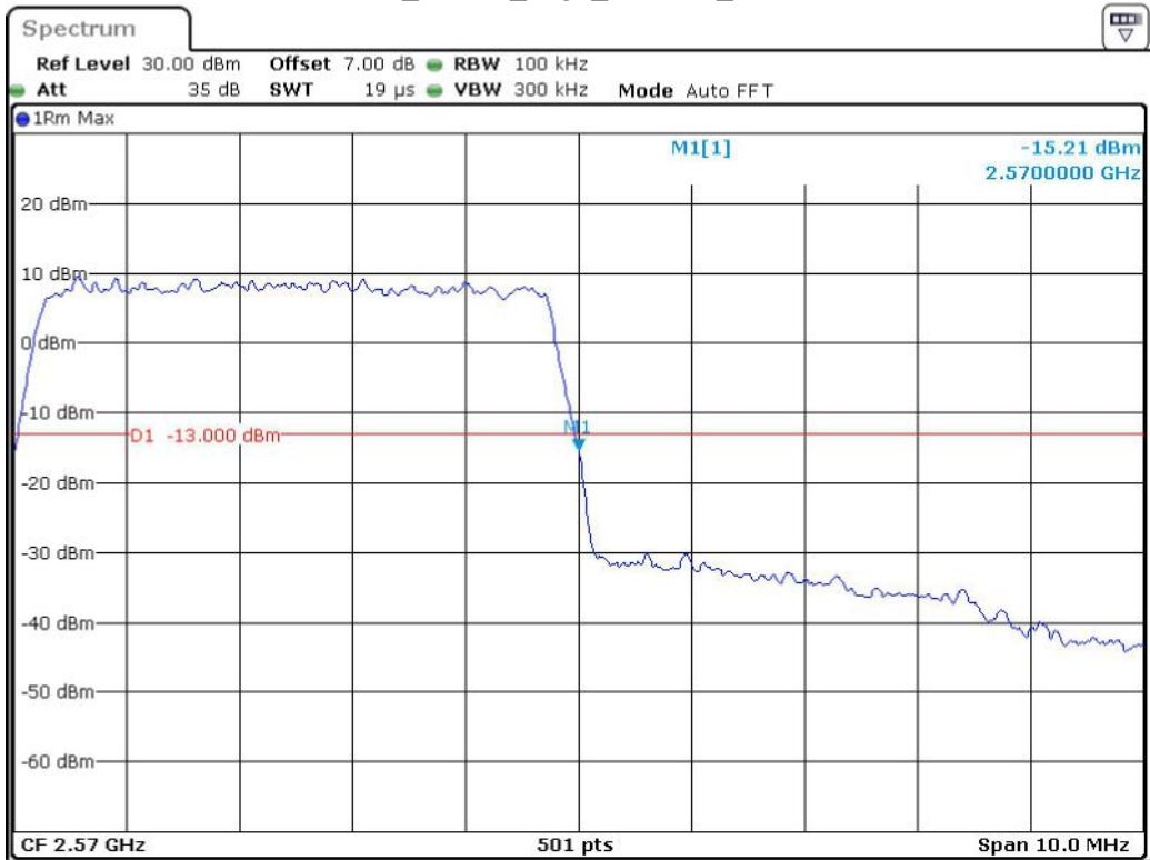
Band 7_5 MHz_High_16QAM_RB25#0
