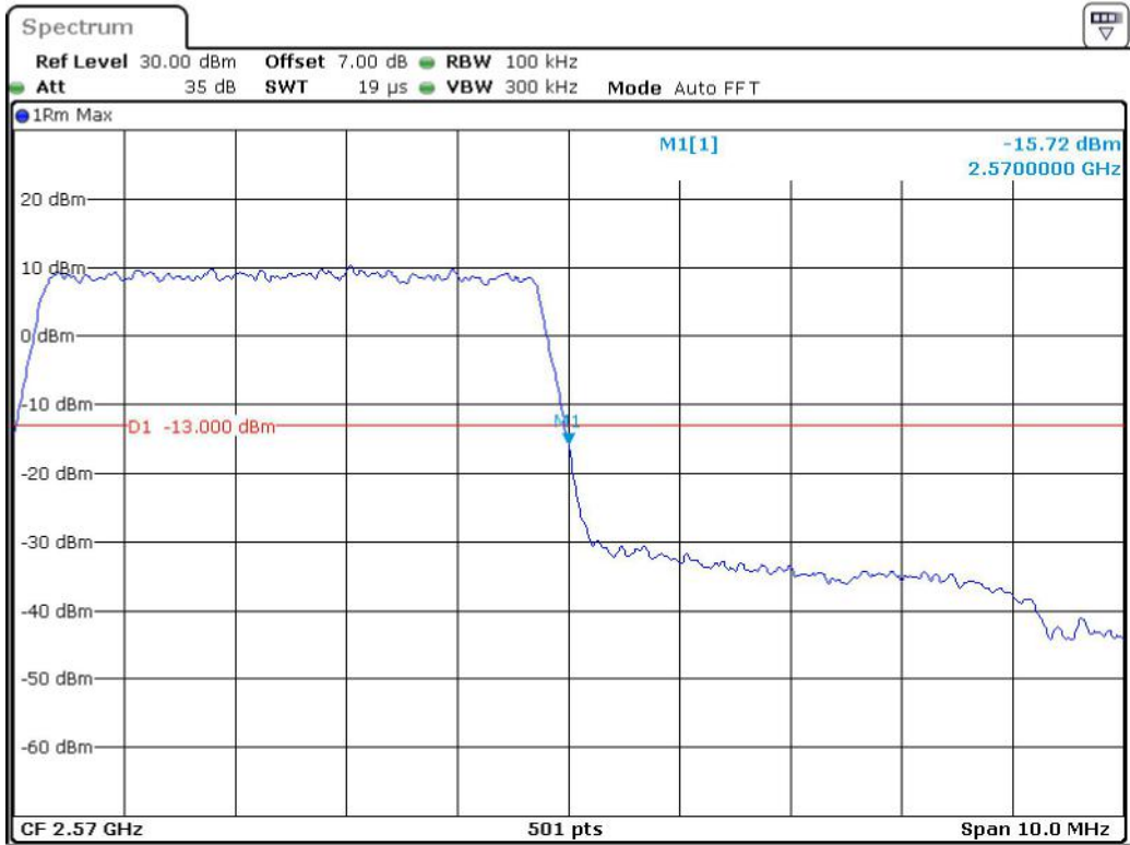
Band 7_5 MHz_High_QPSK_RB25#0
