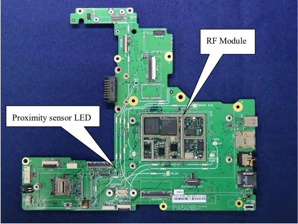
(38) EUT Photo
