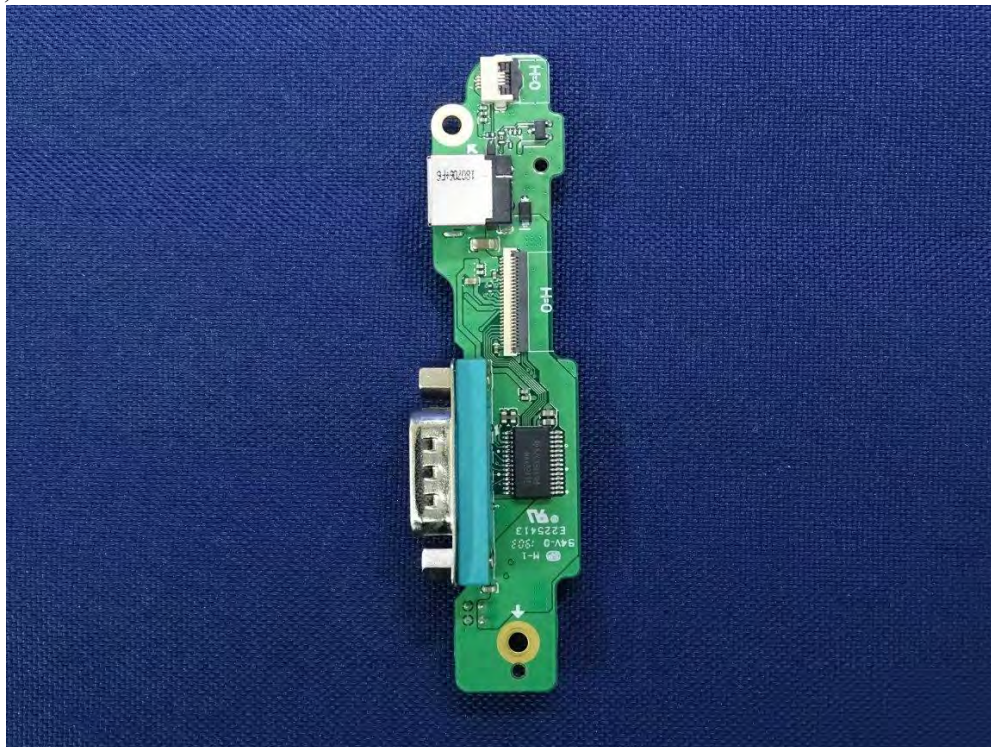
(26) EUT Photo – RS-232
