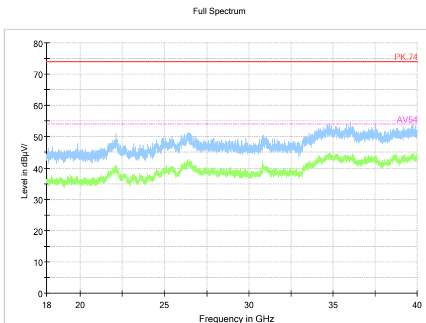
Pic12. Radiated emission (18GHz –40GHz)
