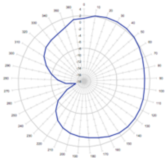
xy plane
