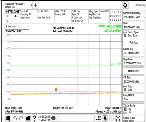
Band4_15MHz_QPSK_20175_75RB#0_3000~20000_3000~2000
