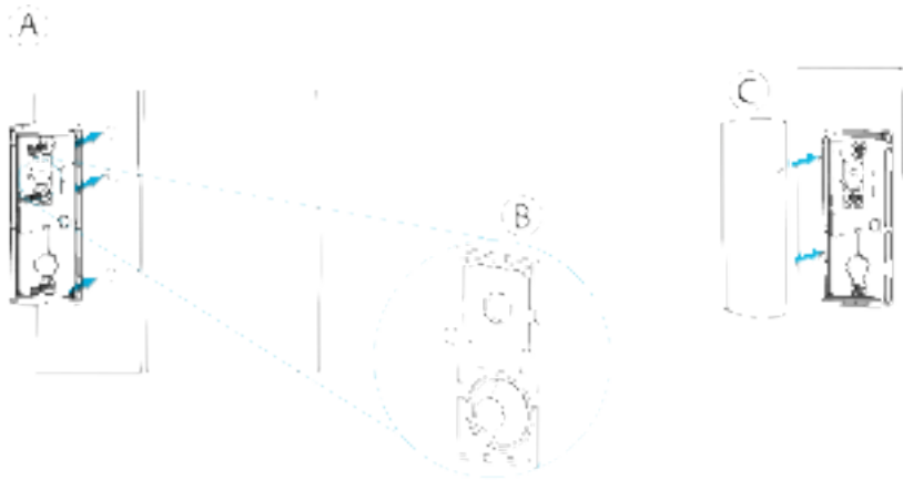
Figure 5: Device screw installation
