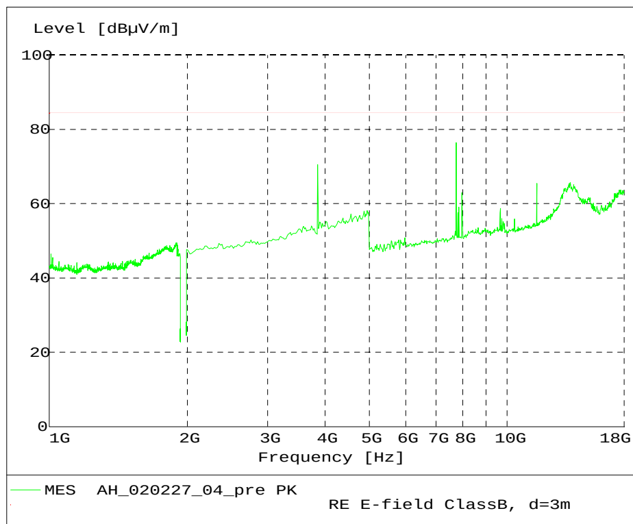
Fig. 41 – Radiated Emission 1 GHz – 18 GHz, 8PSK modulation.
