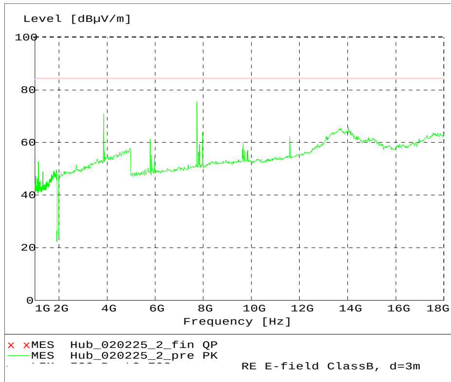
Fig. 40 – Radiated Emission 1 GHz – 18 GHz, GMSK modulation.
