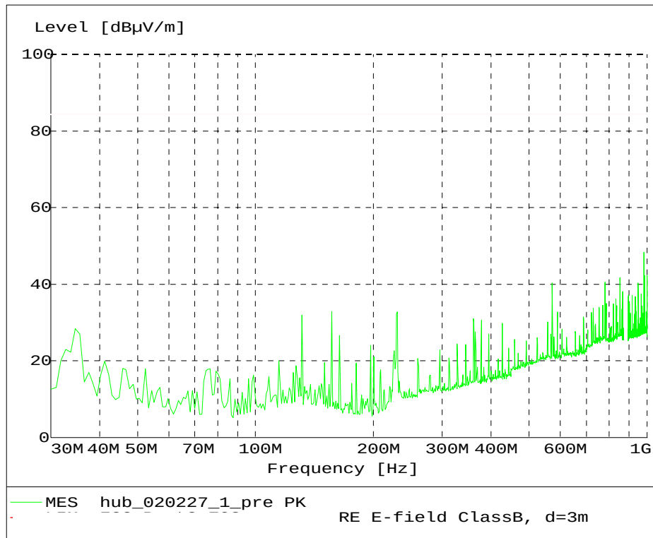
Fig. 38 – Radiated Emission 30 MHz – 1 GHz, GMSK modulation.
