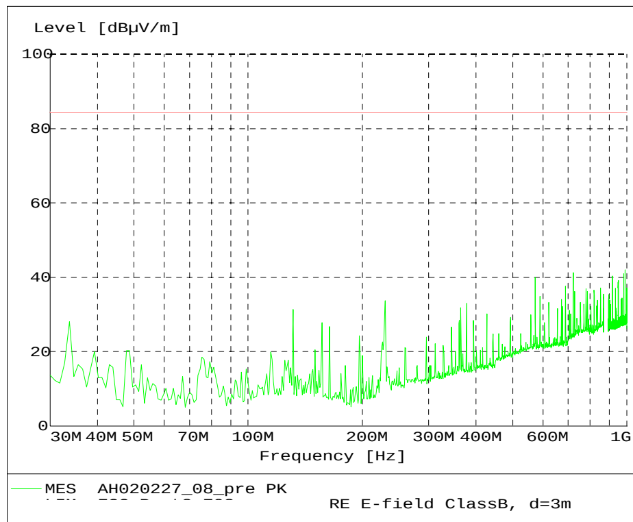
Fig. 39 – Radiated Emission 30 MHz – 1 GHz, 8PSK modulation.
