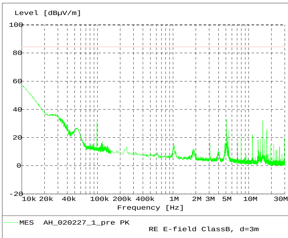
Fig. 37 – Radiated Emission 10 kHz – 30 MHz, 8PSK modulation.
