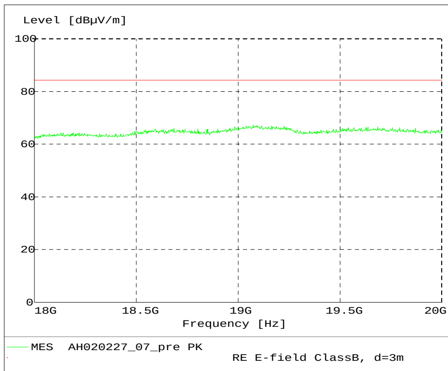
Fig. 43 – Radiated Emission 18 GHz – 20 GHz, 8PSK modulation.
