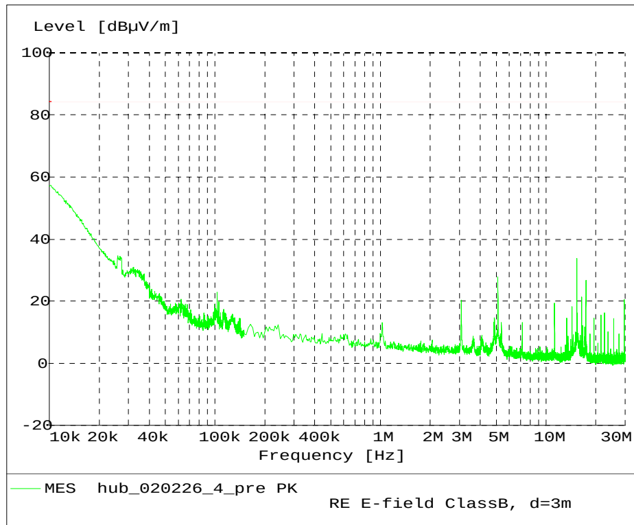
Fig. 36 – Radiated Emission 10 kHz – 30 MHz, GMSK modulation.
