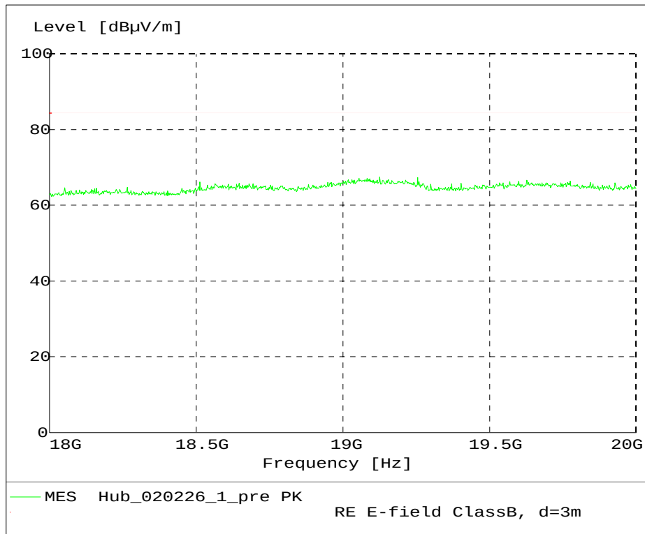
Fig. 42 – Radiated Emission 18 GHz – 20 GHz, GMSK modulation.
