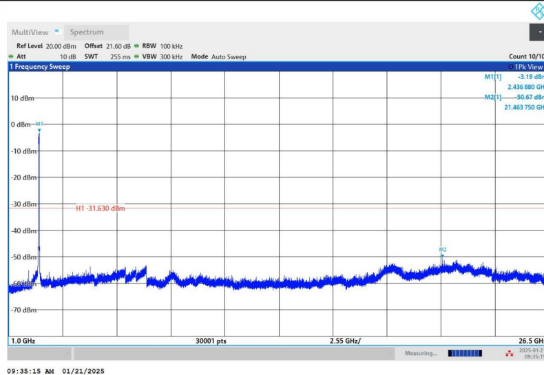
11N40SISO_Ant1_2437_0~Reference
