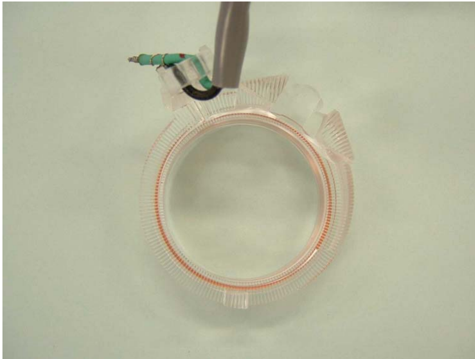
Side A of Key Coil Antenna (Transmitting: 125kHz)
