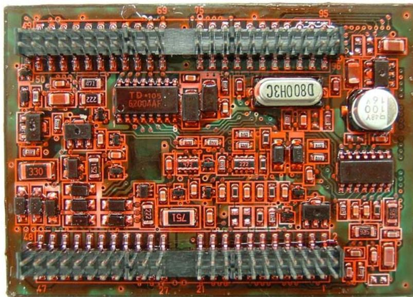
Side B of HIC
