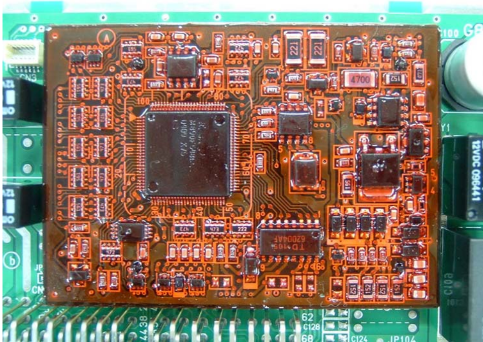
Side A of HIC
