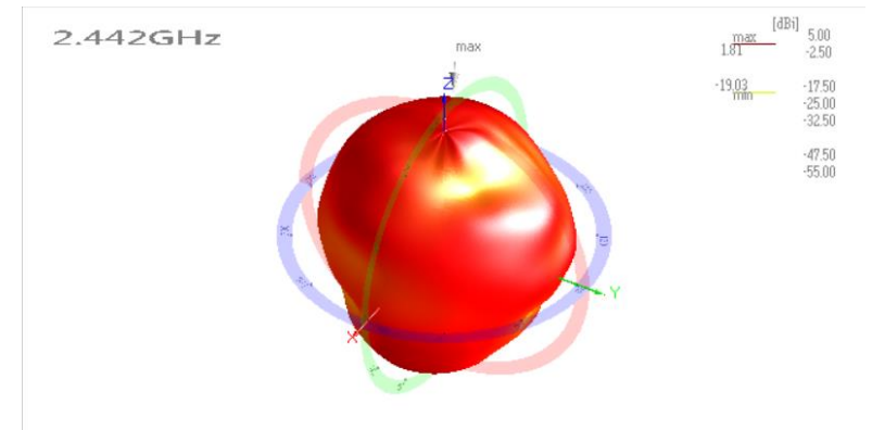
3D radiation pattern @2442MHz
