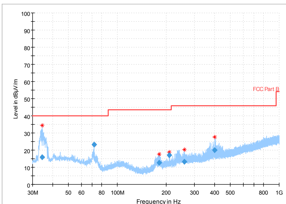
Fig.45 Radiated emission: \pi/4 DQPSK, Ch0, 30MHz~1GHz
