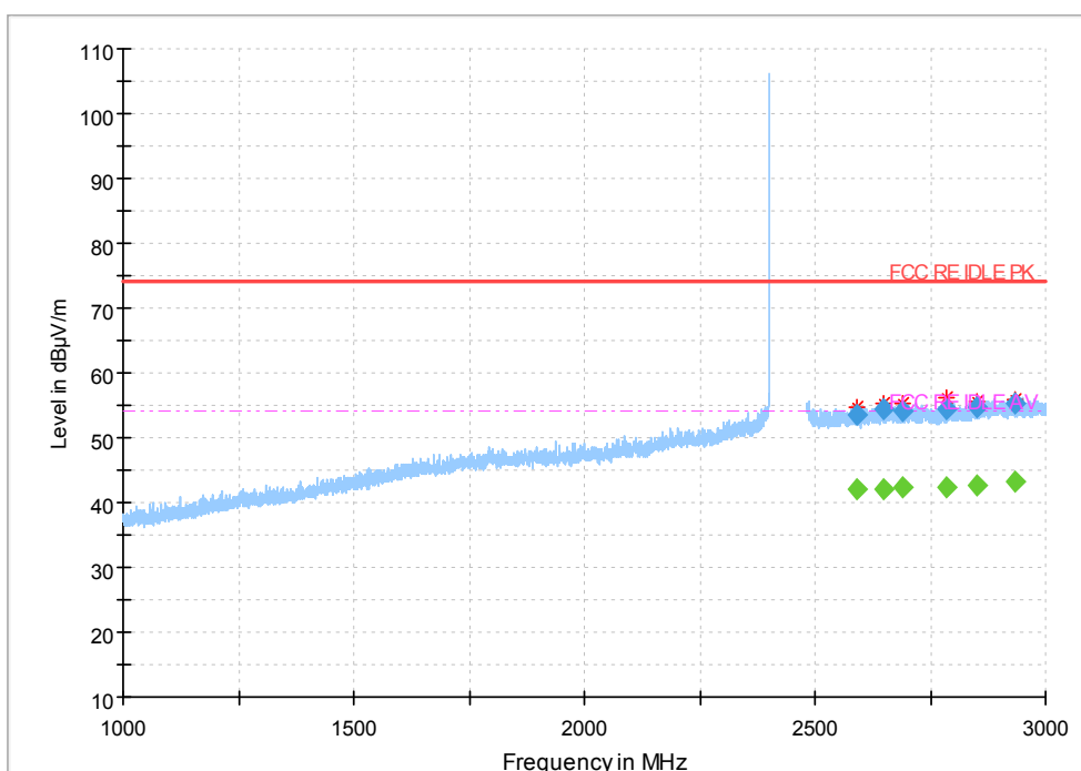
Fig.51 Radiated emission: 8DPSK, Ch0, 1GHz~3GHz
