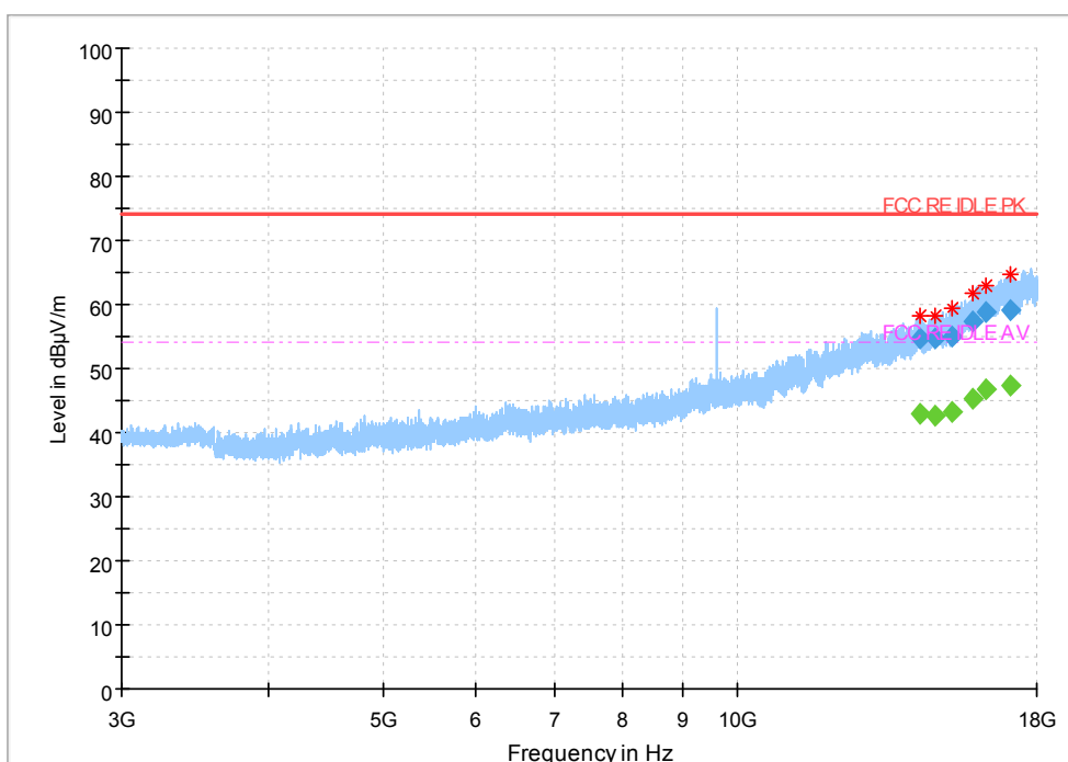
Fig.47 Radiated emission: \pi/4 DQPSK, Ch0, 3GHz~18GHz
