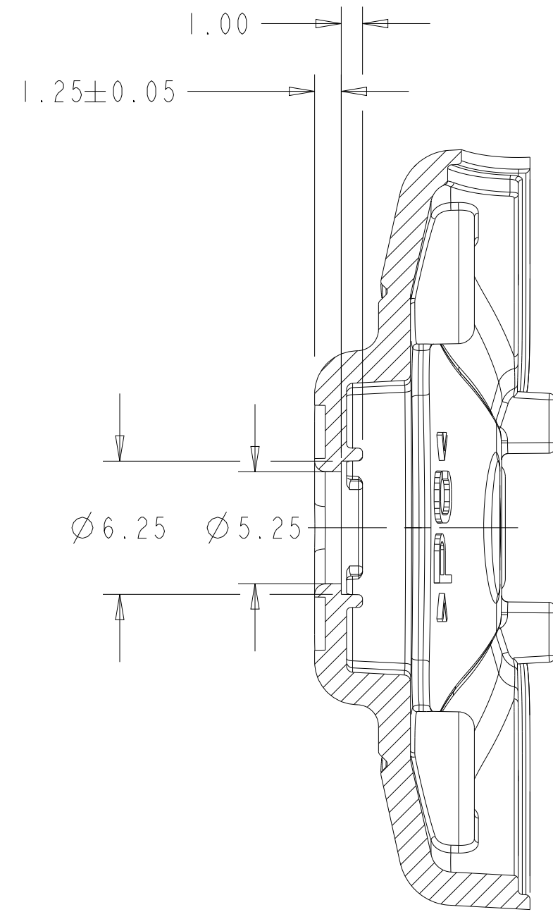
SECTION C-C
