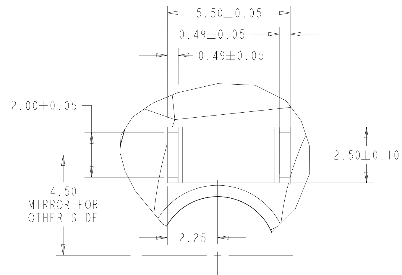
DETAIL Z SCALE 10.000
