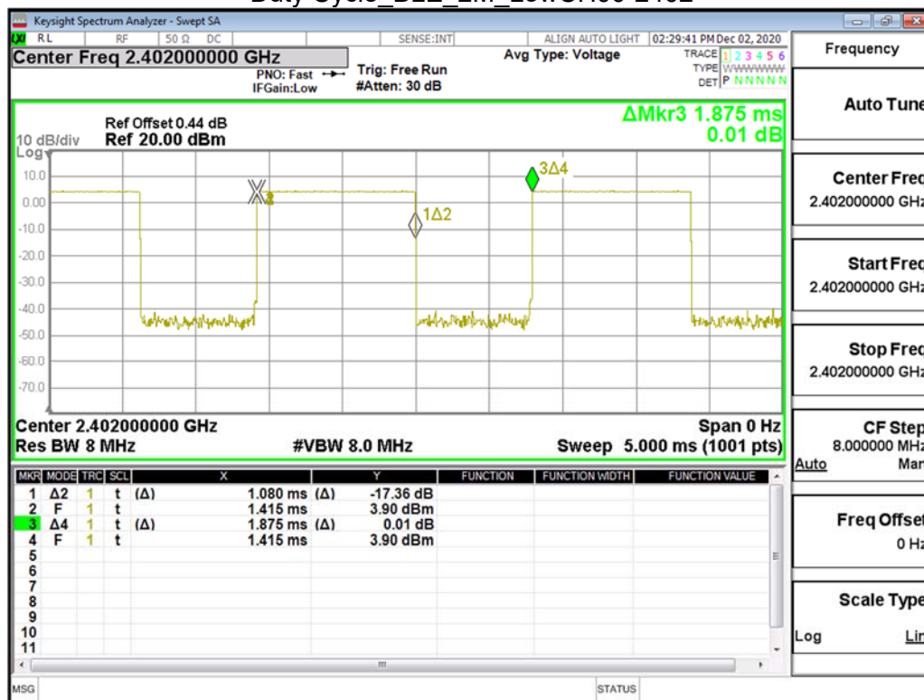
Duty Cycle_BLE_2M_LowCH00-2402
