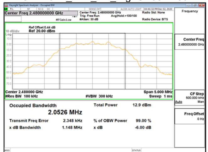
OBW 6dB_BLE_2M_HighCH39-2480
