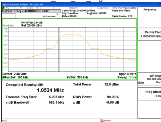
OBW 6dB_BLE_1M_HighCH39-2480
