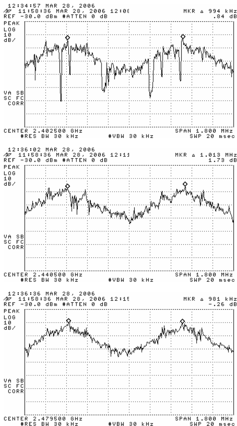
Figure 6.2 Carrier Frequency Separation. (top) Low Channel, (middle) Middle Channel, (bottom) High Channel
