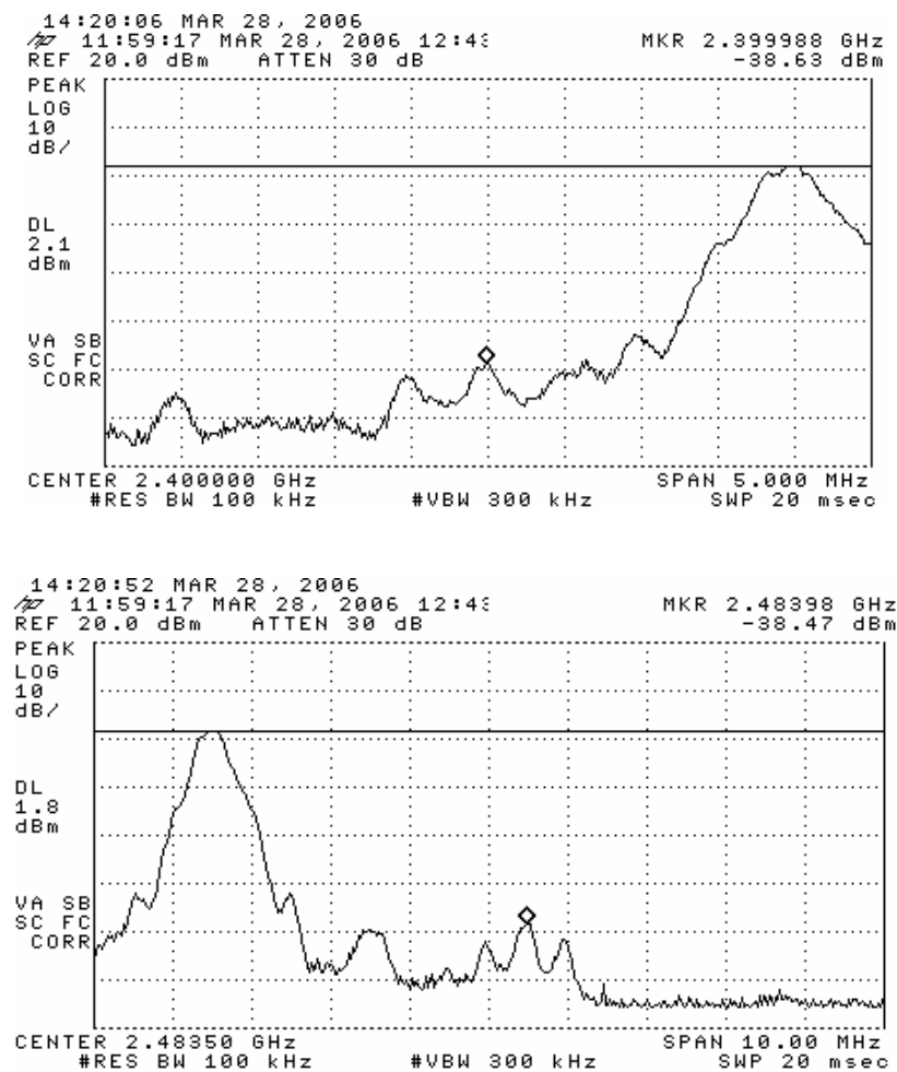
Figure 6.6 Band edge emissions – NOT HOPPING. (top) Low Channel, (bottom) High Channel
