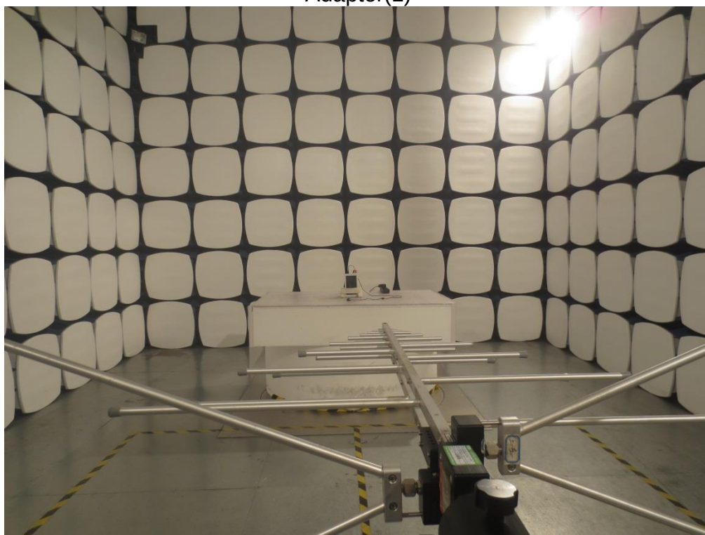
Radiated Spurious Emission(for Below 1GHz) Adapter(1)
