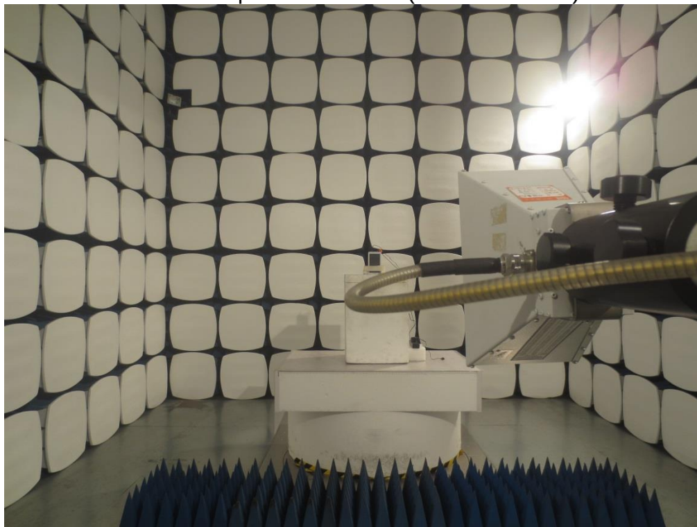
Radiated Spurious Emission(for Above 1GHz)
