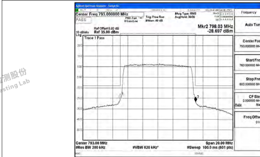
Band14-10MHz-16QAM-23330-50RB#0
