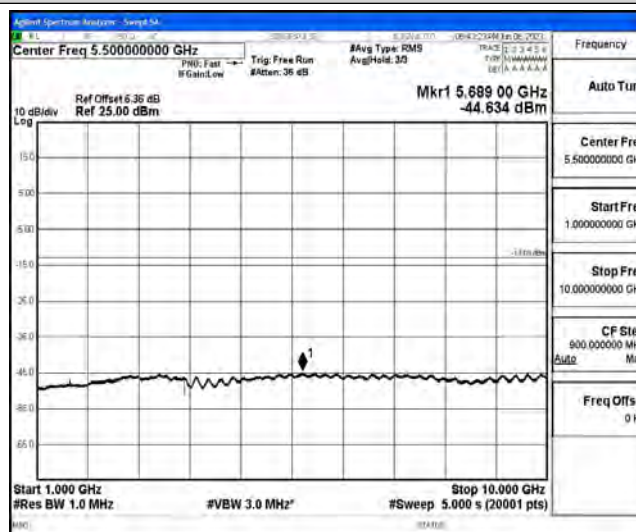
Band14-5MHz-QPSK-23355-1RB#0-Range9:1000~10000MHz
