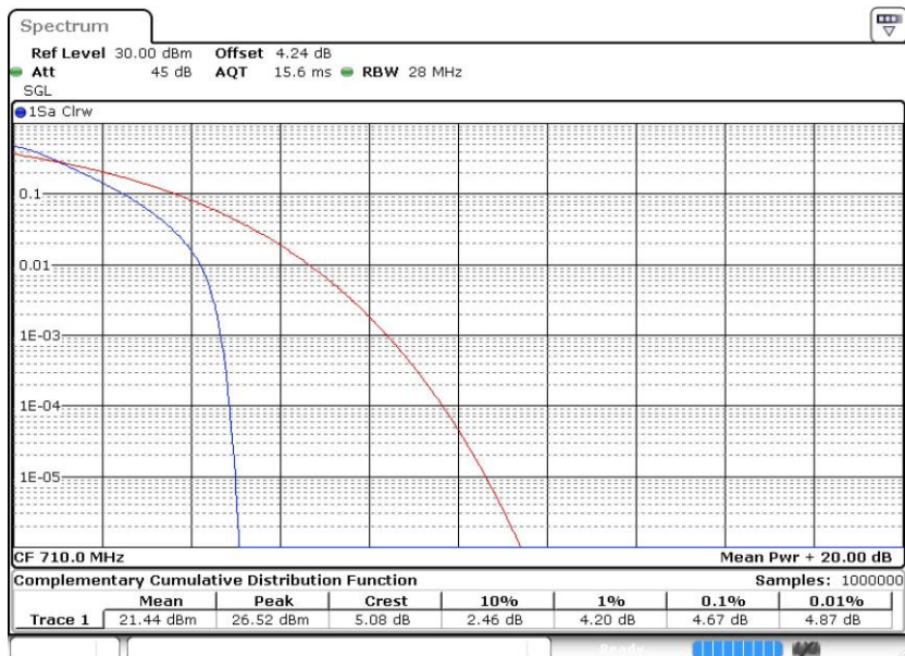
Band17-10MHz-QPSK-23790-50RB#0
