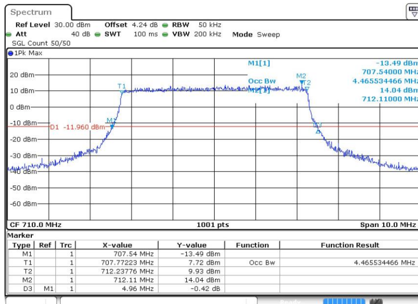
Band17-5MHz-QPSK-23790-25RB#0
