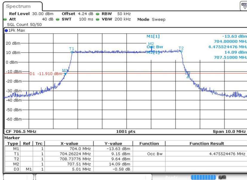
Band17-5MHz-QPSK-23755-25RB#0
