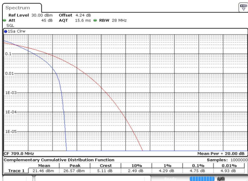
Band17-10MHz-QPSK-23780-50RB#0
