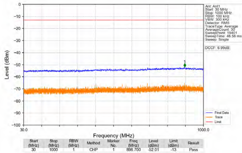
n77d_30kHz_SISO_NTNV_80MHz_CP-OFDM_QPSK_3510MHz_Edge_1RB_Right
