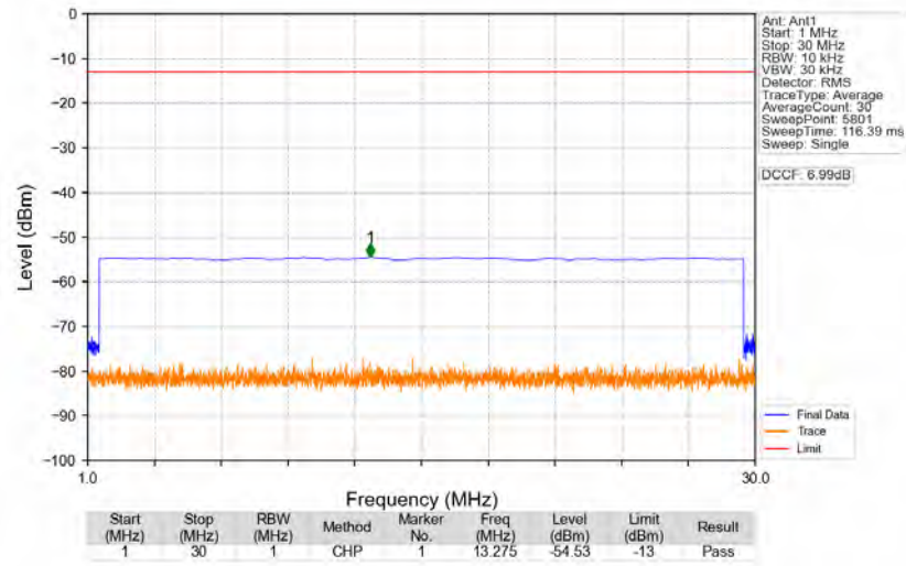
n77d_30kHz_SISO_NTNV_100MHz_CP-OFDM_QPSK_3500.01MHz_Edge_1RB_Right
