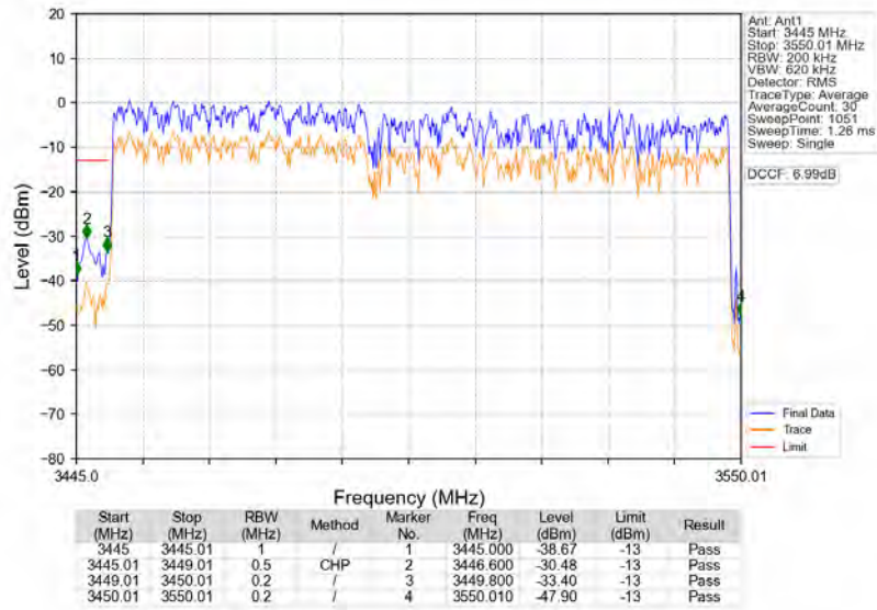
n77d_30kHz_SISO_NTNV_100MHz_DFT-s-OFDM_PI/2_BPSK_3500.01MHz_Outer_Full
