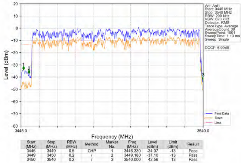
n77d_30kHz_SISO_NTNV_90MHz_DFT-s-OFDM_PI/2_BPSK_3495MHz_Outer_Full
