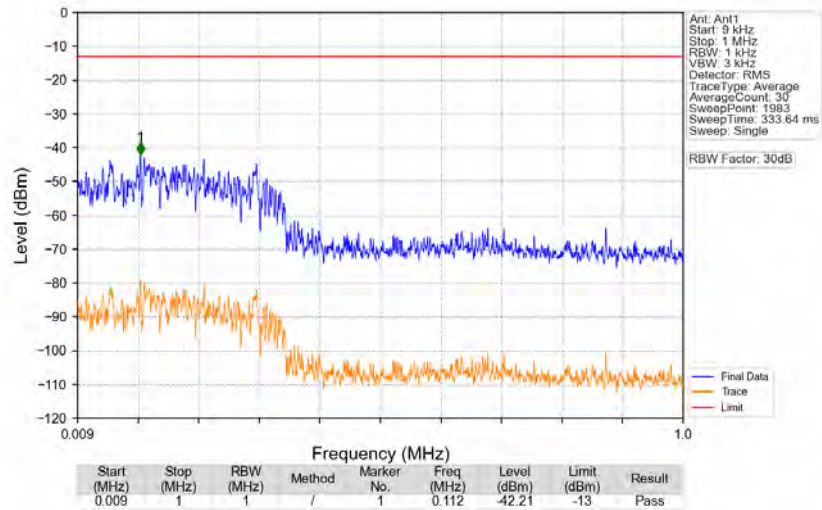
n77d_30kHz_SISO_NTNV_90MHz_DFT-s-OFDM_QPSK_3504.99MHz_Edge_1RB_Right
