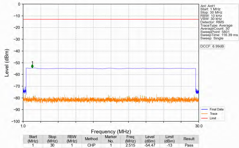
n77d_30kHz_SISO_NTNV_80MHz_CP-OFDM_QPSK_3500.01MHz_Edge_1RB_Left
