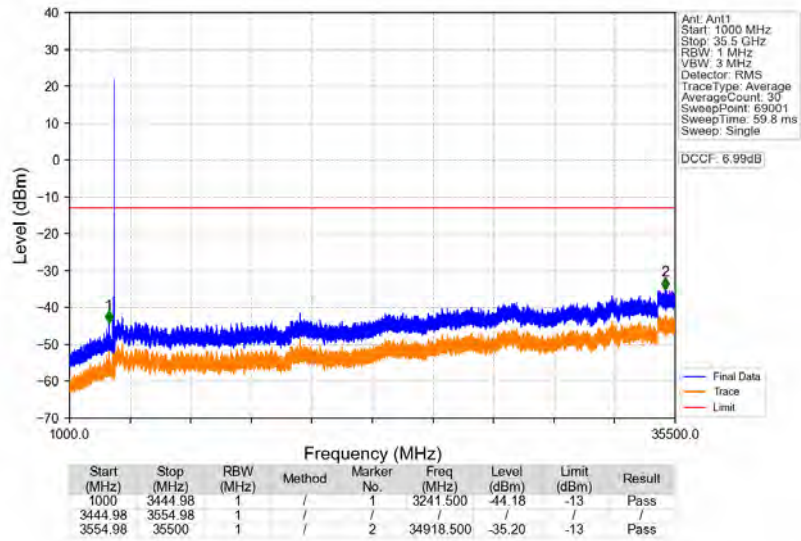
n77d_30kHz_SISO_NTNV_100MHz_DFT-s-OFDM_PI/2_BPSK_3500.01MHz_Edge_1RB_Right
