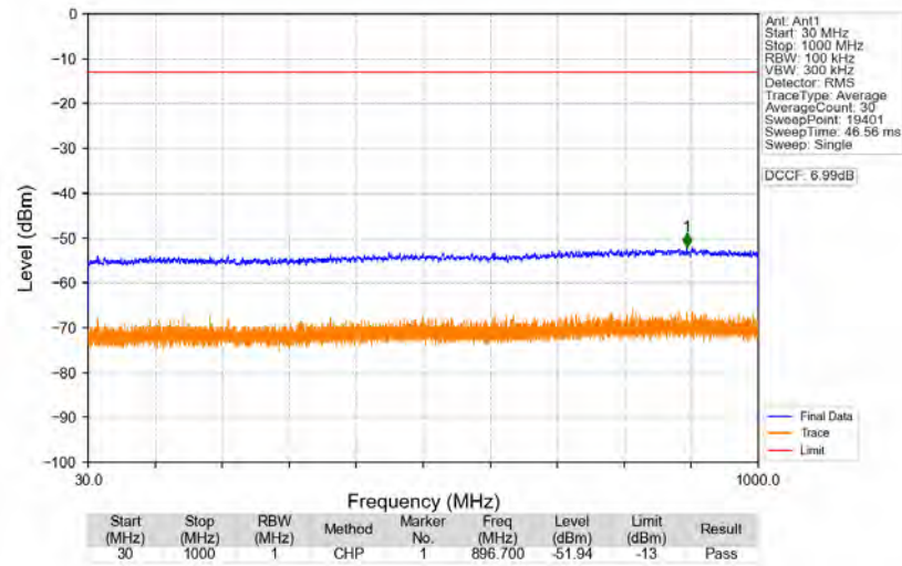
n77d_30kHz_SISO_NTNV_90MHz_CP-OFDM_QPSK_3504.99MHz_Edge_1RB_Right
