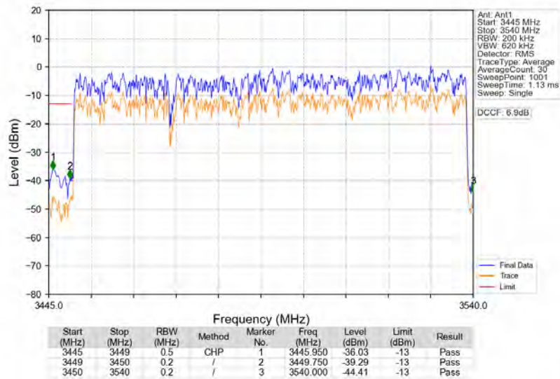
n77d_30kHz_SISO_NTNV_90MHz_DFT-s-OFDM_QPSK_3495MHz_Outer_Full
