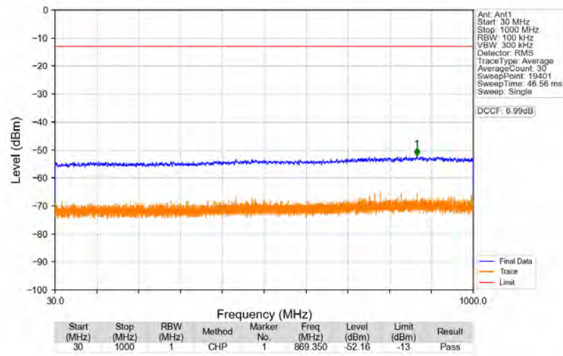
n77d_30kHz_SISO_NTNV_80MHz_CP-OFDM_QPSK_3500.01MHz_Edge_1RB_Left
