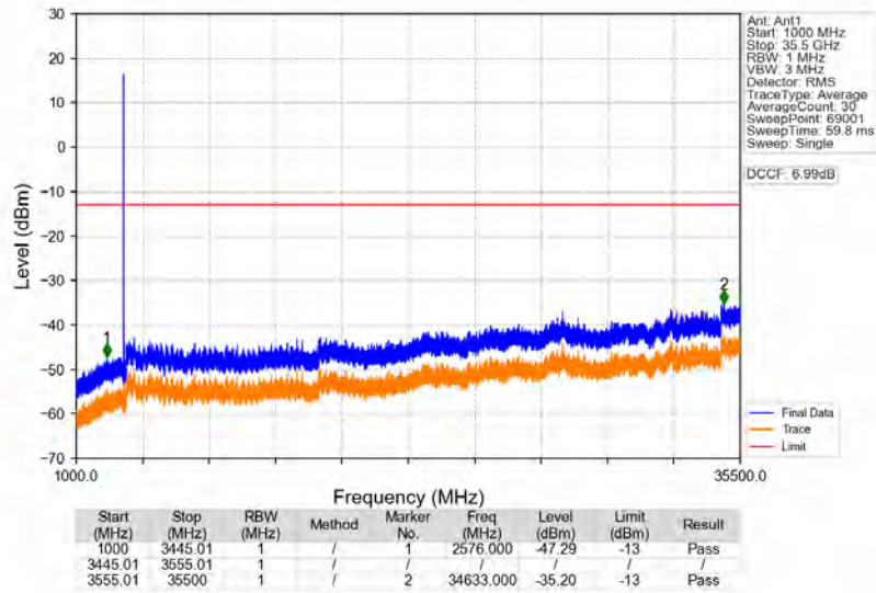
n77d_30kHz_SISO_NTNV_100MHz_CP-OFDM_QPSK_3500.01MHz_Edge_1RB_Left
