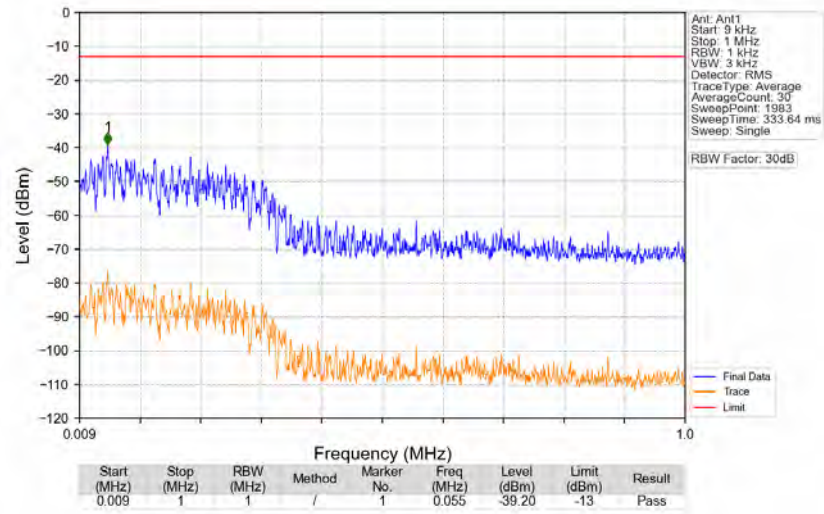
n77d_30kHz_SISO_NTNV_80MHz_CP-OFDM_QPSK_3500.01MHz_Edge_1RB_Left
