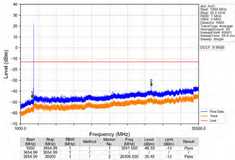
n77d_30kHz_SISO_NTNV_90MHz_CP-OFDM_QPSK_3504.99MHz_Edge_1RB_Right
