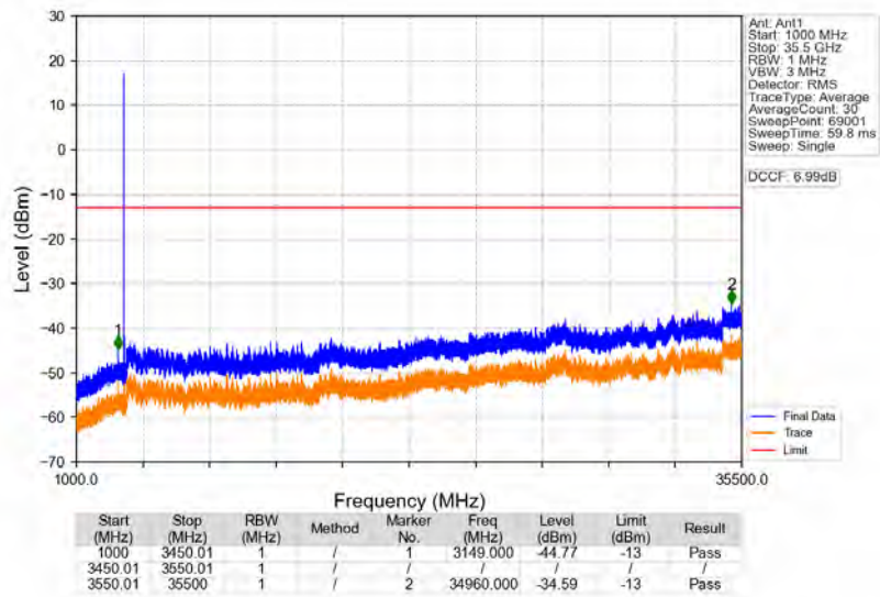
n77d_30kHz_SISO_NTNV_90MHz_CP-OFDM_QPSK_3500.01MHz_Edge_1RB_Left
