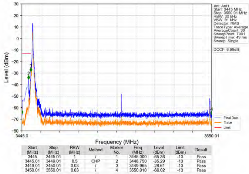
n77d_30kHz_SISO_NTNV_100MHz_DFT-s-OFDM_QPSK_3500.01MHz_Edge_1RB_Left
