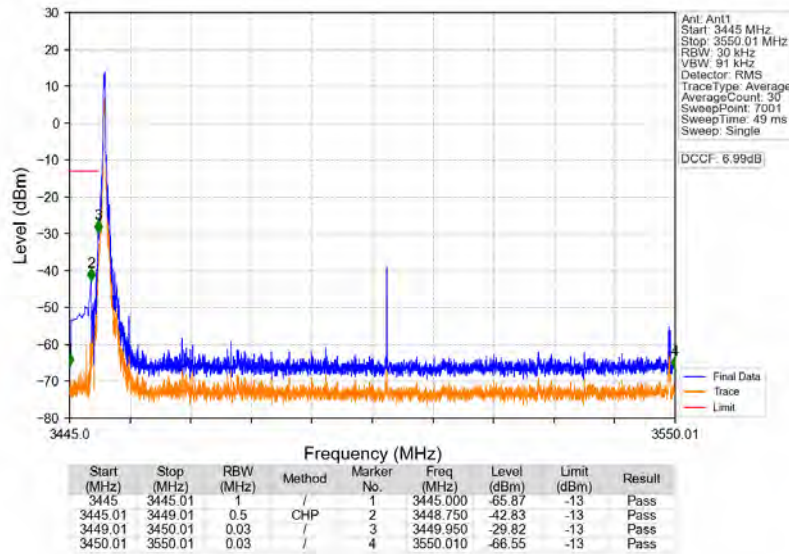
n77d_30kHz_SISO_NTNV_100MHz_CP-OFDM_QPSK_3500.01MHz_Edge_1RB_Left
