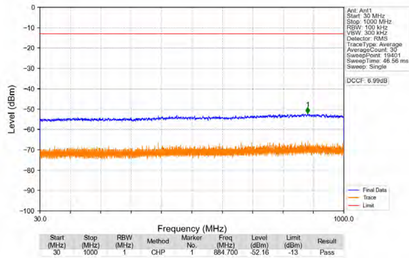
n77d_30kHz_SISO_NTNV_90MHz_CP-OFDM_QPSK_3500.01MHz_Edge_1RB_Left
