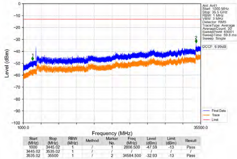
n77d_30kHz_SISO_NTNV_80MHz_CP-OFDM_QPSK_3490.02MHz_Edge_1RB_Left
