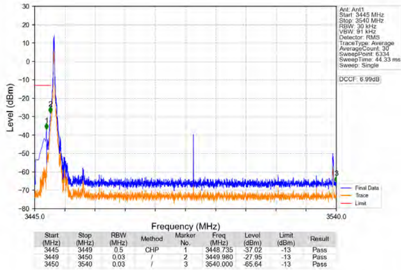
n77d_30kHz_SISO_NTNV_90MHz_DFT-s-OFDM_QPSK_3495MHz_Edge_1RB_Left
