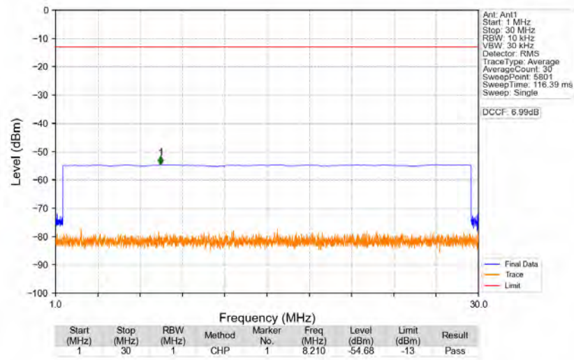
n77d_30kHz_SISO_NTNV_80MHz_CP-OFDM_QPSK_3510MHz_Edge_1RB_Right
