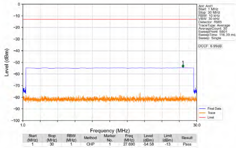
n77d_30kHz_SISO_NTNV_90MHz_CP-OFDM_QPSK_3495MHz_Edge_1RB_Left
