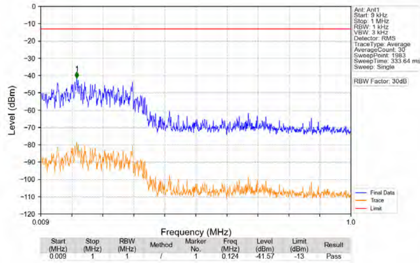
n77d_30kHz_SISO_NTNV_100MHz_DFT-s-OFDM_QPSK_3500.01MHz_Edge_1RB_Left
