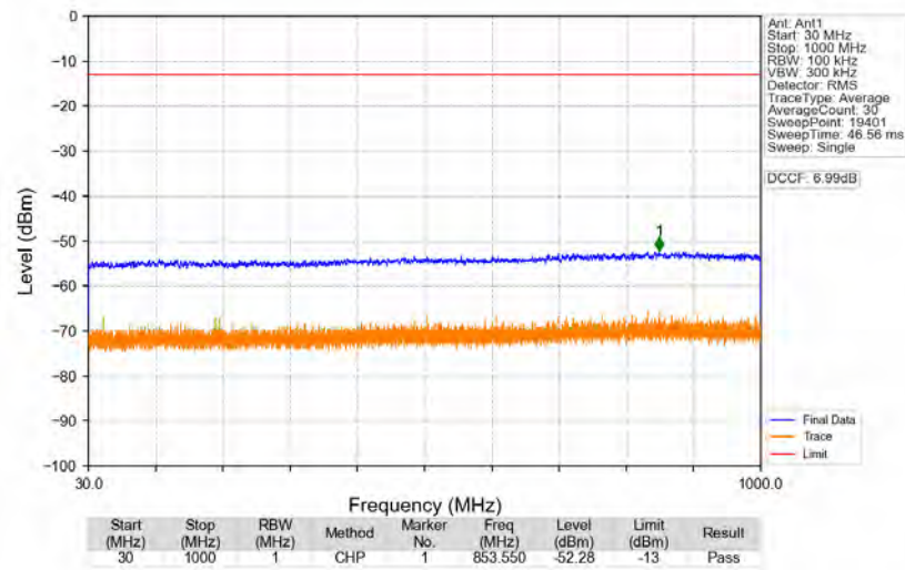
n77d_30kHz_SISO_NTNV_90MHz_CP-OFDM_QPSK_3495MHz_Edge_1RB_Left
