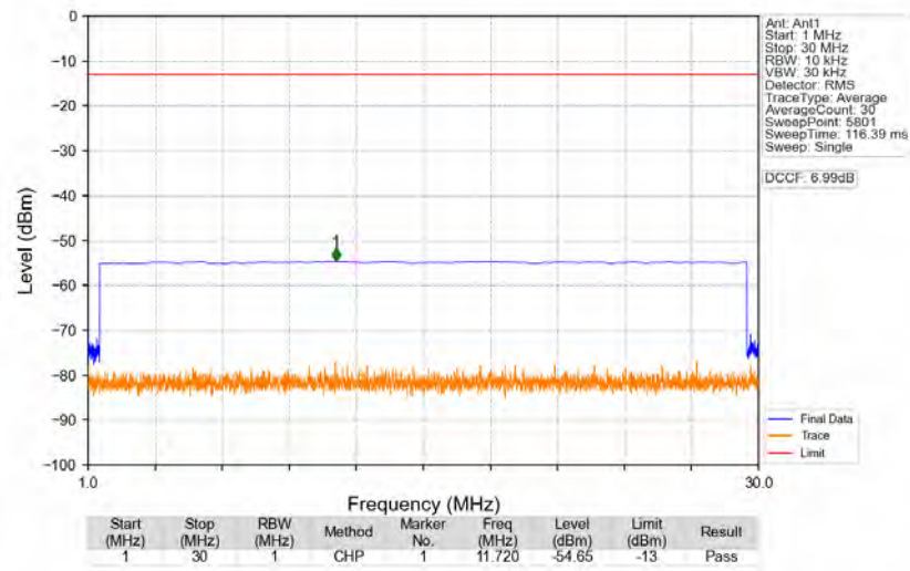
n77d_30kHz_SISO_NTNV_90MHz_DFT-s-OFDM_QPSK_3504.99MHz_Edge_1RB_Right
