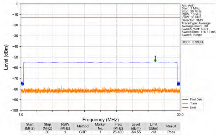
n77d_30kHz_SISO_NTNV_90MHz_DFT-s-OFDM_QPSK_3495MHz_Edge_1RB_Left
