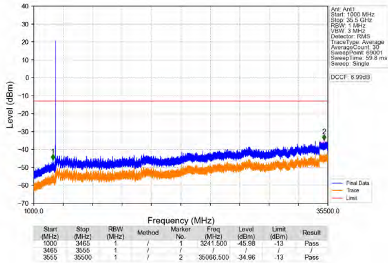
n77d_30kHz_SISO_NTNV_80MHz_CP-OFDM_QPSK_3510MHz_Edge_1RB_Right
