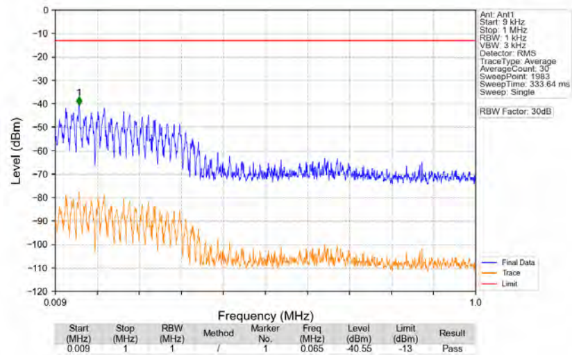
n77d_30kHz_SISO_NTNV_80MHz_CP-OFDM_QPSK_3510MHz_Edge_1RB_Right
