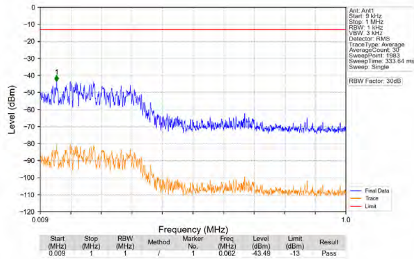
n77d_30kHz_SISO_NTNV_100MHz_DFT-s-OFDM_QPSK_3500.01MHz_Edge_1RB_Right
