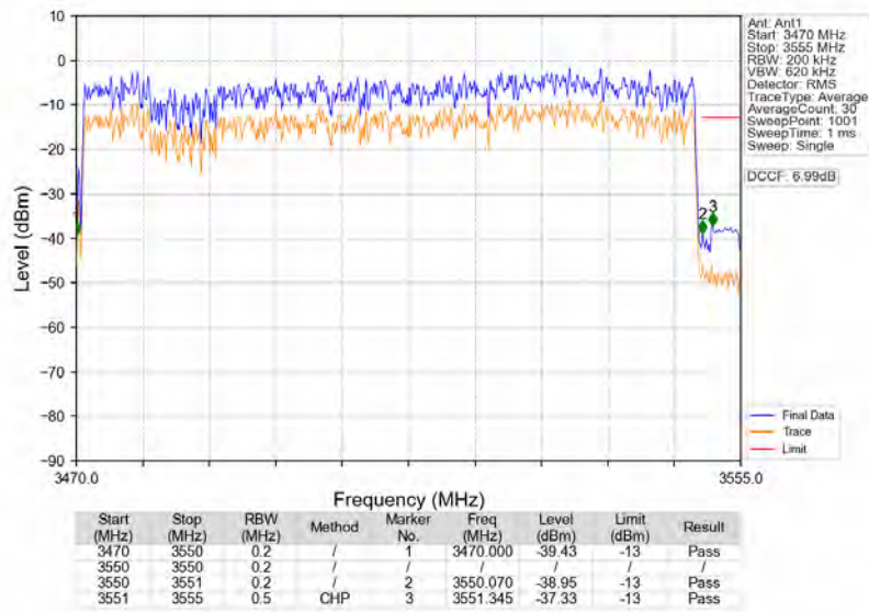
n77d_30kHz_SISO_NTNV_80MHz_CP-OFDM_QPSK_3510MHz_Outer_Full
