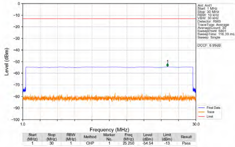
n77d_30kHz_SISO_NTNV_90MHz_CP-OFDM_QPSK_3504.99MHz_Edge_1RB_Right
