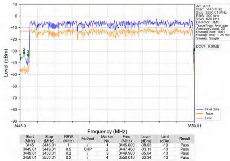
n77d_30kHz_SISO_NTNV_100MHz_CP-OFDM_QPSK_3500.01MHz_Outer_Full
