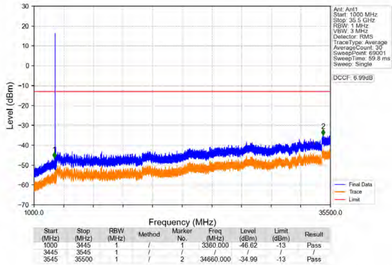
n77d_30kHz_SISO_NTNV_90MHz_DFT-s-OFDM_PI/2_BPSK_3495MHz_Edge_1RB_Left
