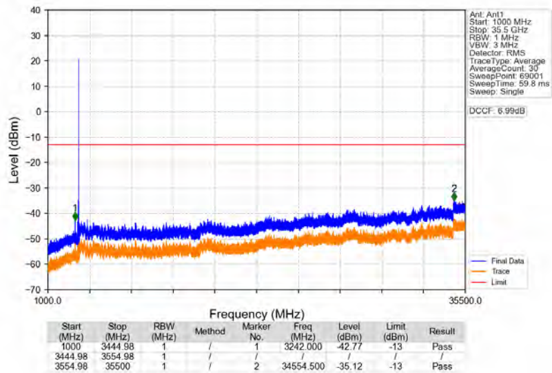
n77d_30kHz_SISO_NTNV_100MHz_DFT-s-OFDM_QPSK_3500.01MHz_Edge_1RB_Right
