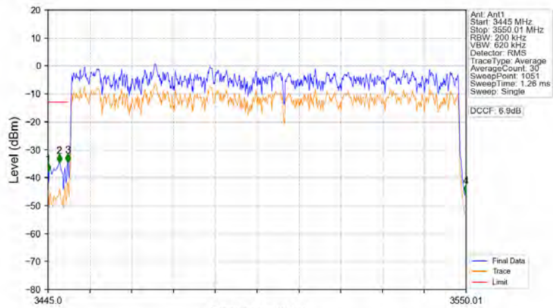
n77d_30kHz_SISO_NTNV_100MHz_DFT-s-OFDM_QPSK_3500.01MHz_Outer_Full
