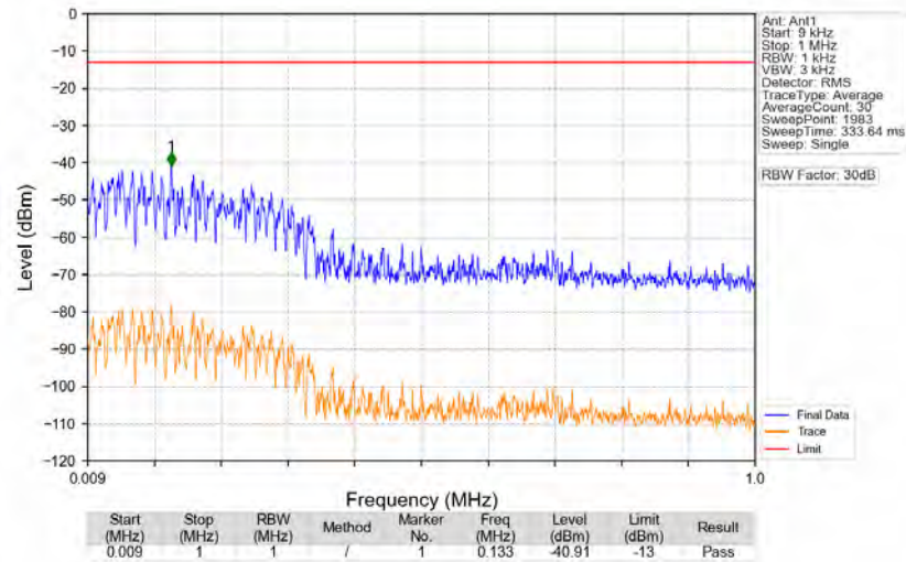
n77d_30kHz_SISO_NTNV_100MHz_CP-OFDM_QPSK_3500.01MHz_Edge_1RB_Left
