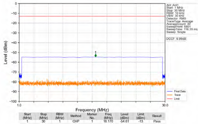
n77d_30kHz_SISO_NTNV_100MHz_CP-OFDM_QPSK_3500.01MHz_Edge_1RB_Left
