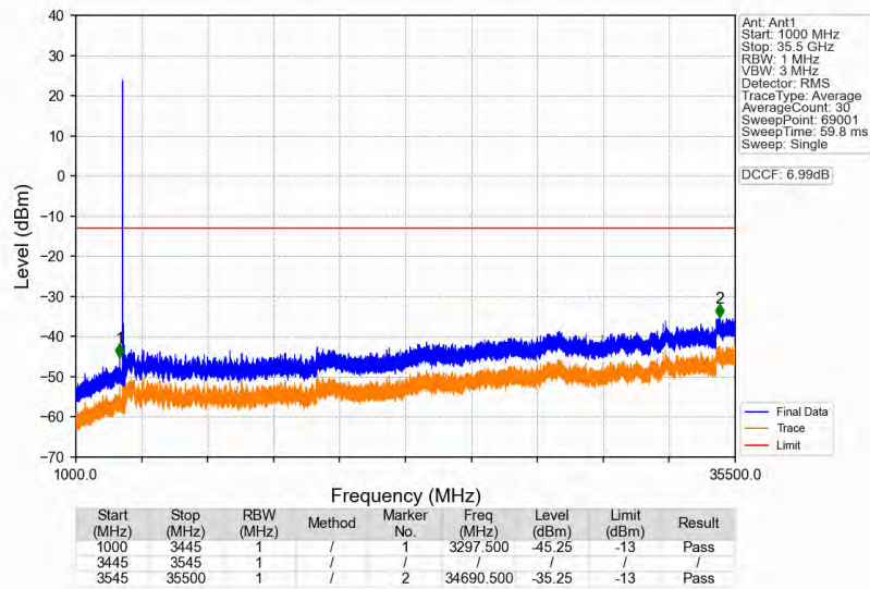
n77d_30kHz_SISO_NTNV_90MHz_DFT-s-OFDM_QPSK_3495MHz_Edge_1RB_Left
