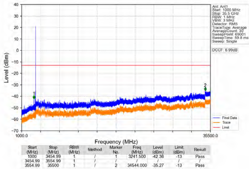
n77d_30kHz_SISO_NTNV_90MHz_DFT-s-OFDM_QPSK_3504.99MHz_Edge_1RB_Right
