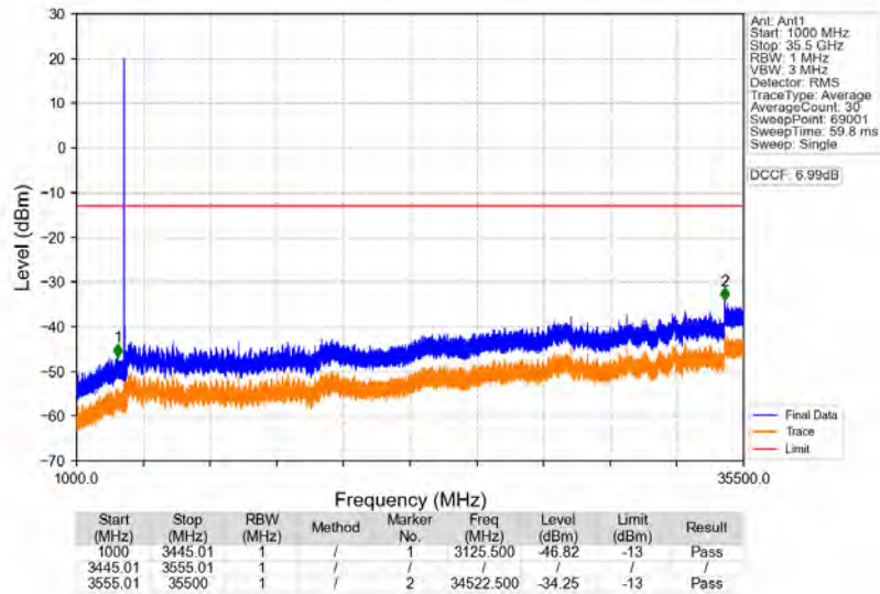
n77d_30kHz_SISO_NTNV_100MHz_DFT-s-OFDM_PI/2_BPSK_3500.01MHz_Edge_1RB_Left
