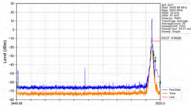
n77d_30kHz_SISO_NTNV_100MHz_DFT-s-OFDM_QPSK_3500.01MHz_Edge_1RB_Right
