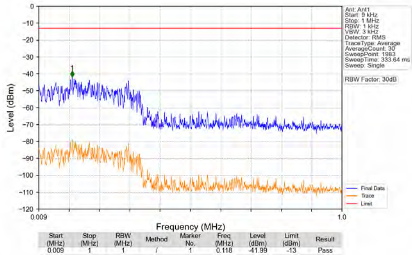
n77d_30kHz_SISO_NTNV_90MHz_DFT-s-OFDM_QPSK_3495MHz_Edge_1RB_Left
