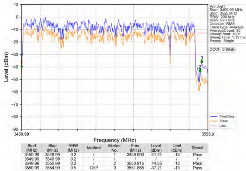
n77d_30kHz_SISO_NTNV_90MHz_DFT-s-OFDM_QPSK_3504.99MHz_Outer_Full
