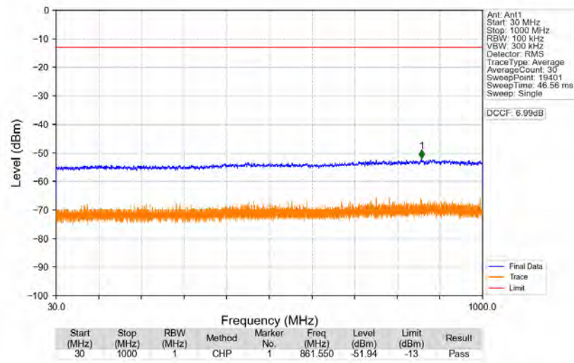
n77d_30kHz_SISO_NTNV_100MHz_DFT-s-OFDM_QPSK_3500.01MHz_Edge_1RB_Right
