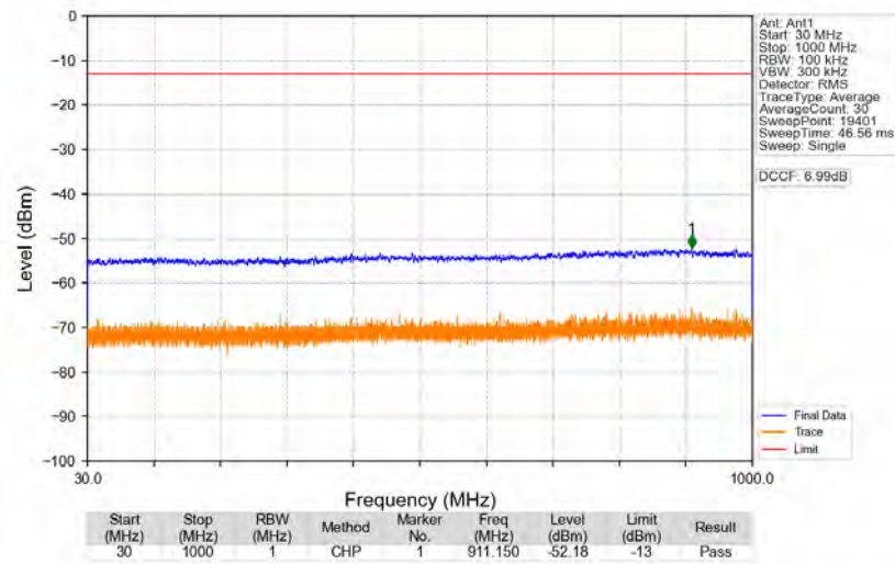
n77d_30kHz_SISO_NTNV_100MHz_DFT-s-OFDM_QPSK_3500.01MHz_Edge_1RB_Left
