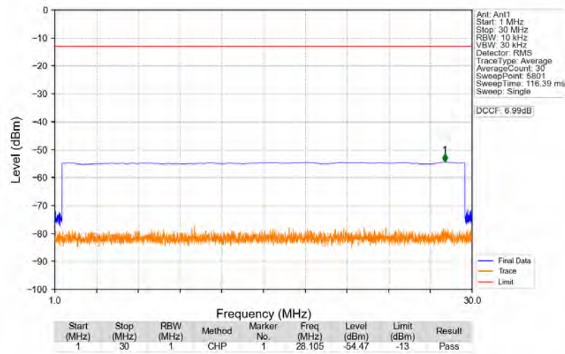
n77d_30kHz_SISO_NTNV_90MHz_DFT-s-OFDM_QPSK_3500.01MHz_Edge_1RB_Left
