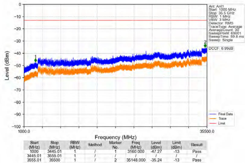
n77d_30kHz_SISO_NTNV_100MHz_DFT-s-OFDM_QPSK_3500.01MHz_Edge_1RB_Left
