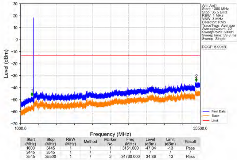
n77d_30kHz_SISO_NTNV_90MHz_CP-OFDM_QPSK_3495MHz_Edge_1RB_Left
