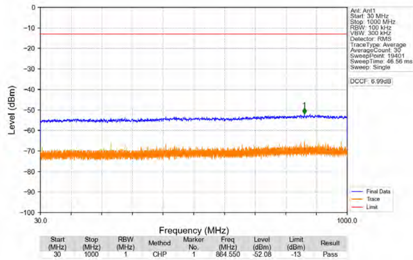
n77d_30kHz_SISO_NTNV_90MHz_DFT-s-OFDM_QPSK_3504.99MHz_Edge_1RB_Right
