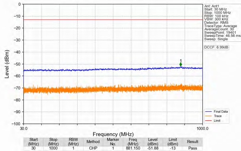
n77d_30kHz_SISO_NTNV_100MHz_CP-OFDM_QPSK_3500.01MHz_Edge_1RB_Left
