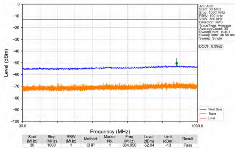
n77d_30kHz_SISO_NTNV_90MHz_DFT-s-OFDM_QPSK_3500.01MHz_Edge_1RB_Left
