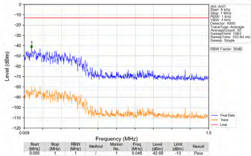
n77d_30kHz_SISO_NTNV_90MHz_CP-OFDM_QPSK_3504.99MHz_Edge_1RB_Right
