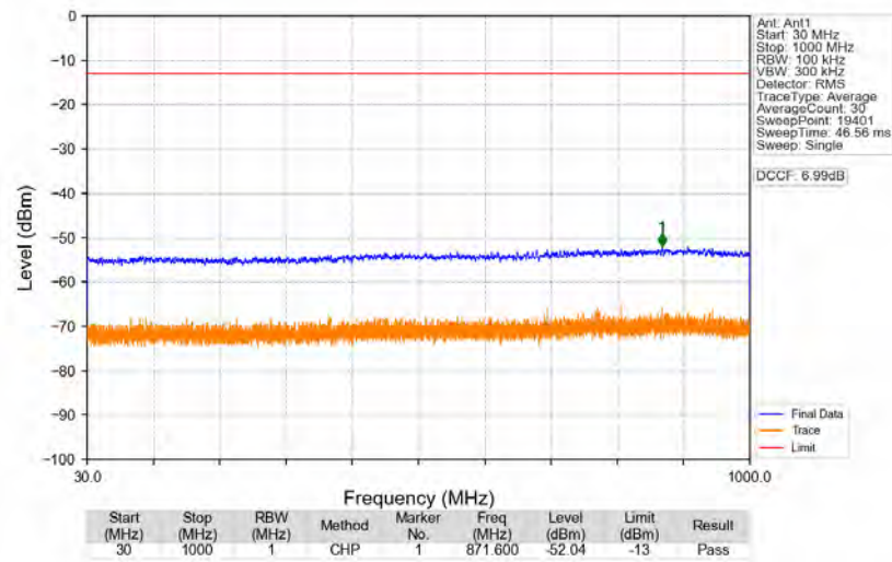
n77d_30kHz_SISO_NTNV_90MHz_DFT-s-OFDM_QPSK_3495MHz_Edge_1RB_Left
