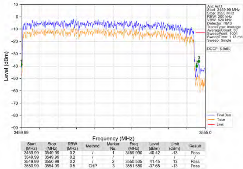
n77d_30kHz_SISO_NTNV_90MHz_CP-OFDM_QPSK_3504.99MHz_Outer_Full
