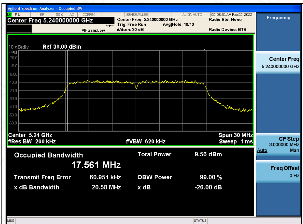
Test_Graph_802.11ac20_ANT1_5240_MCS9_OBW
