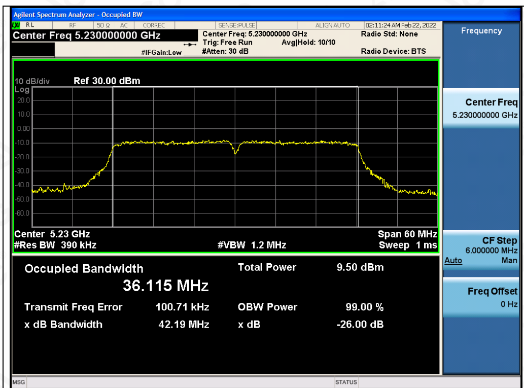
Test_Graph_802.11ac40_ANT1_5230_MCS9_OBW
