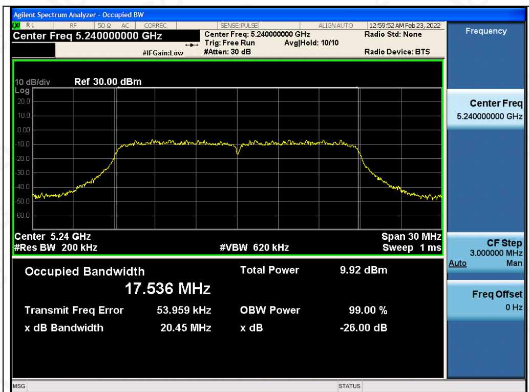
Test_Graph_802.11ac20_ANT2_5240_MCS9_OBW
