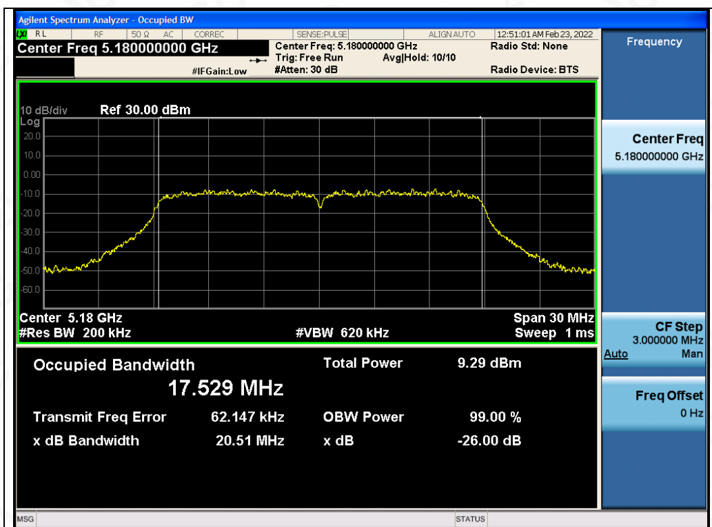
Test_Graph_802.11ac20_ANT2_5180_MCS0_OBW
