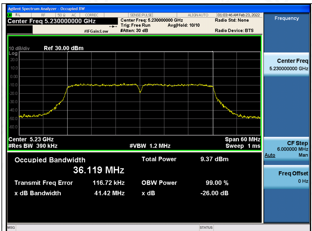
Test_Graph_802.11ac40_ANT2_5230_MCS9_OBW
