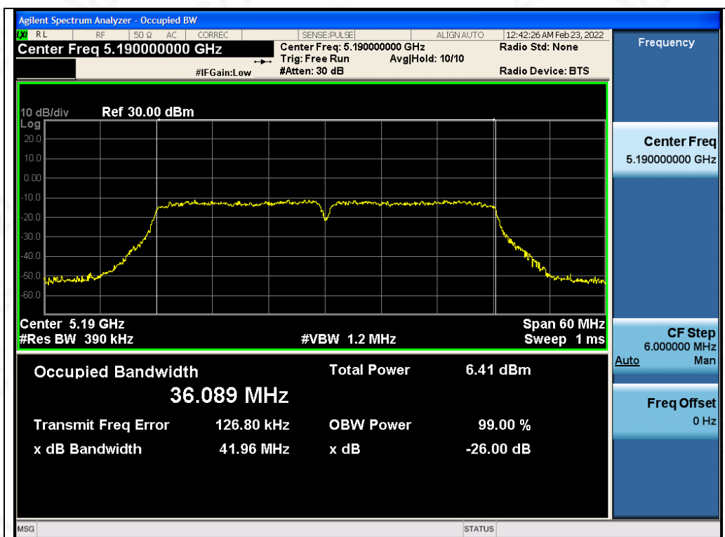
Test_Graph_802.11n40_ANT2_5190_MCS0_OBW
