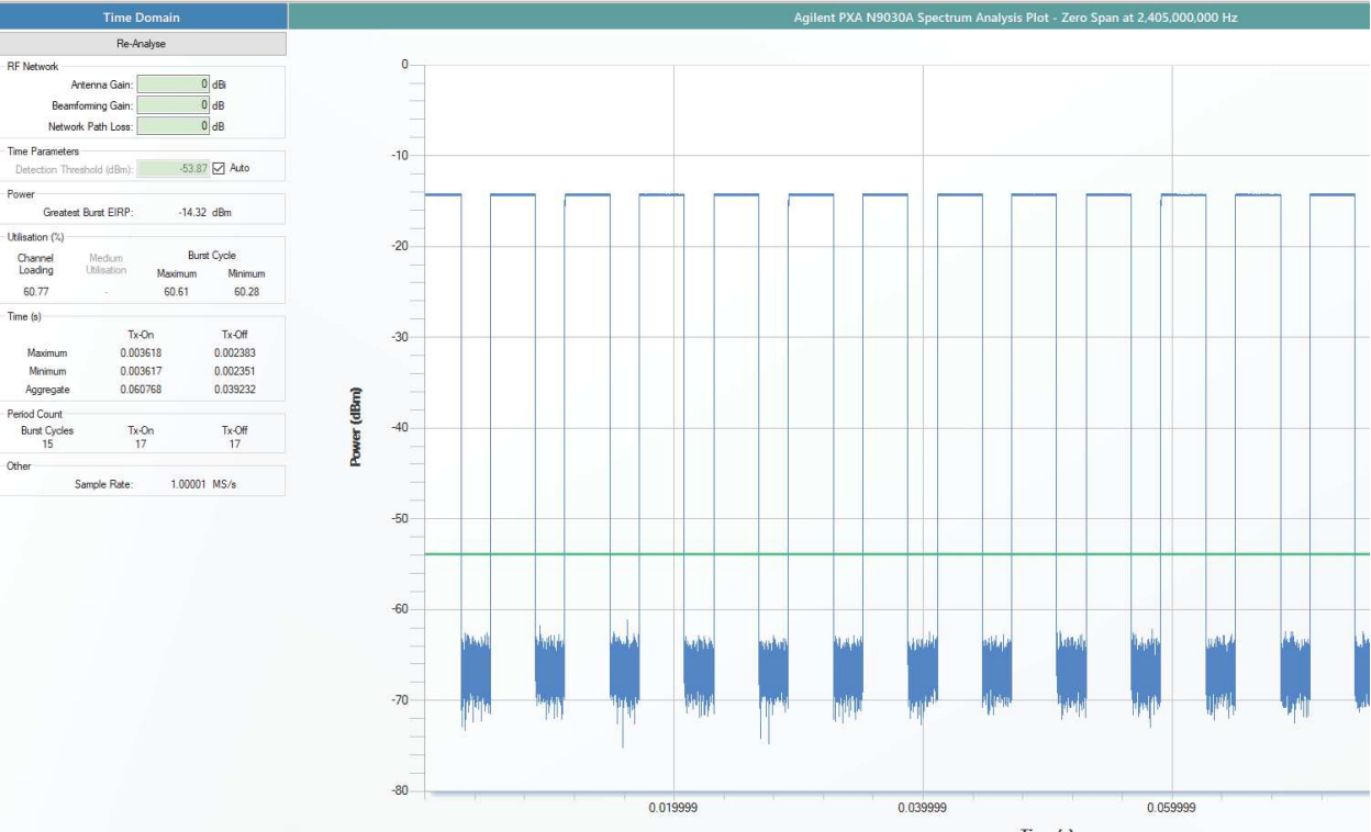
Figure 2 - Thread ePA - Frequency of 2405 MHz (60.61% Duty Cycle)
