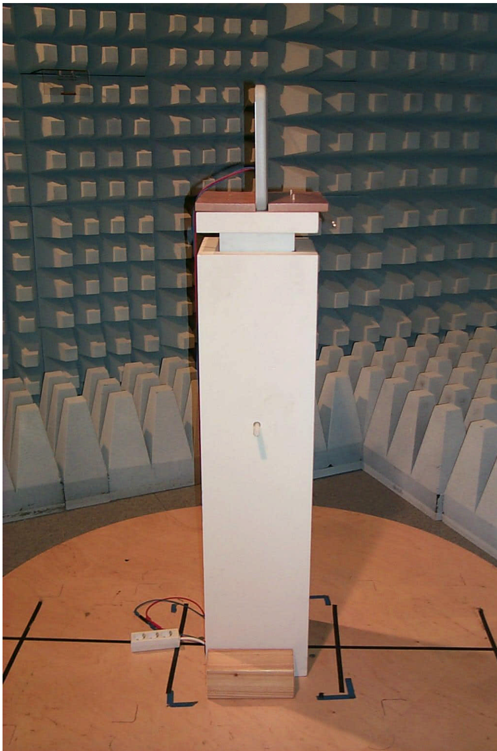
30052emi5.jpg Test set-up preliminary emission measurement (9 kHz to 30 MHz)
