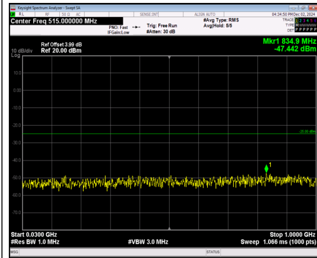
Band66-1.4MHz-QPSK-131979-1RB#0-Range1:30~1000MHz
