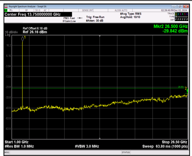
Band38-5MHz-64QAM-37775-1RB#0-Range2:1000~26500MHz
