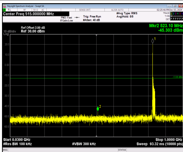
Band26-15MHz-64QAM-26965-1RB#0-Range1:30~1 000MHz
