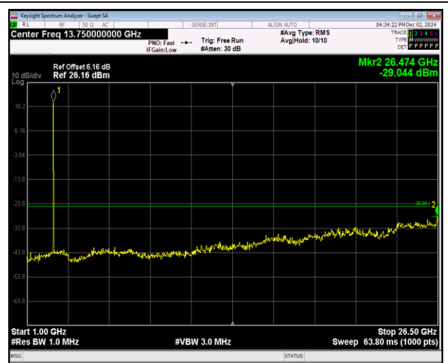
Band41-20MHz-16QAM-40140-1RB#0-Range2:1000~26500MHz
