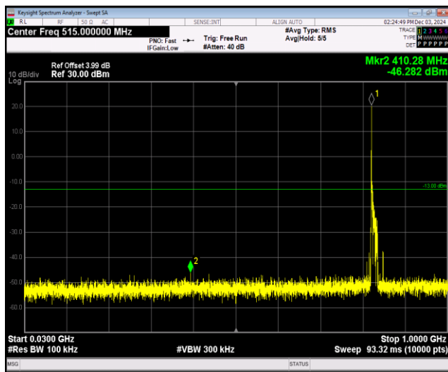
Band26-15MHz-64QAM-26915-1RB#0-Range1:30~1 000MHz
