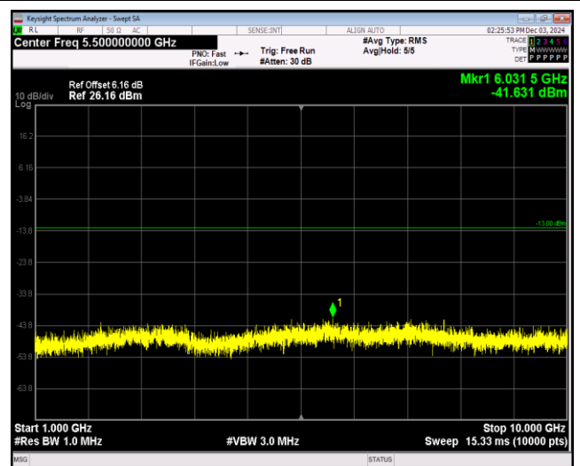
Band26-15MHz-64QAM-26965-1RB#0-Range2:1000 ~10000MHz
