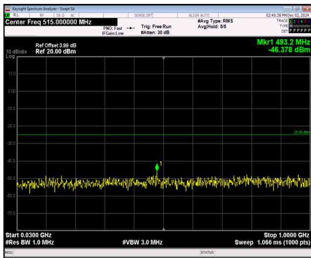
Band38-5MHz-64QAM-38225-1RB#0-Range1:30~1000MHz
