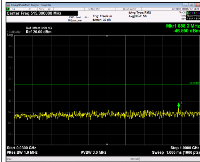
Band38-5MHz-QPSK-38000-1RB#0-Range1:30~100 OMHz
