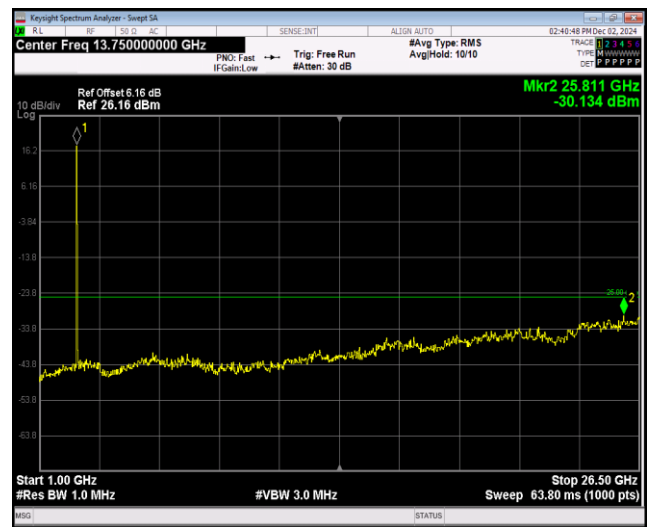
Band38-5MHz-64QAM-38225-1RB#0-Range2:1000~26500MHz
