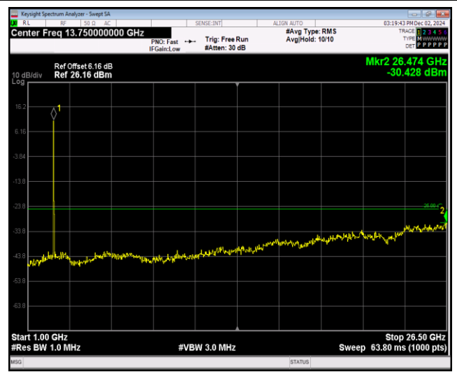
Band38-20MHz-64QAM-38000-1RB#0-Range2:1000~26500MHz
