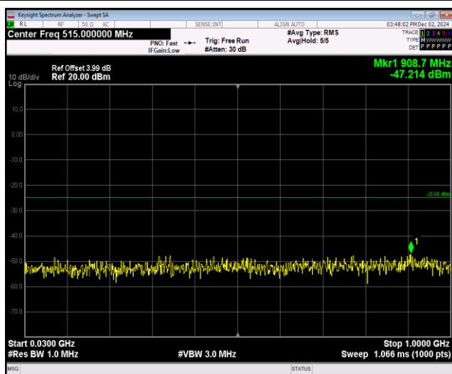
Band41-5MHz-QPSK-40640-1RB#0-Range1:30~1000MHz
