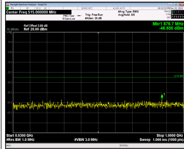
Band41-20MHz-16QAM-40640-1RB#0-Range1:30~1000MHz
