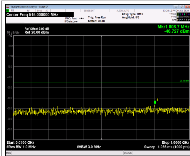
Band38-20MHz-64QAM-37850-1RB#0-Range1:30~1000MHz
