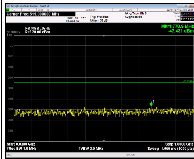
Band38-5MHz-QPSK-38000-1RB#0-Range1:30~100 OMHz
