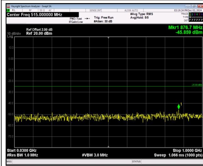
Band38-20MHz-64QAM-38000-1RB#0-Range1:30~1000MHz
