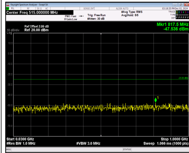
Band38-20MHz-64QAM-38000-1RB#0-Range1:30~1000MHz
