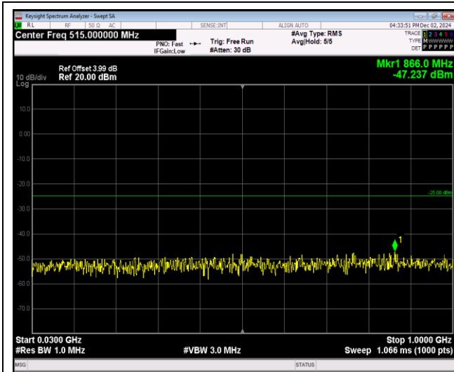
Band41-20MHz-64QAM-41140-1RB#0-Range1:30~1000MHz
