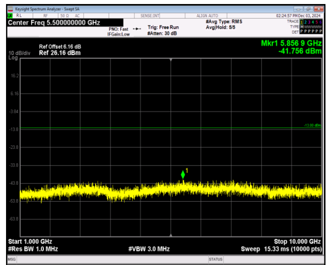
Band26-15MHz-64QAM-26915-1RB#0-Range2:1000 ~10000MHz
