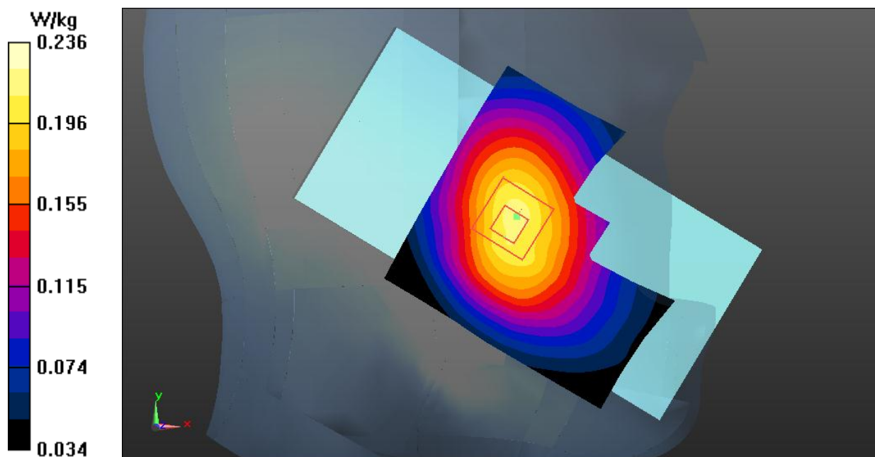
Fig.1 GSM 850 Head
