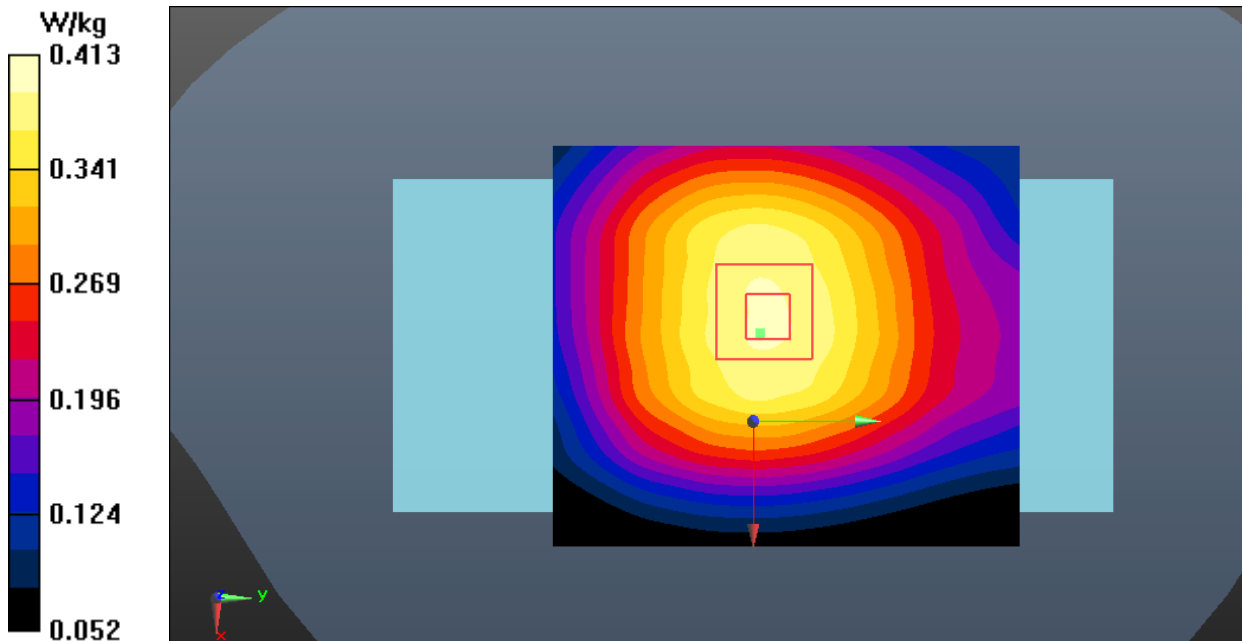
Fig.2 GSM 850 Body
