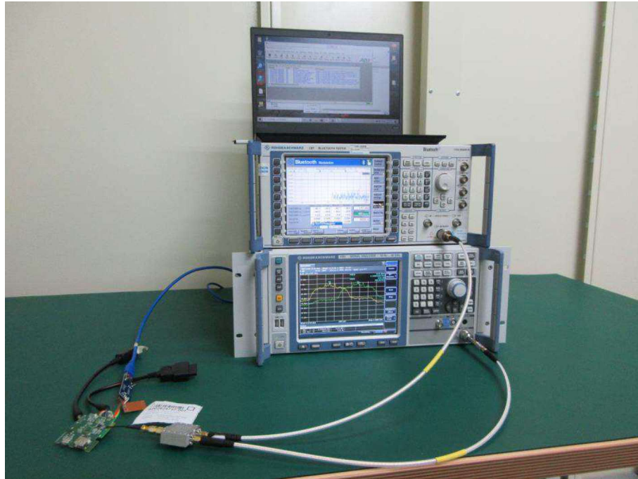
Photograph 7: Set-up for Conducted testing (View 1)
